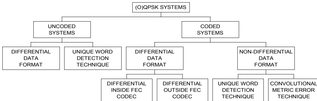
Figure 2.4.11-1: List of Phase-Ambiguity Resolution Techniques
