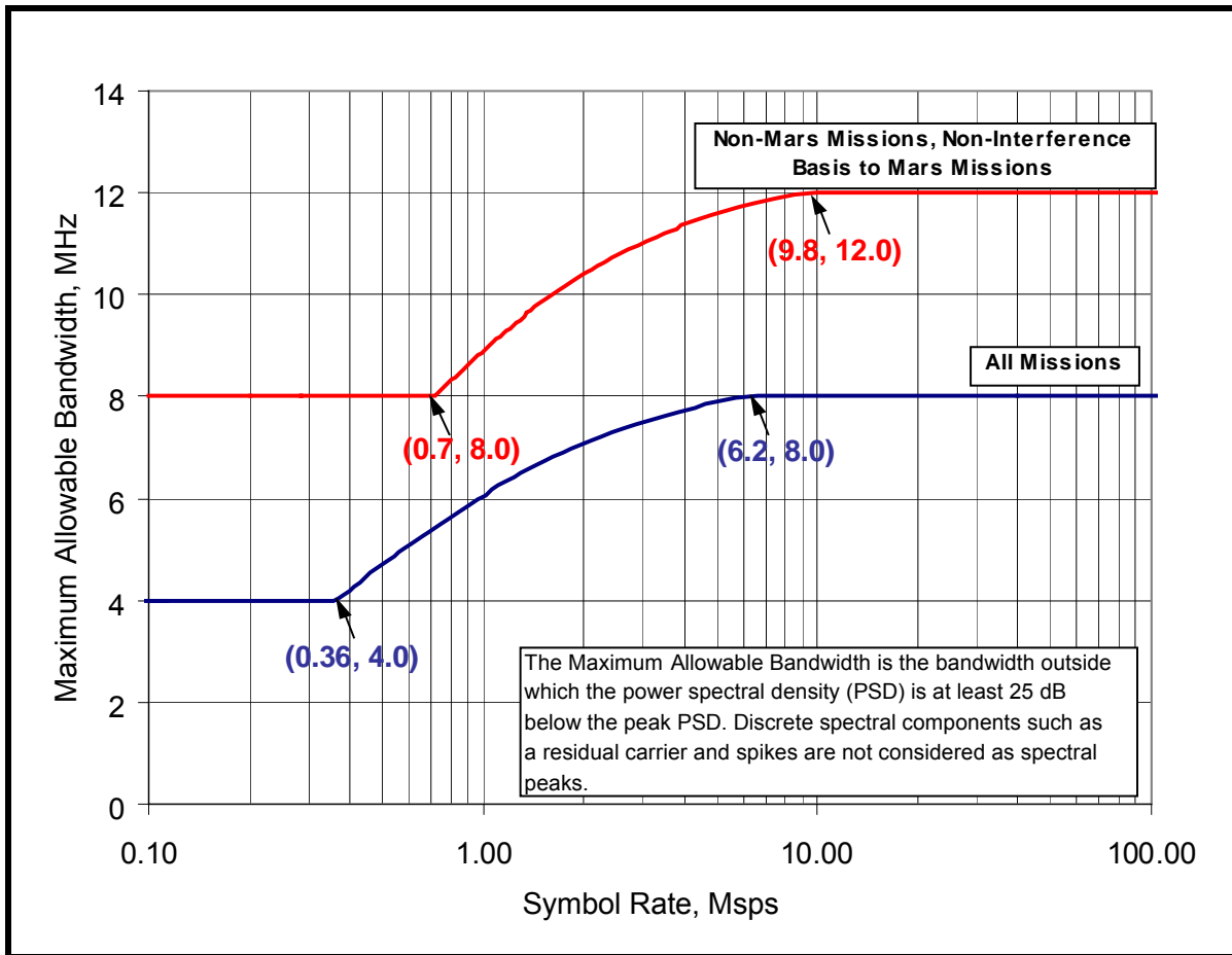
Figure 3.1.2B-1: Maximum Allowable Bandwidth (B25) vs. Symbol Rate (Rs) (in the Transition Regions, B_{25} in MHz= k \cdot R_s / (0.41 + R_s) where k=8.53 and 12.5 for All-Missions and Non-Mars Missions, Respectively)
