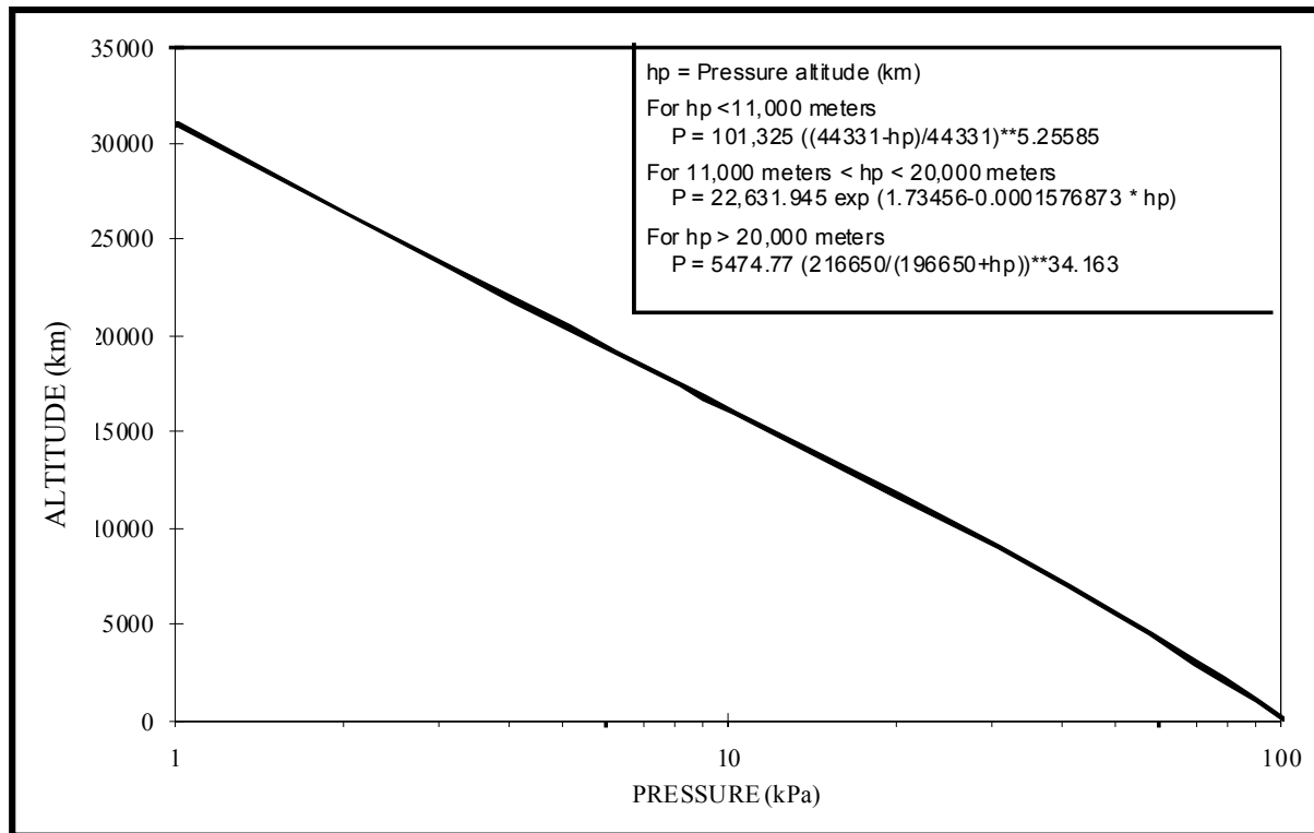
Figure C-1. Altitude versus pressure conversion plot.
