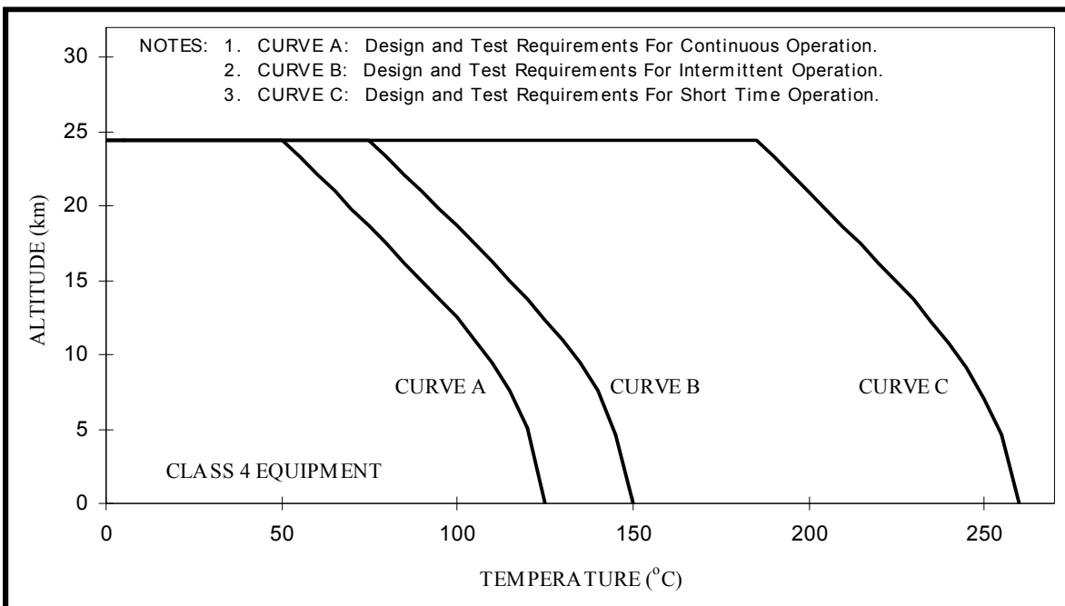
Figure B-4. Operational planning requirements for Class 4 aerospace equipment, temperature versus altitude.
