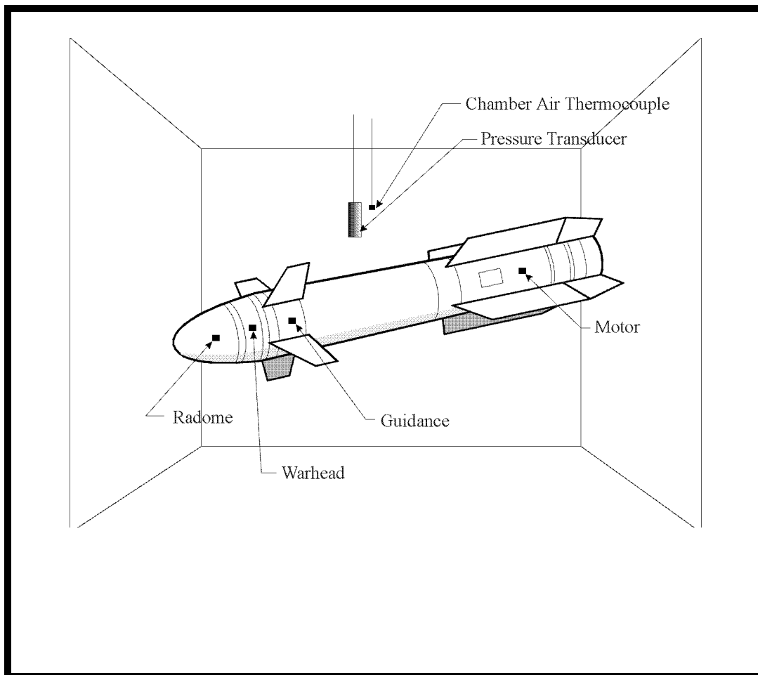
Figure A-1. Transducer locations (pressure thermocouple) on test item.
