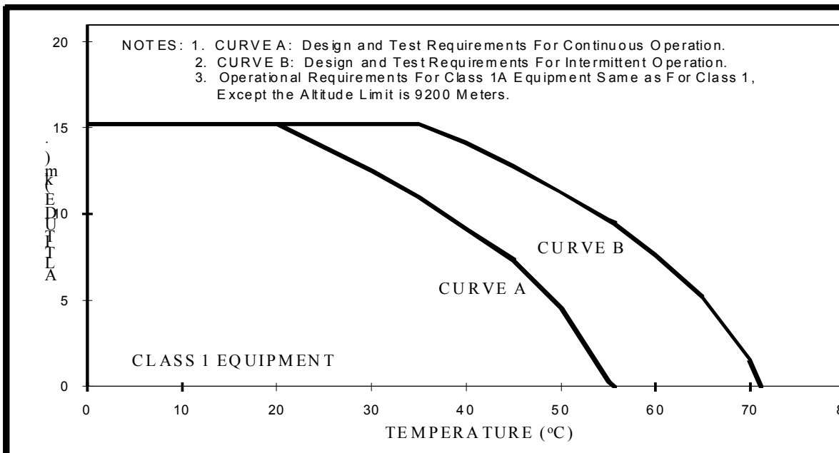
Figure B-1. Operational planning requirements for Class 1 aerospace equipment, temperature versus altitude.
