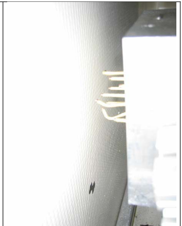
Figure 3b. Piezopins following test. Note pin deformation caused by wall movement.
