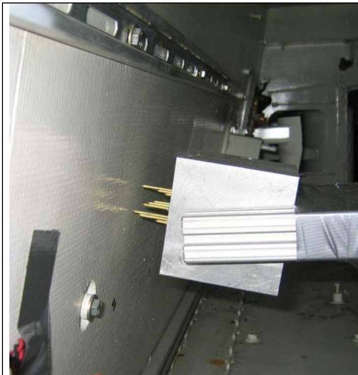
Figure 3a. Multiple Piezopins arrayed in a Nylon Block for measuring different levels of deformation.
