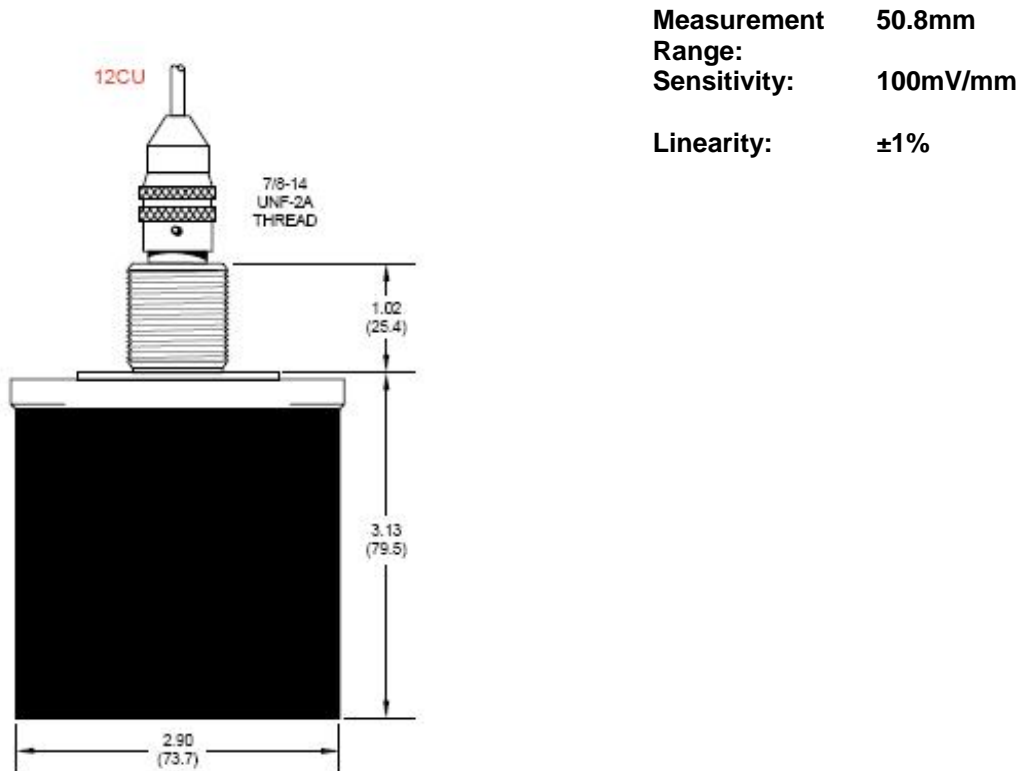
Figure 11. Kaman Eddy Current Sensor 12CU.
