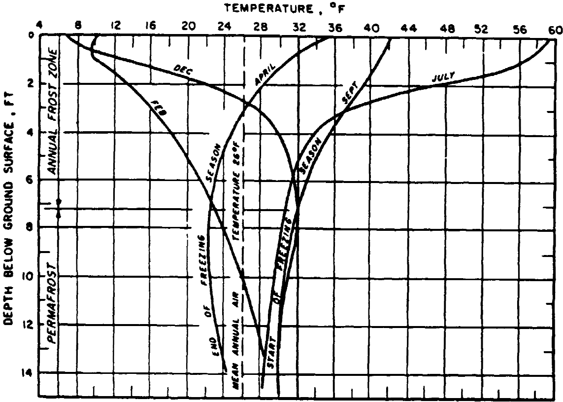
Figure 4-1. Typical ground temperatures, Fairbanks, Alaska.
