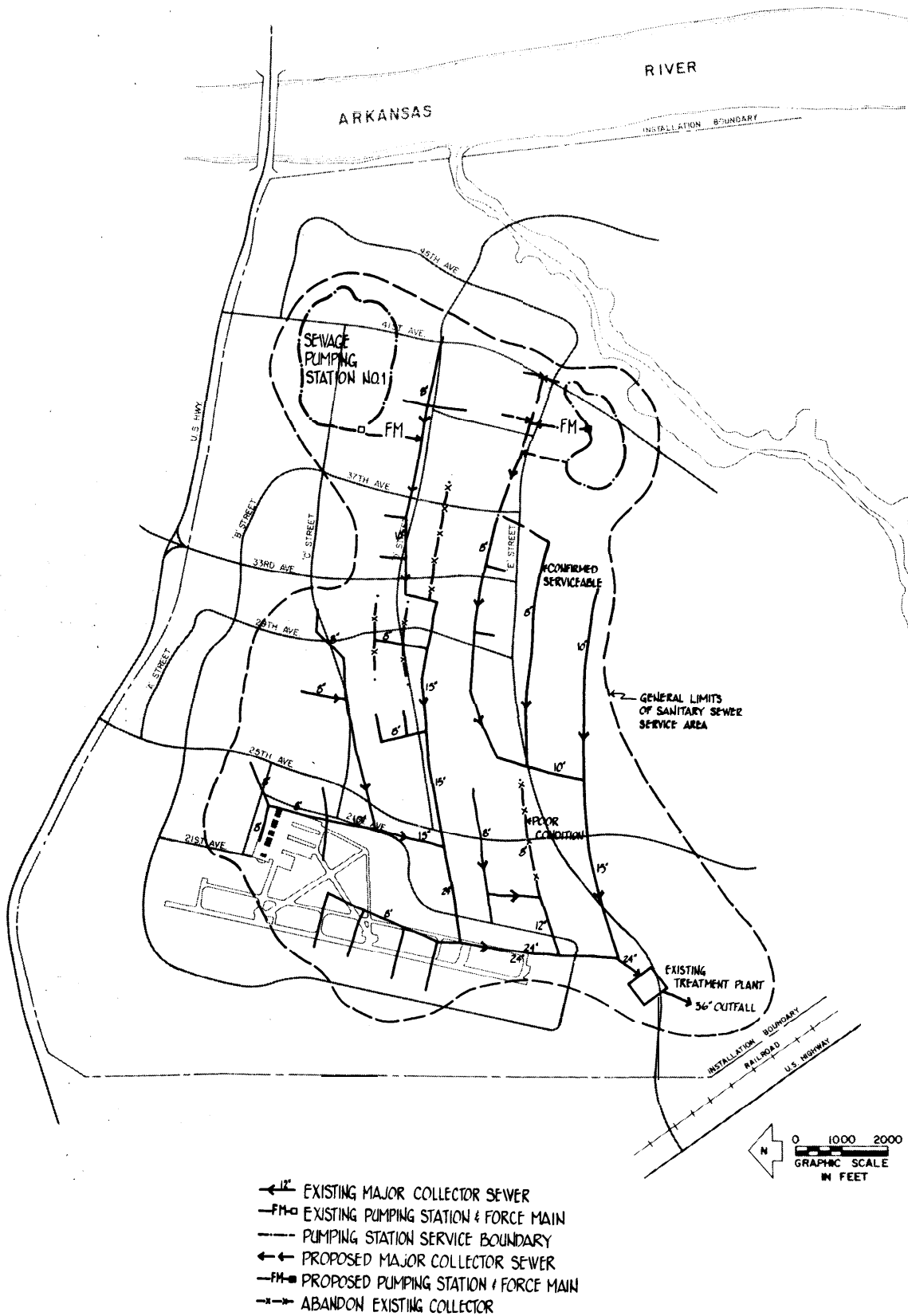
Figure 4-3. Sanitary sewer service plan.
