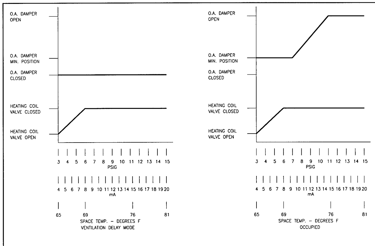
Figure 27. Typical sequencing schedule.
