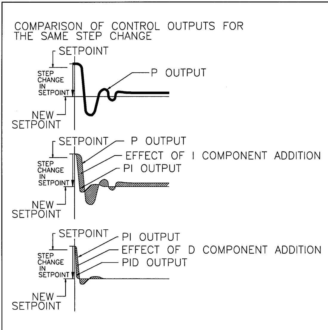
Figure 13. Proportional-integral-derivative control.
