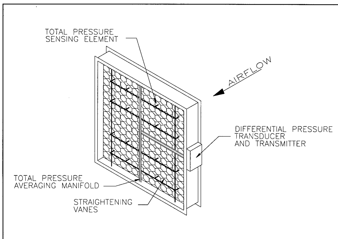
Figure 51. Typical pitot tube airflow measurement station.
