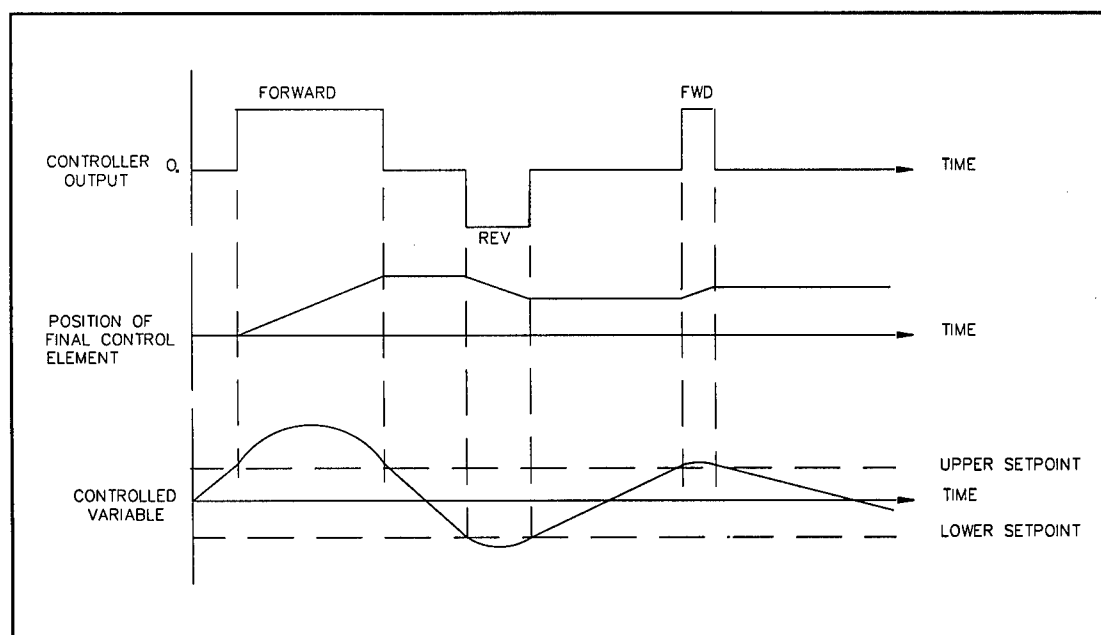
Figure 7. Floating control.
