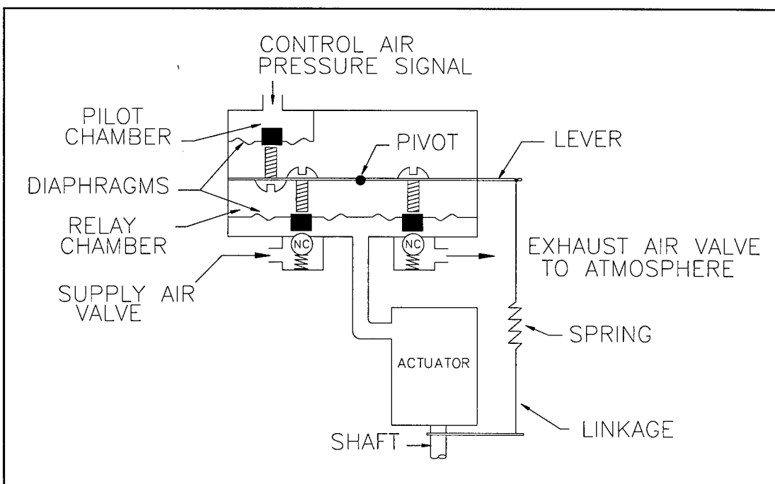
Figure 52. Positive positioner schematic.
