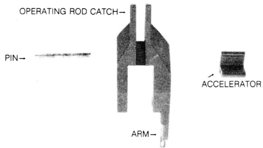
OPERATING ROD CATCH ASSEMBLY DISASSEMBLED
