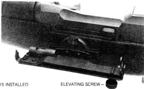
POSITIONING SIGHT ON MOUNTING PLATE.
