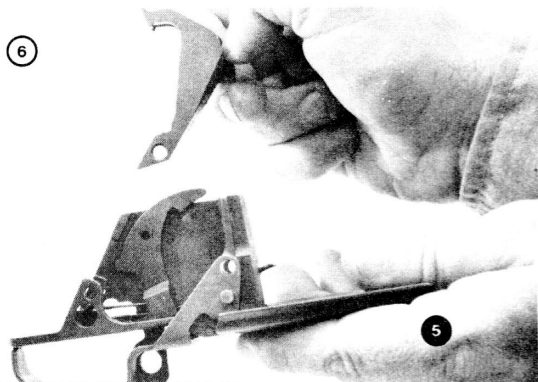
DISASSEMBLE/ASSEMBLE HAMMER.
