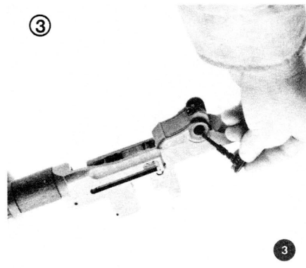
DISASSEMBLE/ASSEMBLE ELEVATING PINION.
