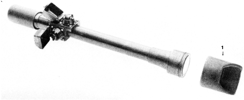
Figure 37. Telescope, M 84.
