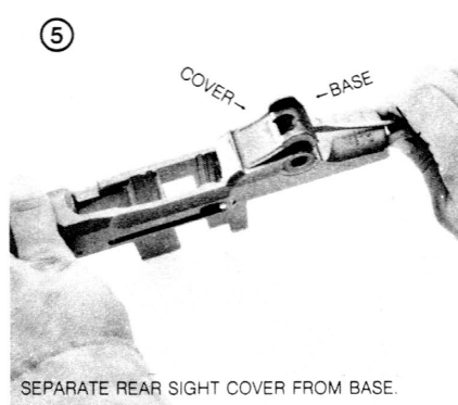
Figure 30. Disassembly / assembly of rear sight group.
