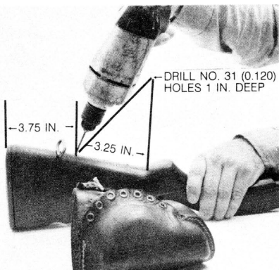
DRILLING HOLES IN STOCK ASSEMBLY FOR INSTALLING WOOD SCREWS.
