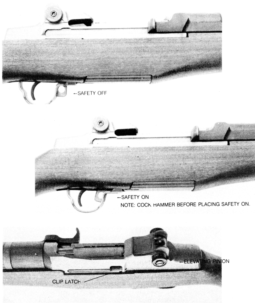
Figure 12. Controls.
