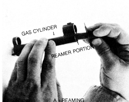
Figure 48. Reaming and gaging front interior of gas cylinder.
