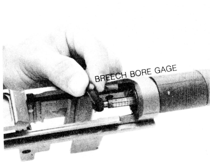
Figure 50. Gaging breech bore.
