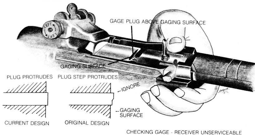
Figure 49. Gaging receiver.
