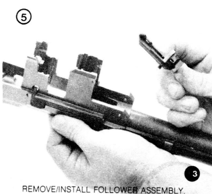
Figure 25. Disassembly / assembly of magazine follower group (1 of 2).
