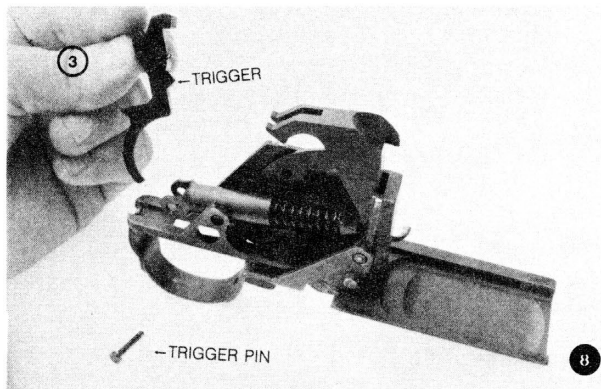
DISASSEMBLE/ASSEMBLE TRIGGER
