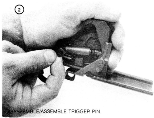
Figure 16. Disassembly / assembly of trigger housing assembly (1 of 4).
