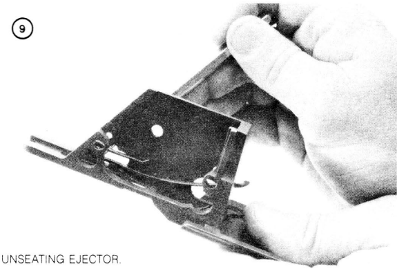
Figure 18. Disassembly / assembly of trigger housing assembly (3 of 4).
