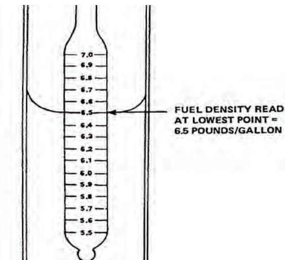
Figure 5-3 - Reading a Hydrometer
