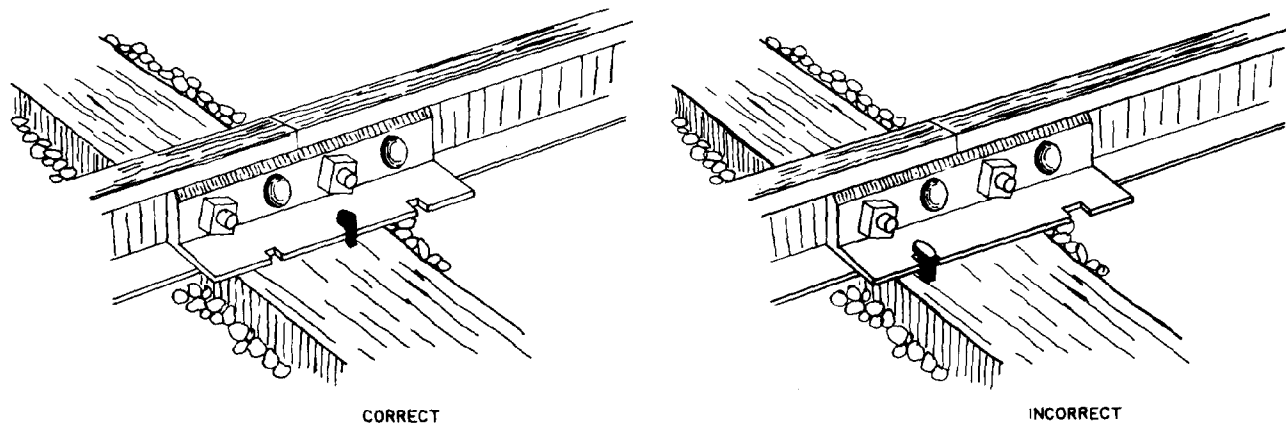
Figure 6-5. Spiking through angle bars.
