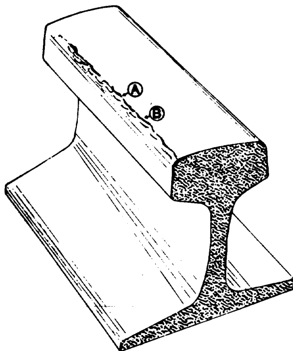
Figure B-11. General appearance of flaking.
