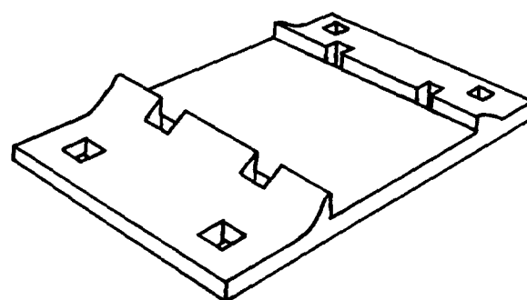
Figure 6-2. Double shoulder tie plate.
