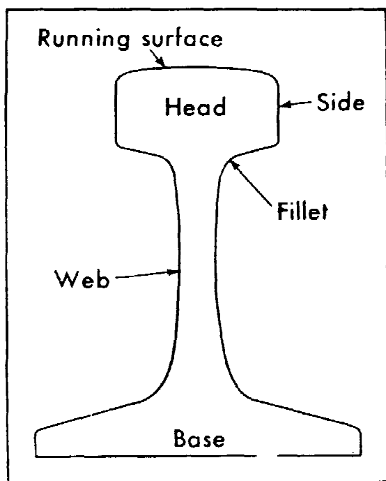
Figure B-1. Rail nomenclature.
