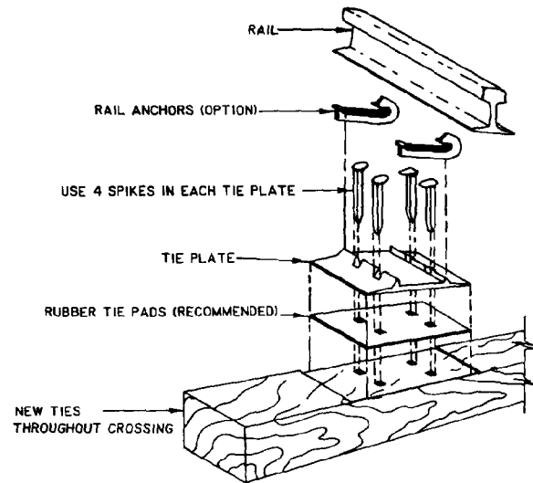
Figure 10-1. Track construction for road crossing.
