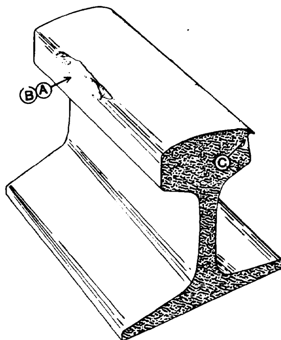
Figure B-19. General appearance of shelling.
