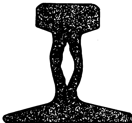
Figure B-17. Cross-sectional view of piped rail.
