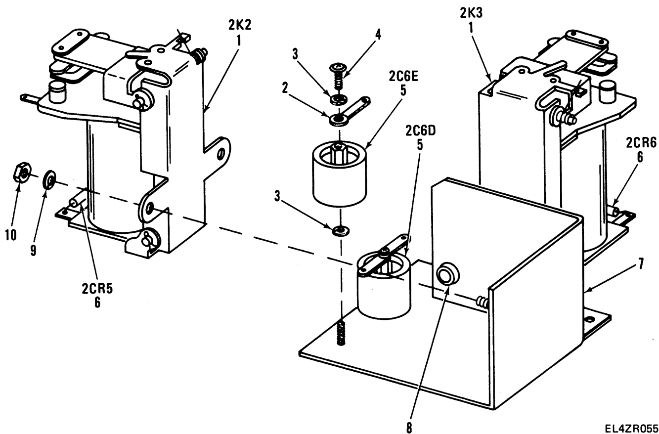
Figure 47. Coupler Unit CU-2229/URC-92-KR-K3 Relay Assembly.
