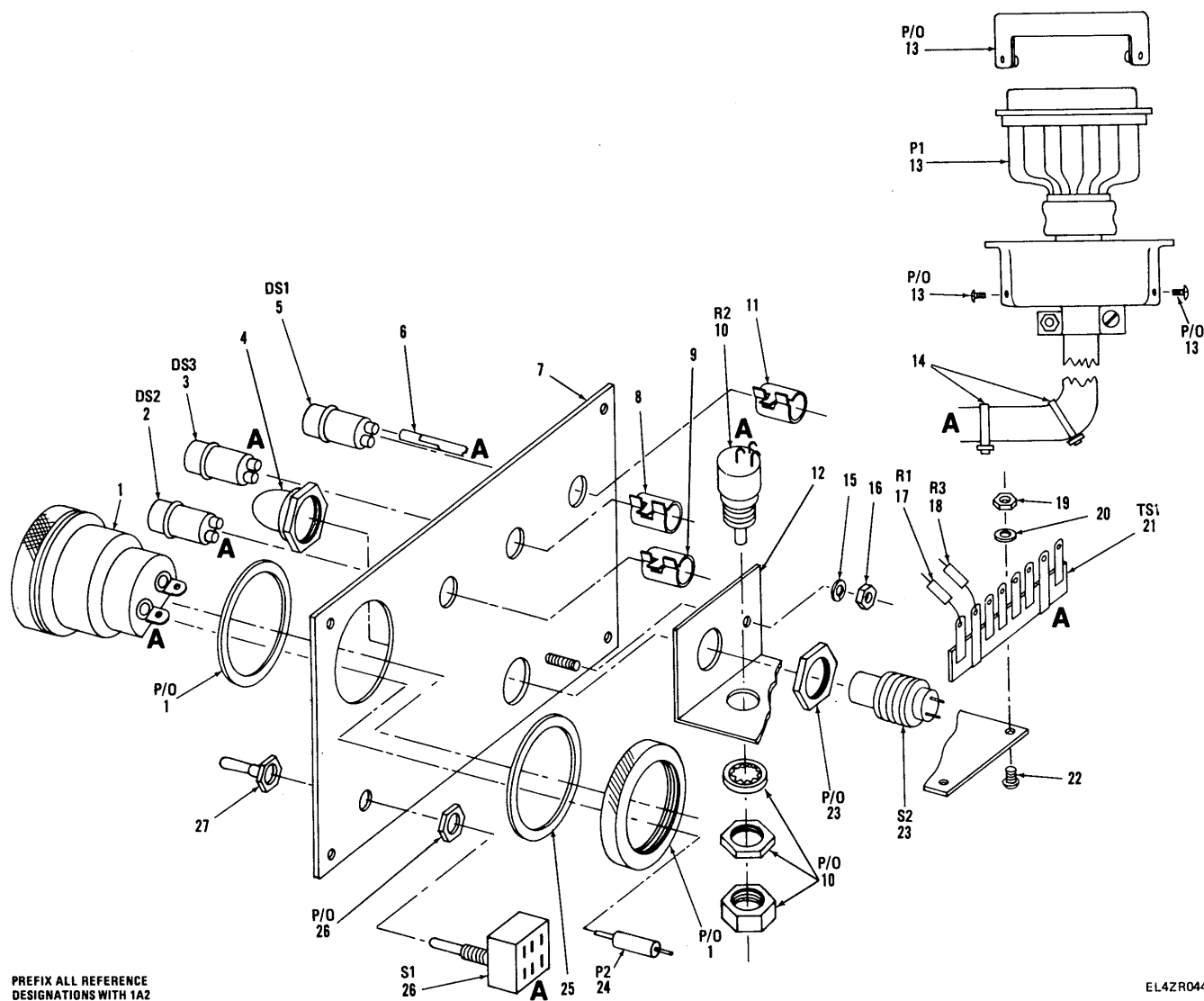
Figure 42. Tuning Control.
