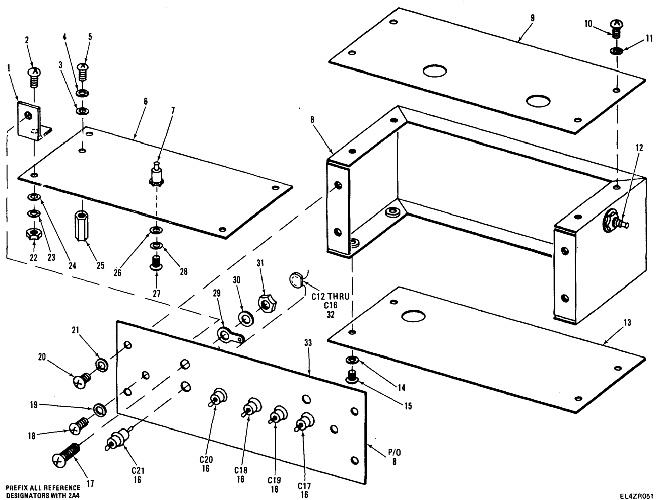
Figure 51. Phase and Amplitude Assembly
