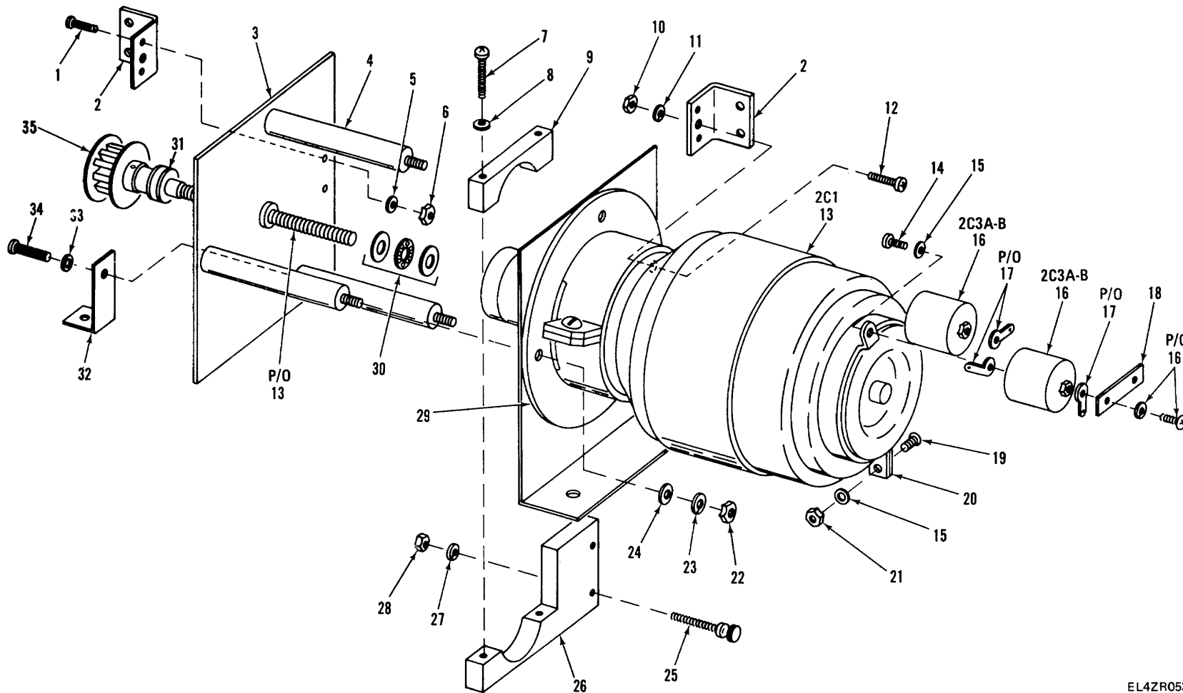
Figure 56. C1 Assembly
