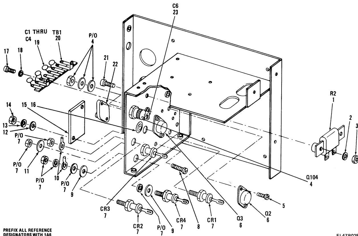
Figure 20. Power Supply Assembly, Chassis, Exploded View.
