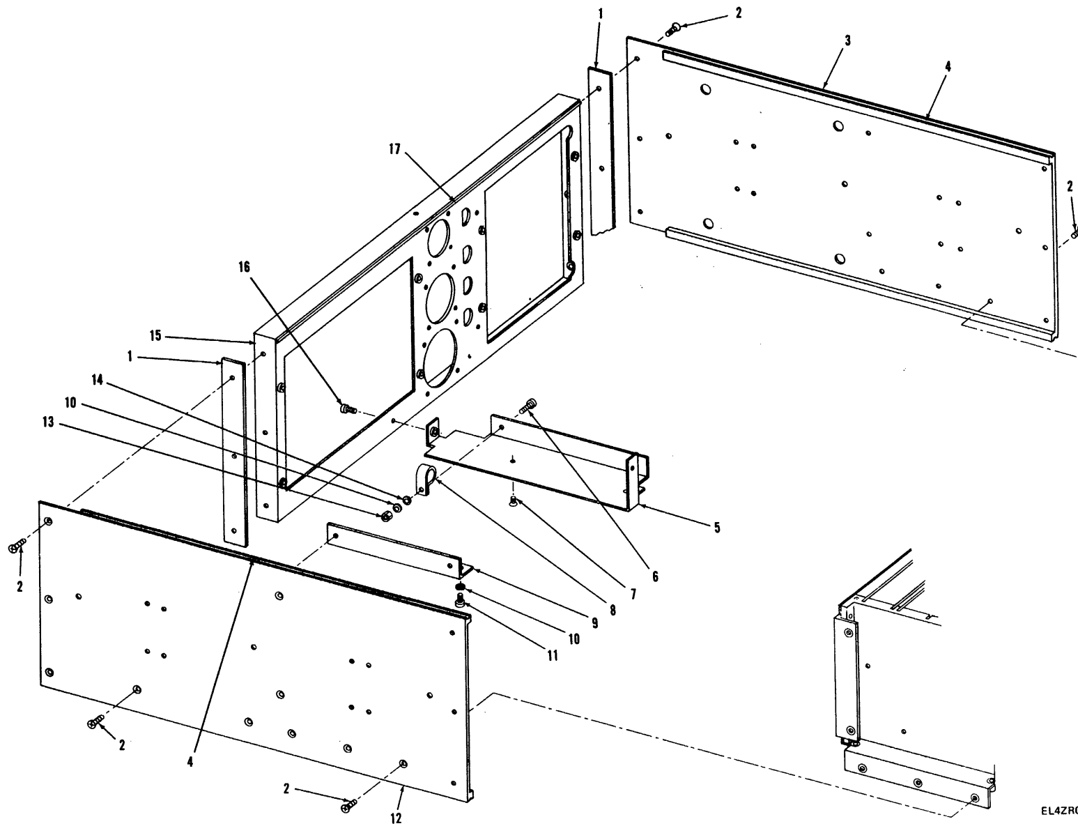
Figure 7. Receiver-Transmitter RT-1277/URC-92-Rear.
