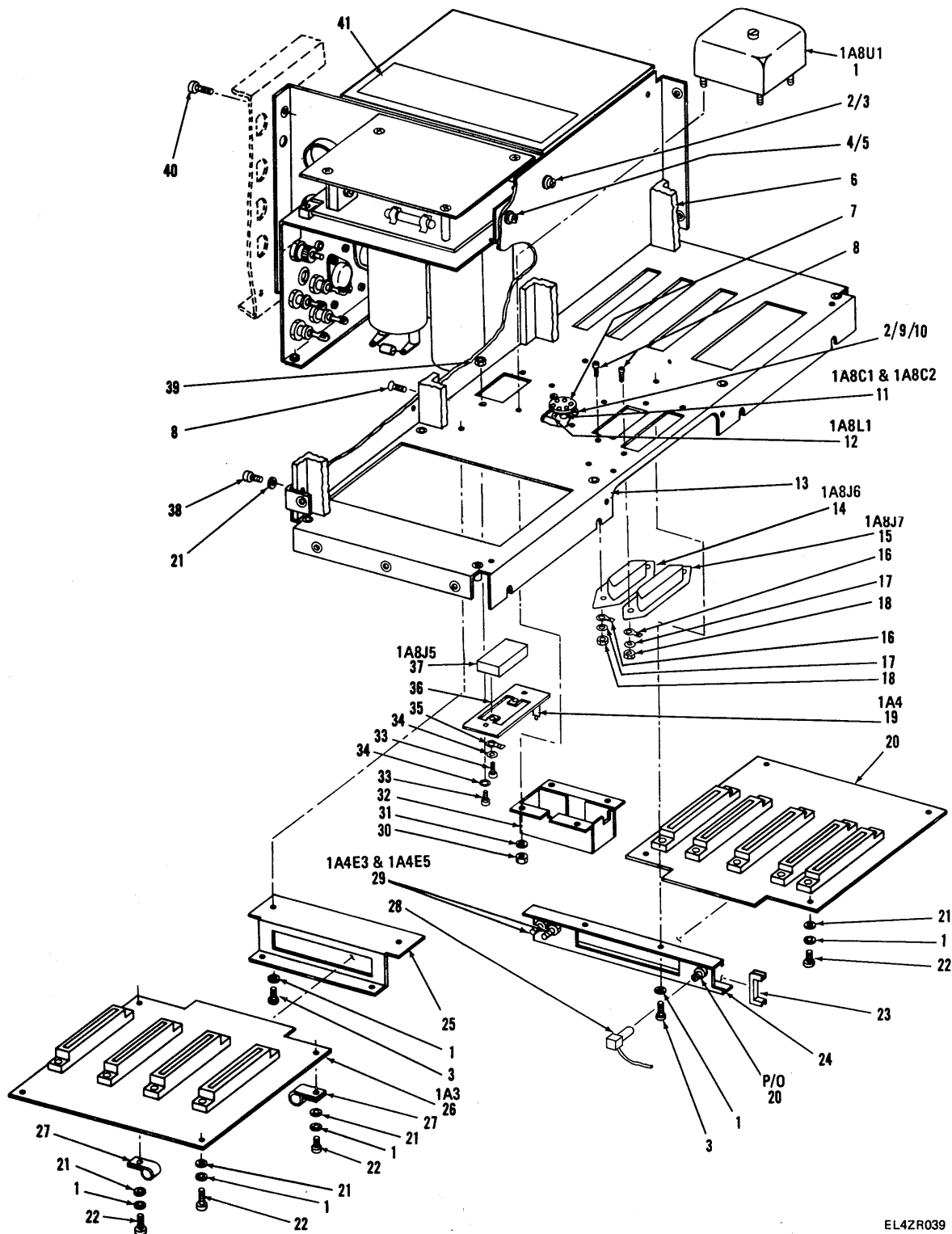
Figure 8. Receiver-Transmitter RT-1277/URC-Center.
