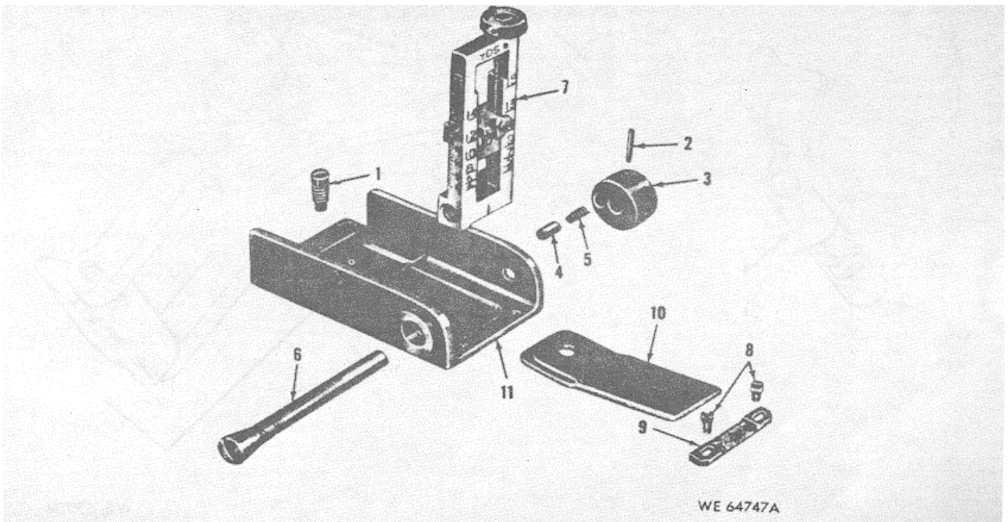
Figure B-8. Rear sight assembly - exploded view.
