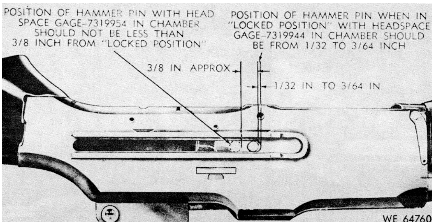
Figure 3-11. Gaging headspace.
