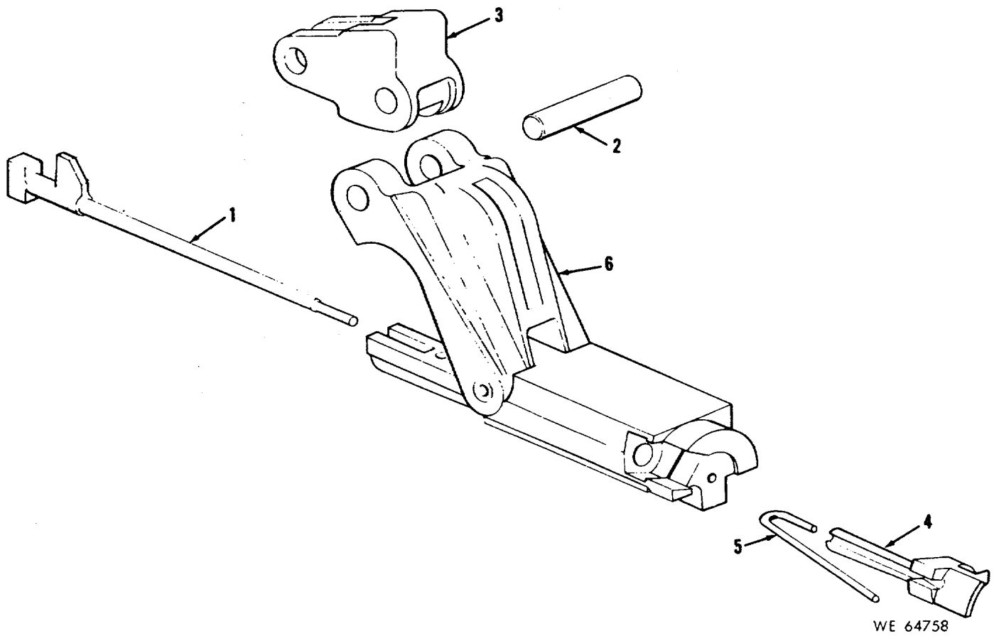
Figure B-3. Bolt Group—exploded group.
