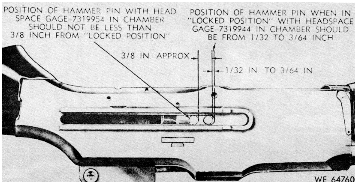
Figure 3-11. Gaging headspace.
