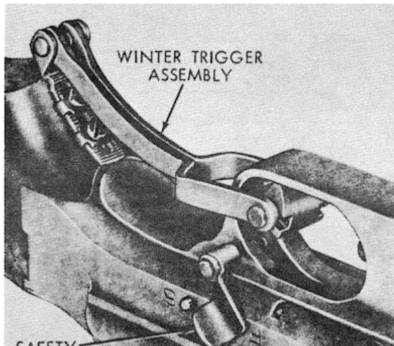
Figure 4-2. Winter trigger kit installed
