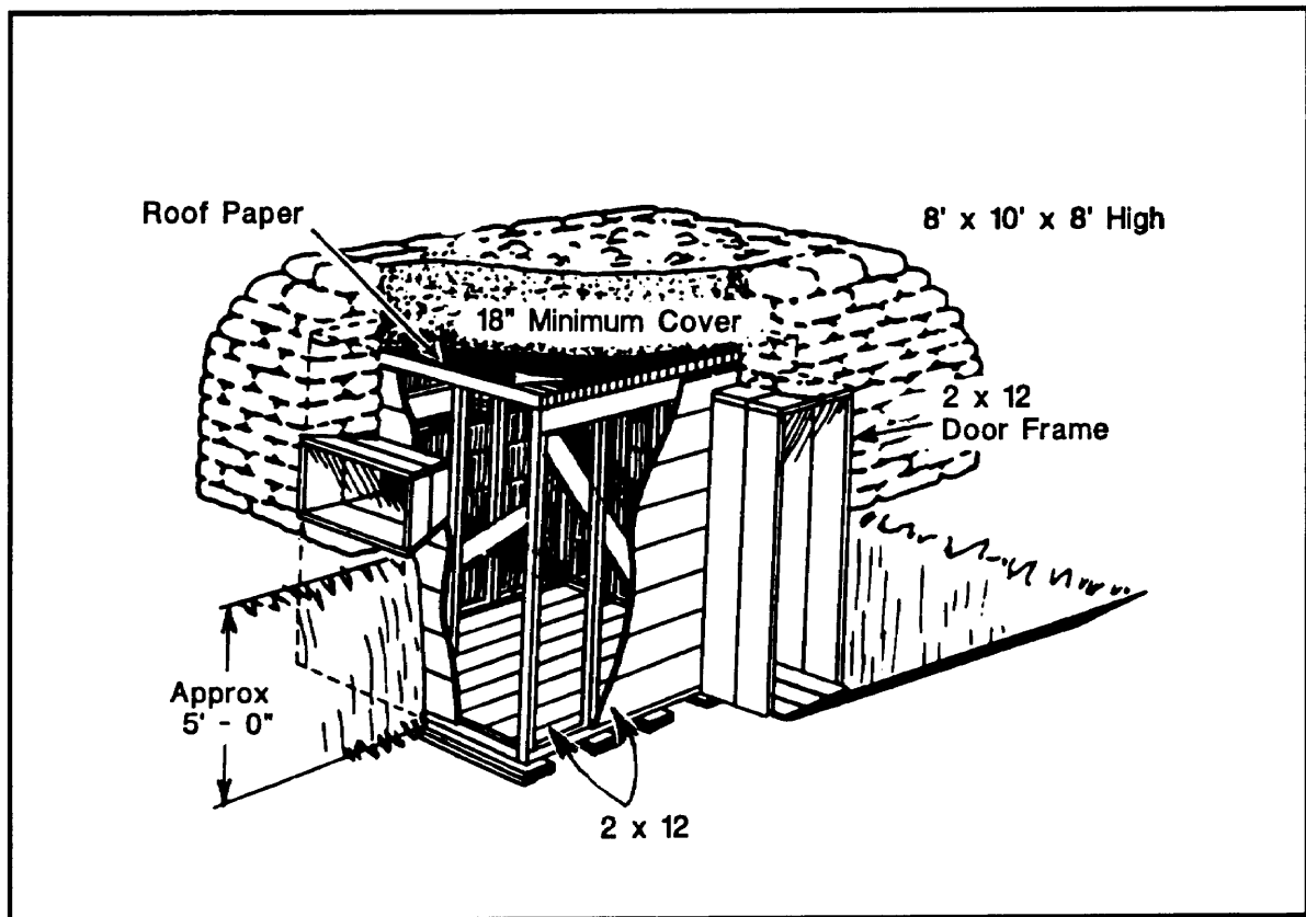
Figure 3-4. Command bunker.
