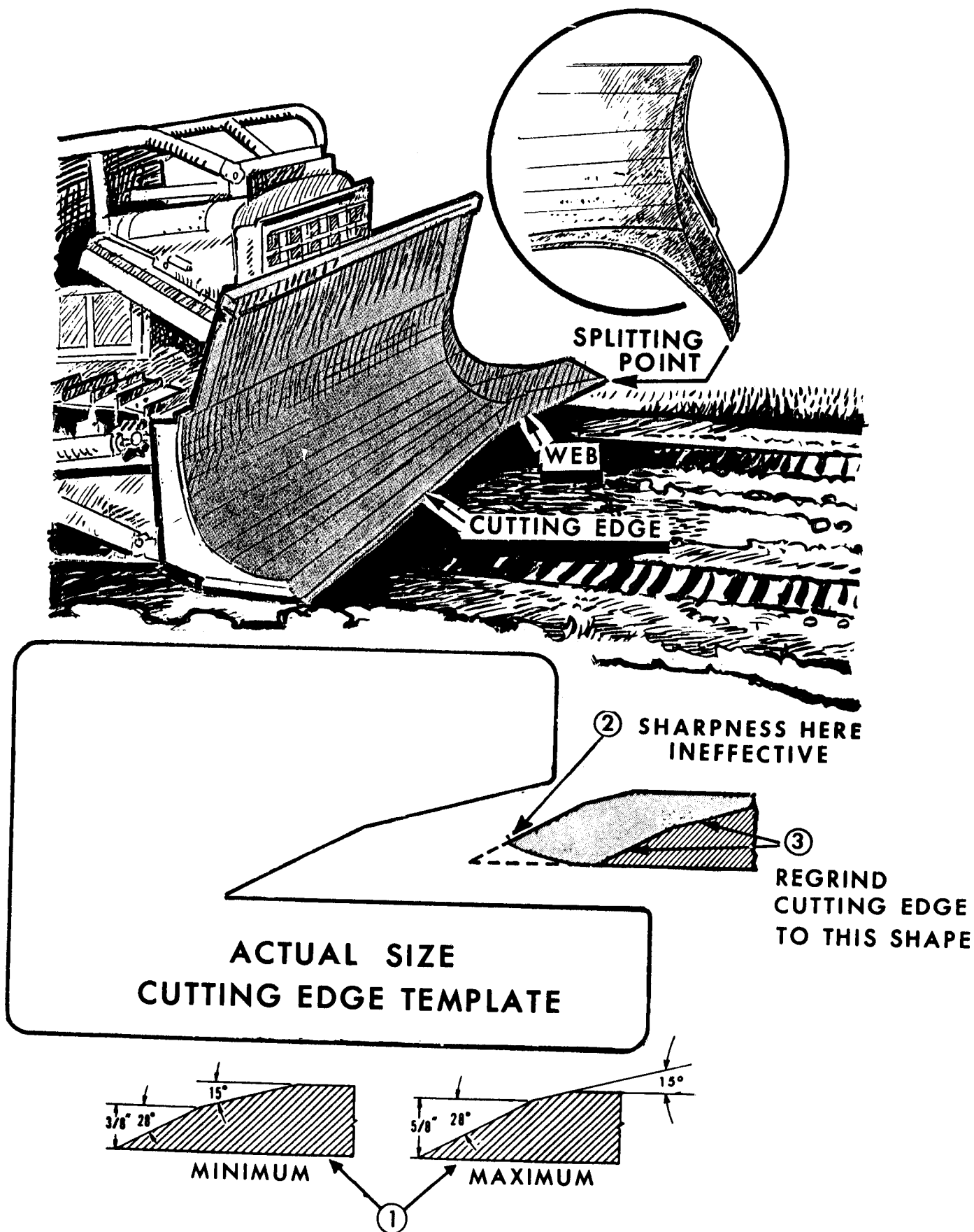
Figure D-1. Cutting edge grinding specifications.
