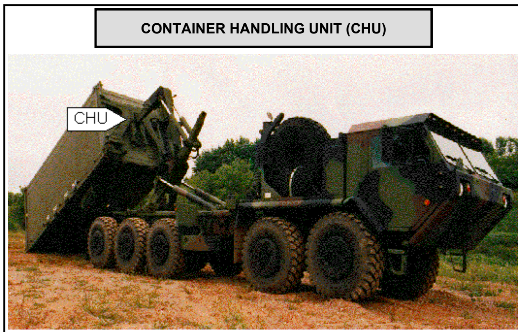
Figure J-7. Container Handling Unit (CHU)
