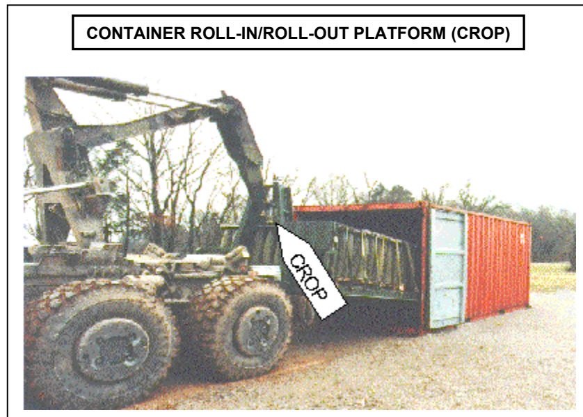
Figure J-17. Container Roll-In/Roll-Out Platform (CROP)
