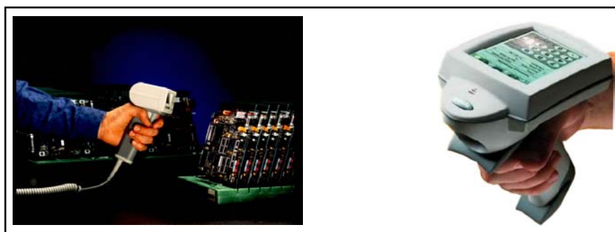
Figure C-12. Bar Coded Data Collection Devices. Tethered reader on the left, portable reader on the right.
