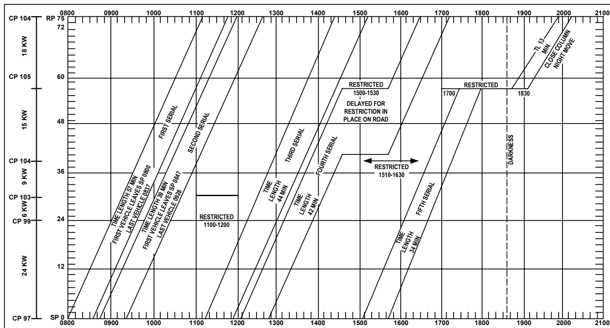
Figure G-8. Road Movement Graph for Five Serials
