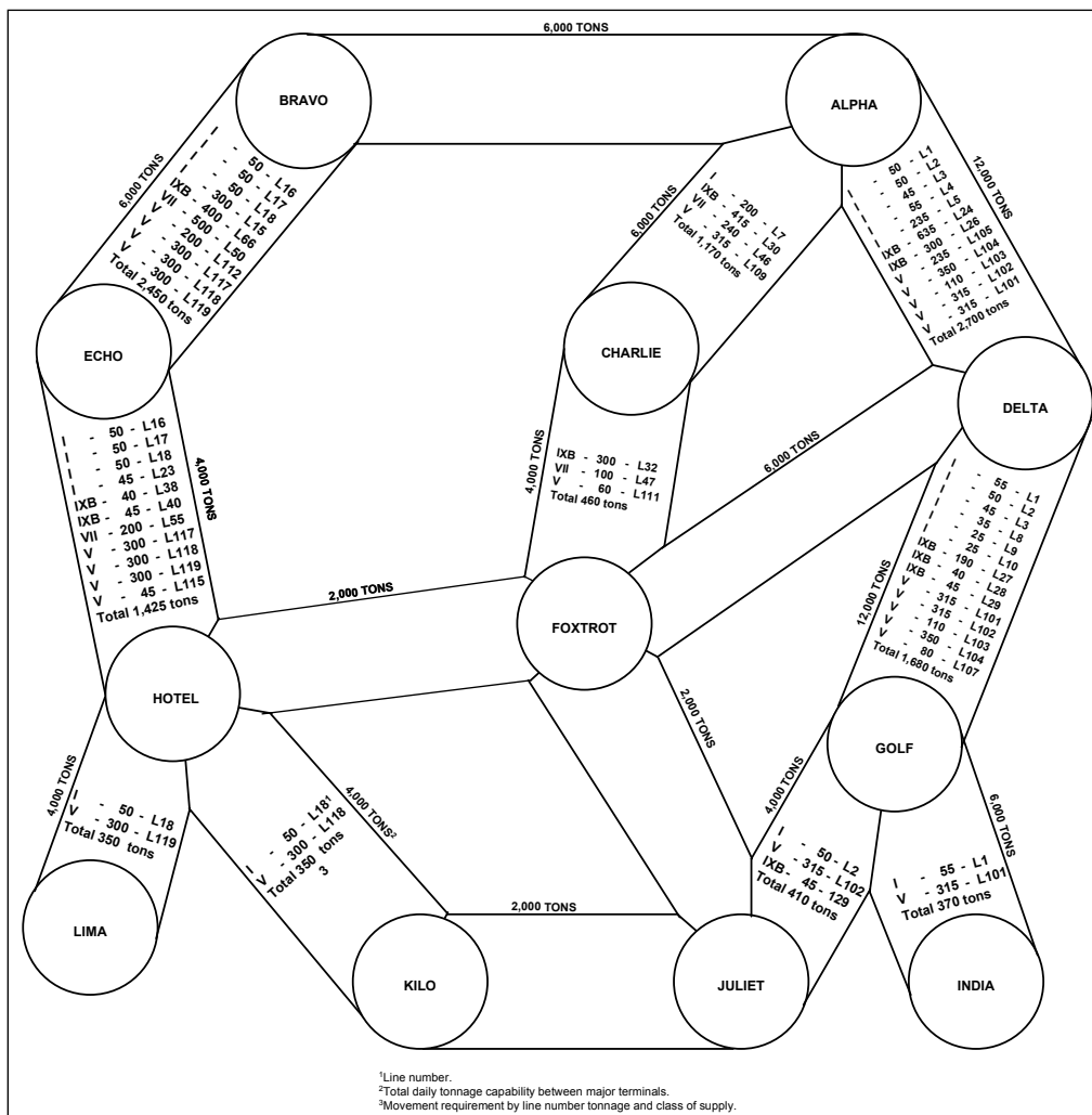
Figure 7-7. Mode Schematic - Rail
