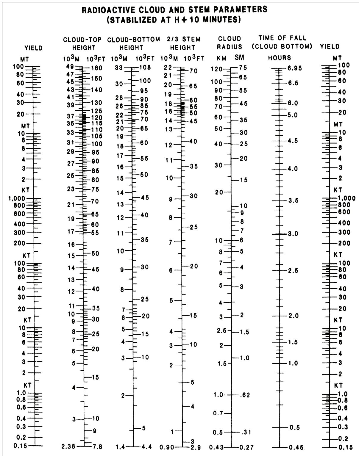
Figure G-21. Stabilized Cloud and Stem Parameters for Detailed Fallout Prediction (Example)
