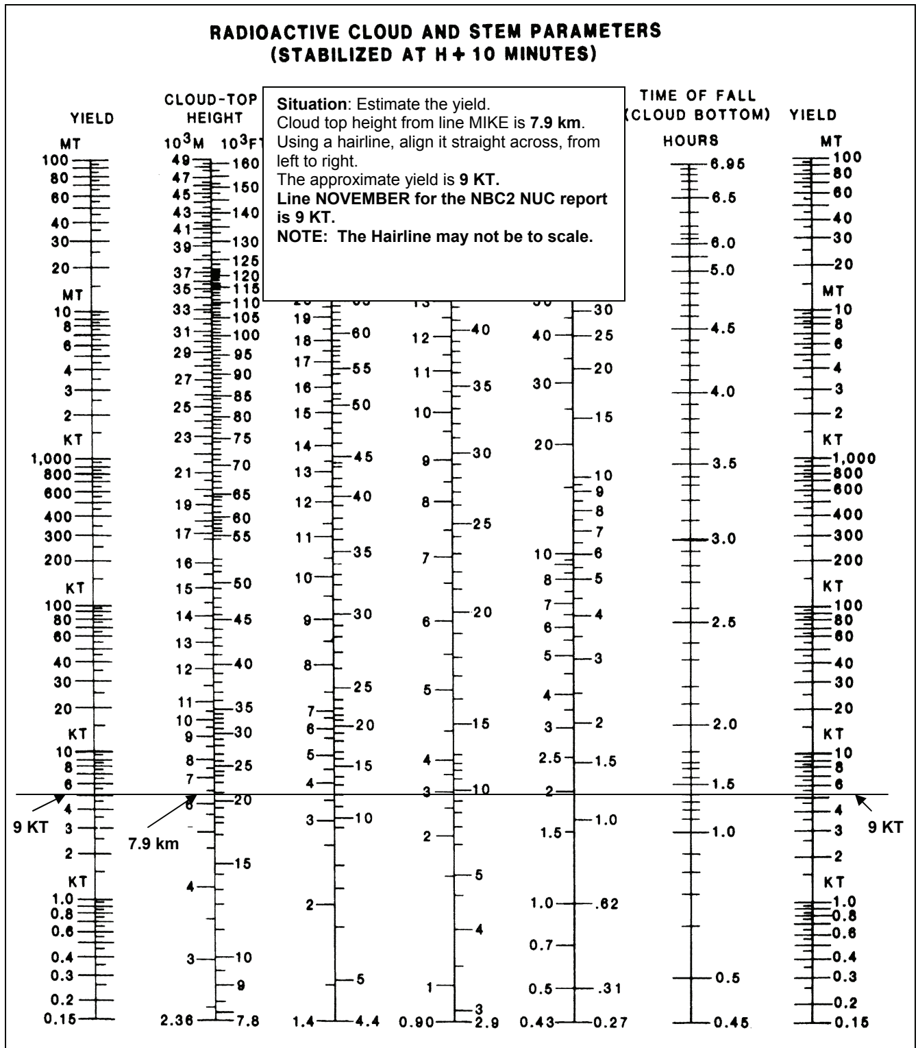
Figure G-9. Stabilized Cloud and Stem Parameters—Cloud Top/Bottom Height (Example)
