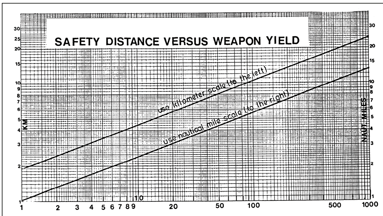
Figure J-5. Safety Distance as a Function of Weapon Yield
