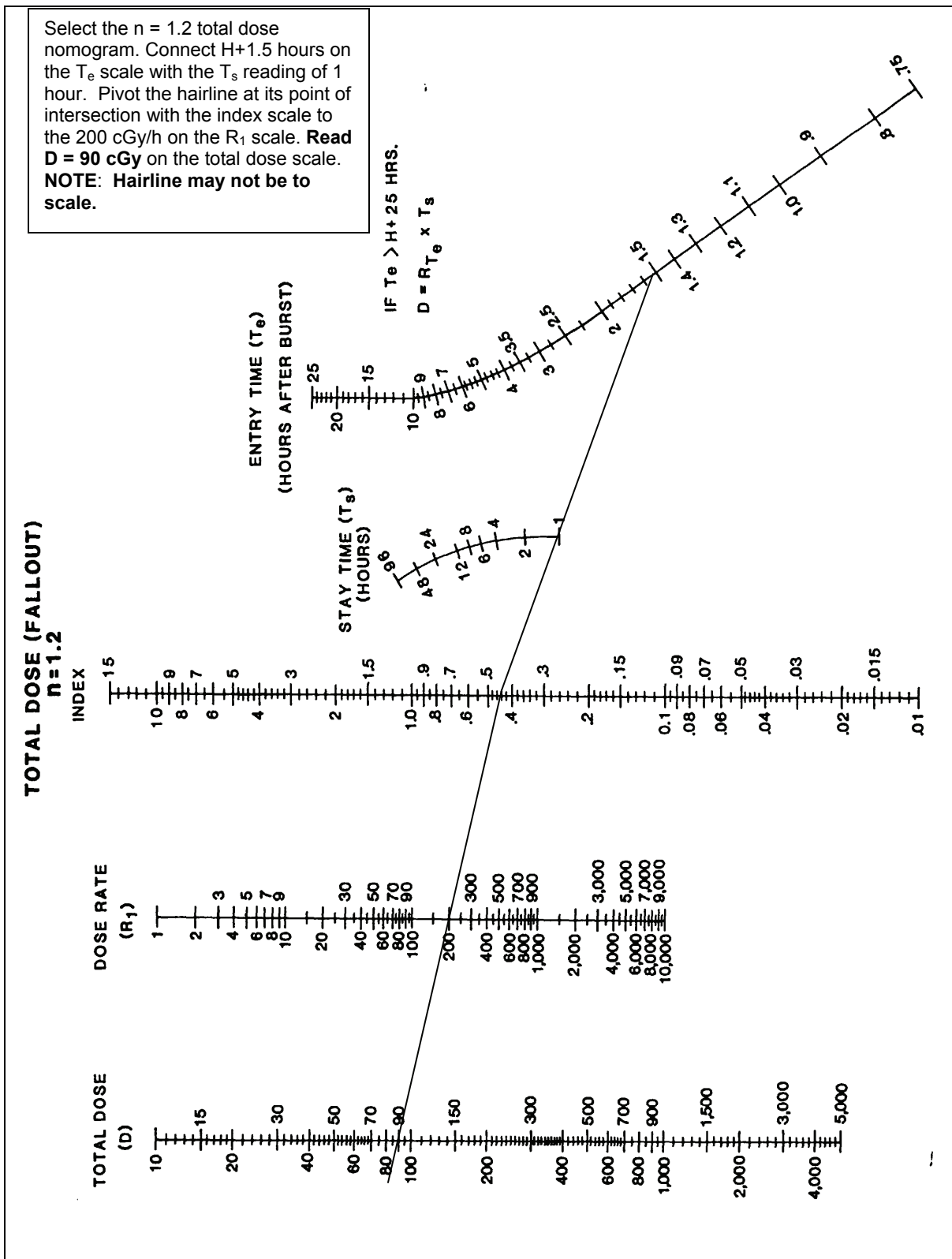
Figure G-36. Total Dose Fallout ( n=1.2 ) (Example)
