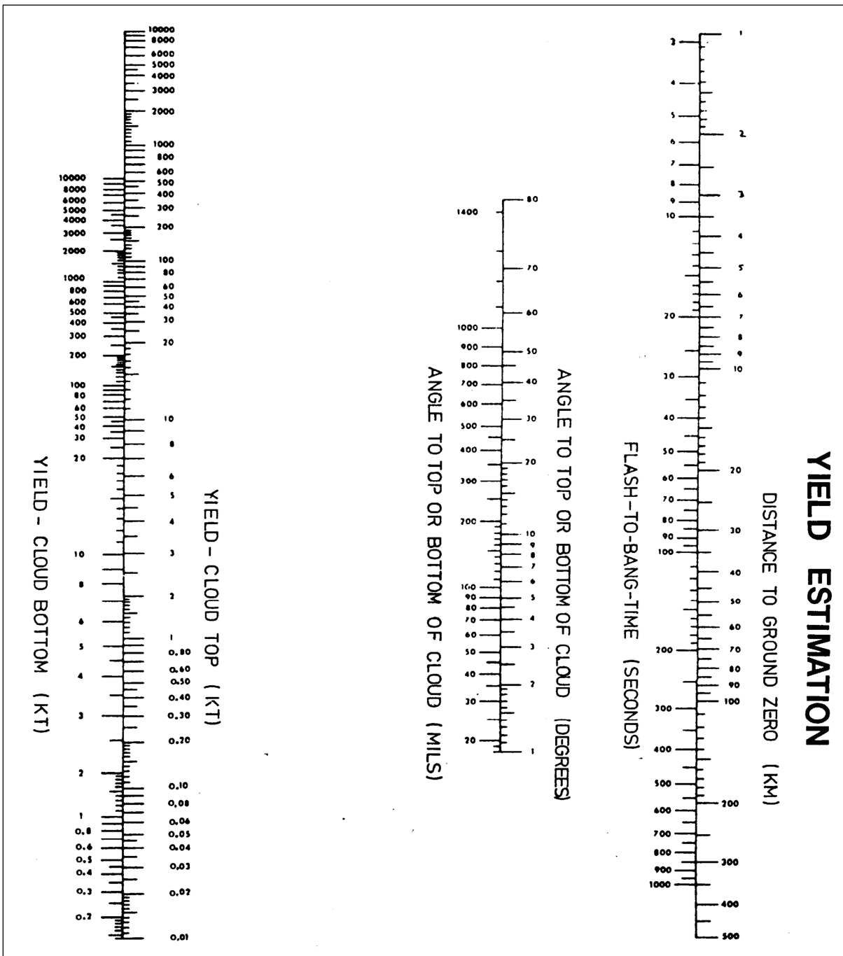
Figure J-7. Yield Estimation, Angle to Top/Bottom of Cloud and Flash-to-Bang Time/Distance to GZ
