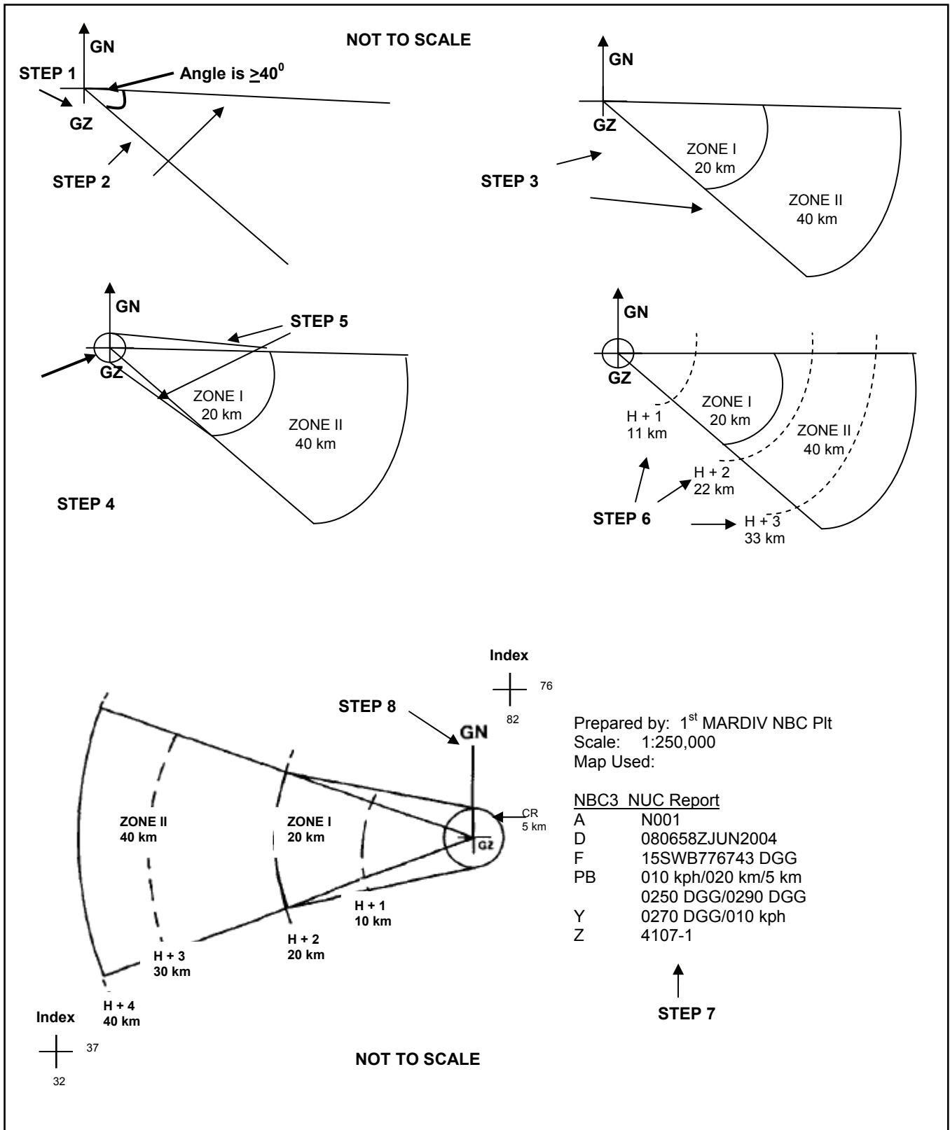
Figure G-27. Detailed Fallout Prediction
