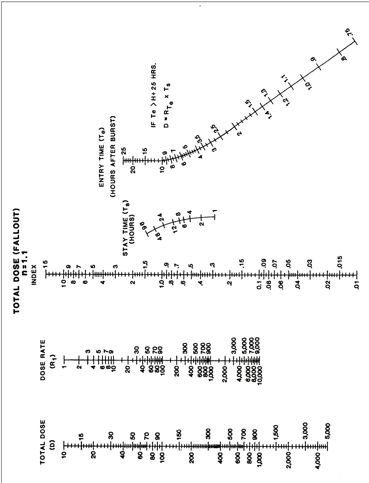
Figure J-37. Total Dose (Fallout) (n=1.1)
