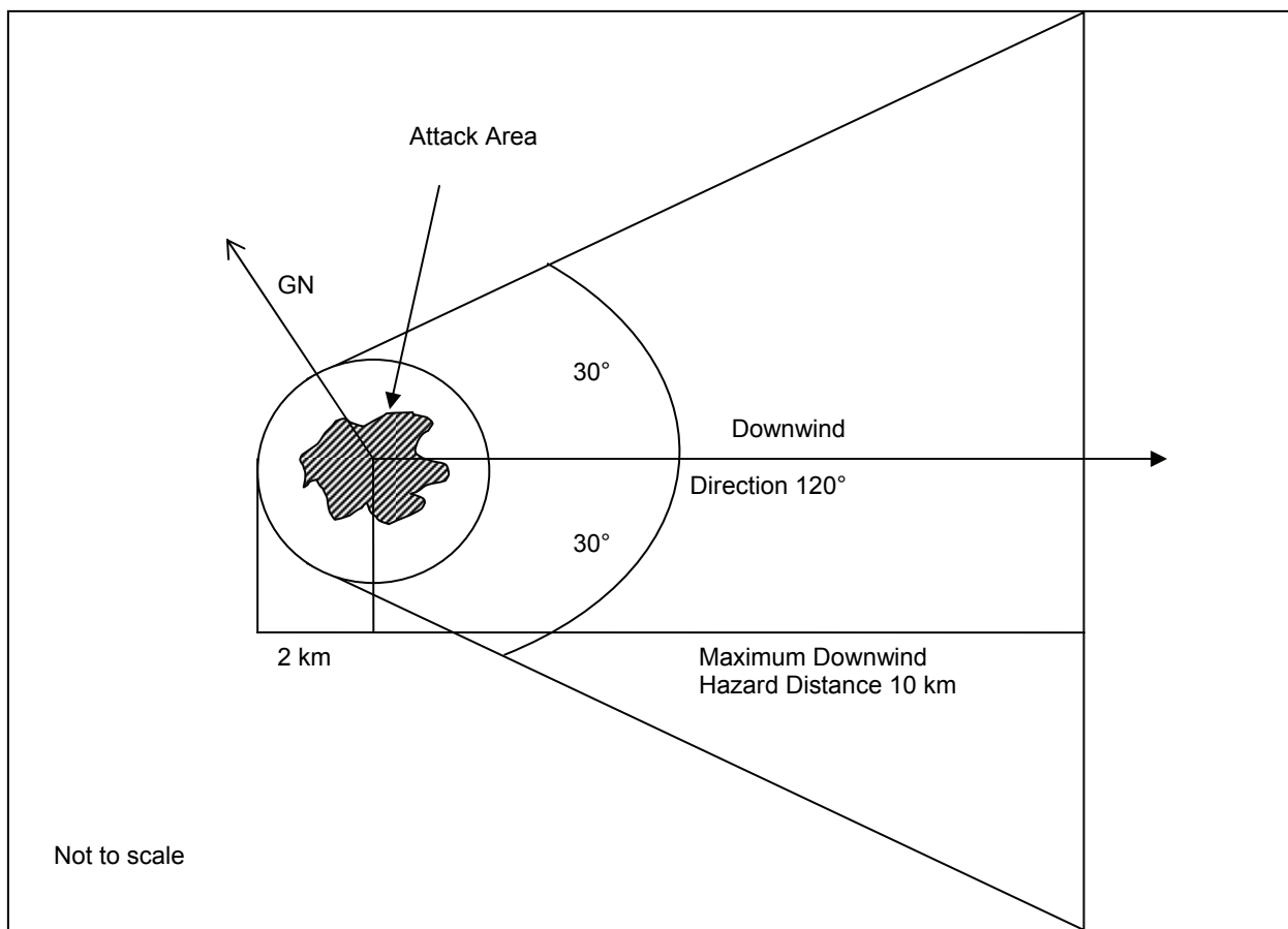
Figure E-10. Hazard Area From Type B Attack, Case 4 (Attack Area Radius >1 km but \leq 2 km, Wind Speed >10 kph)
