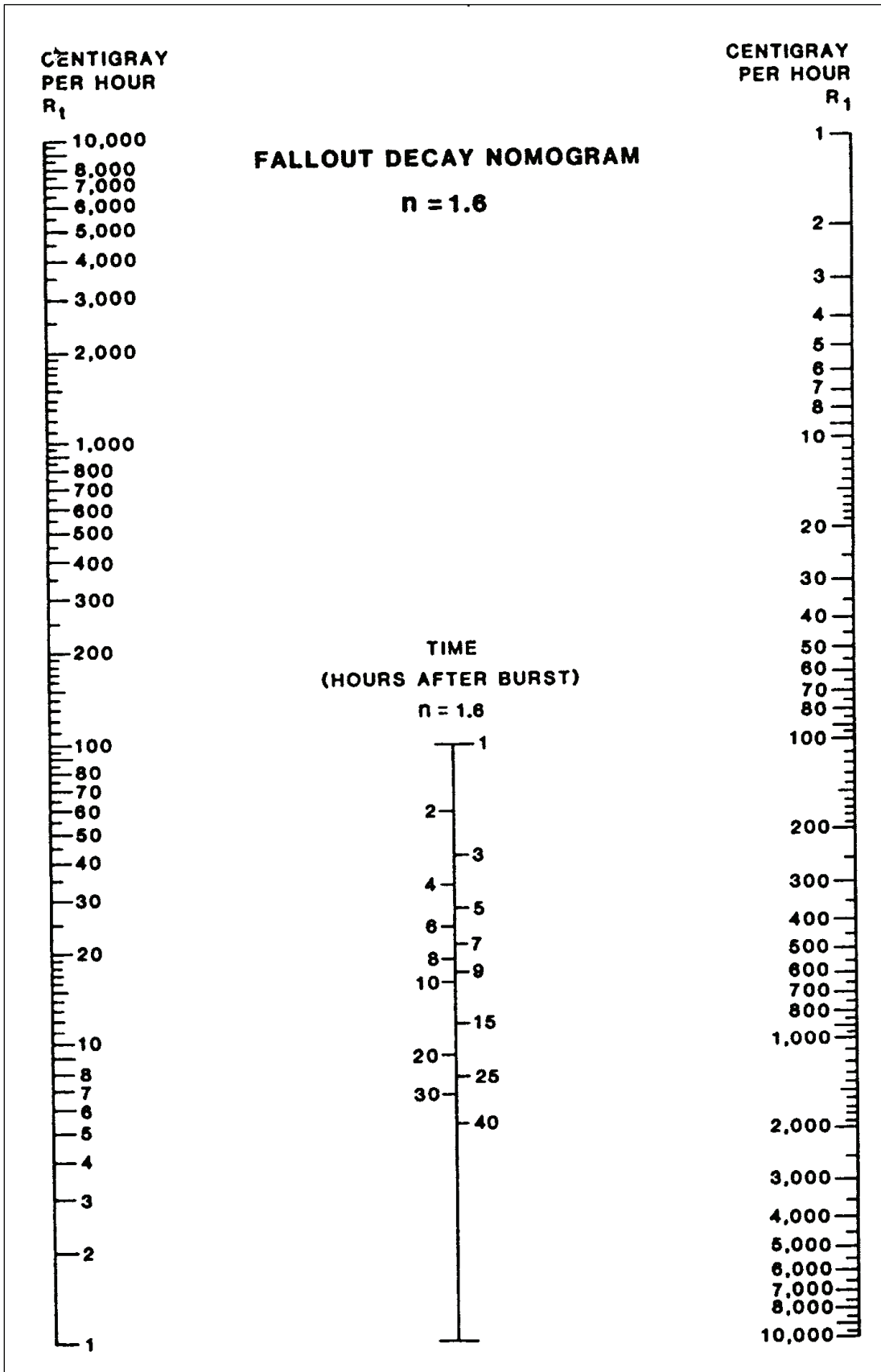
Figure J-23. Fallout Decay Nomogram (n=1.6)
