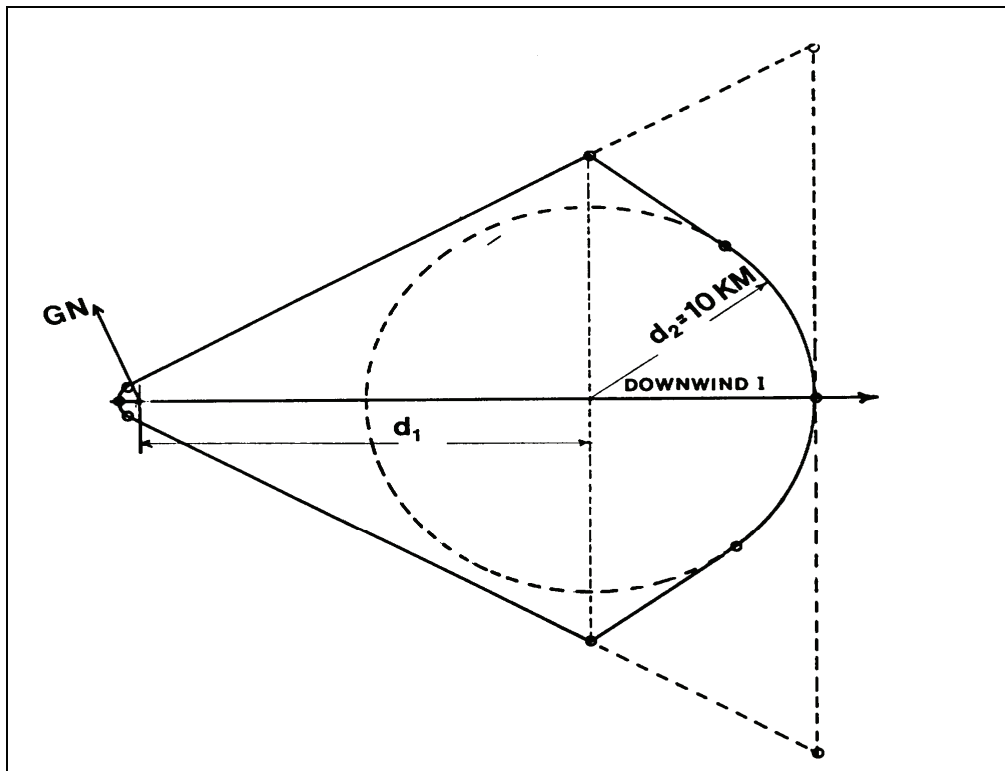
Figure E-17. Recalculation of Downwind Hazard Area Type A Attack (Change In Wind Speed From >10 kph to \leq 10 kph) (Example 3)
