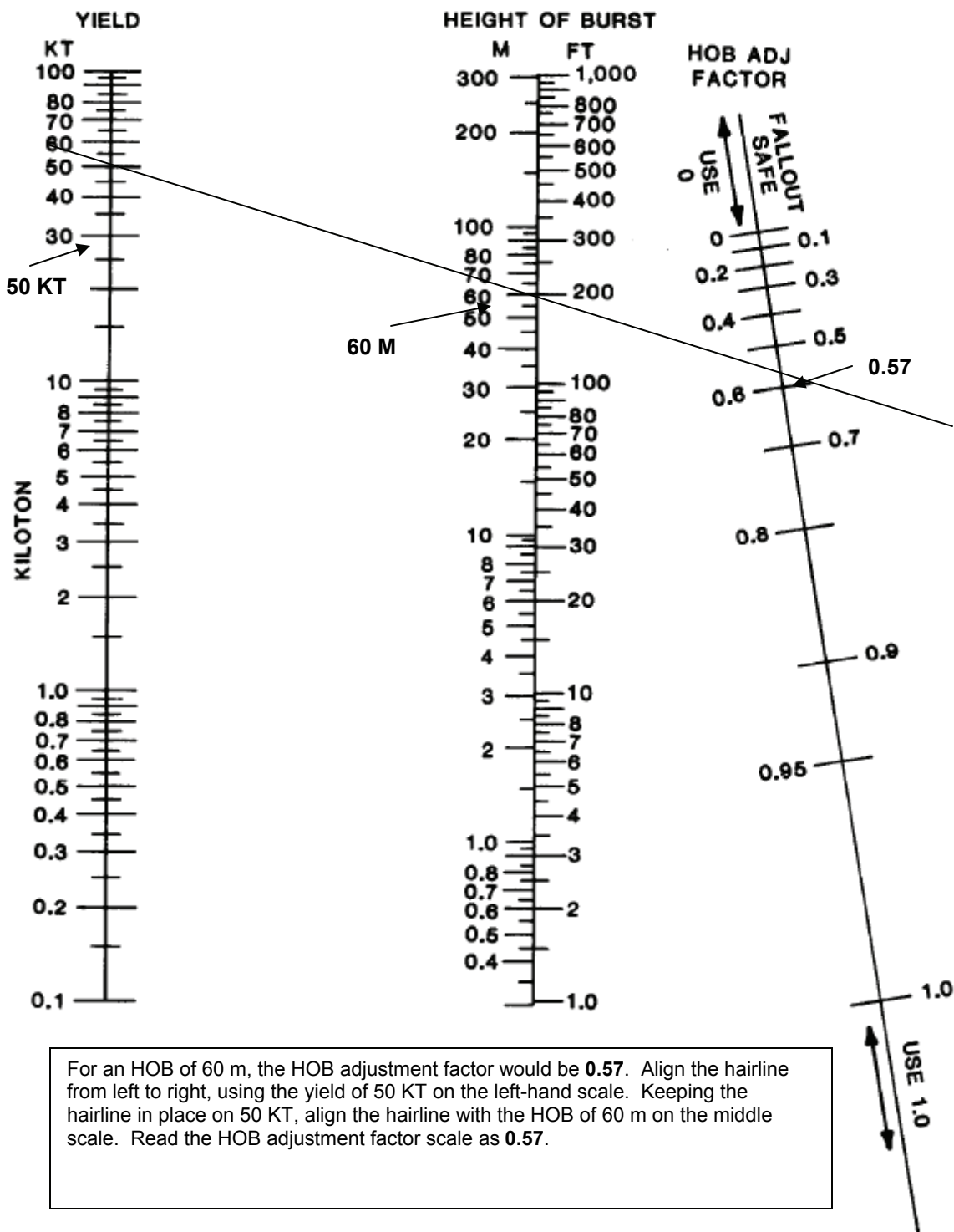
Figure G-24. HOB (Kilaton) Adjustment Factor (Example)
