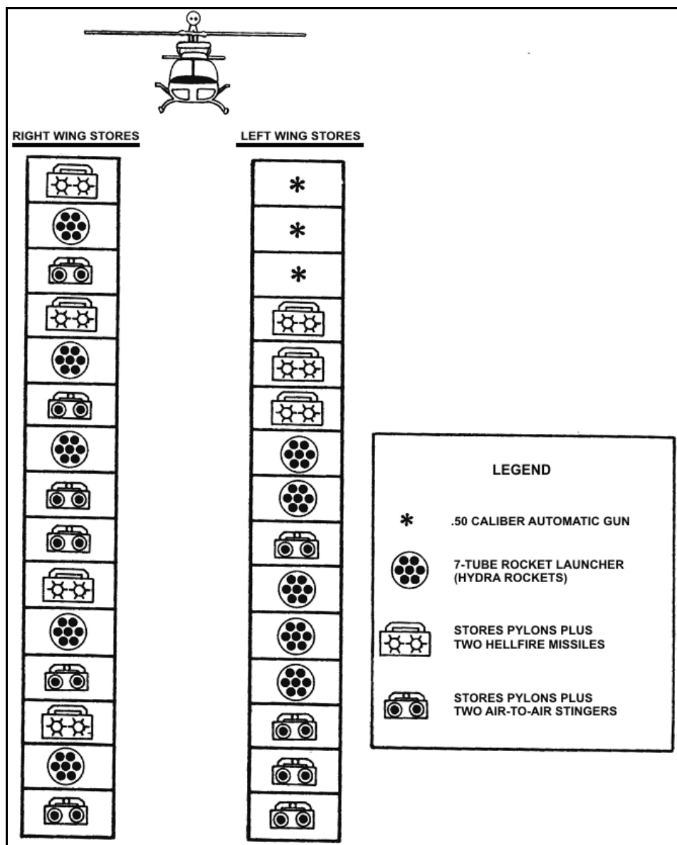
Figure F-2. OH-58D authorized armament configurations
