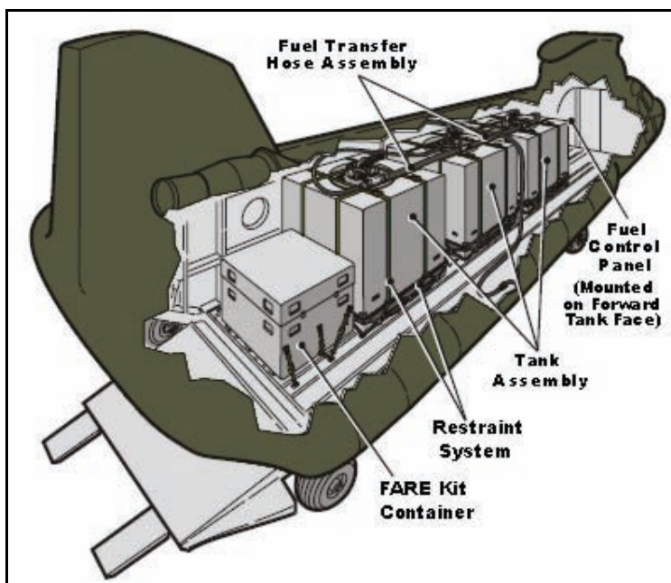
Figure 3-8. Extended range fuel system II functional components
