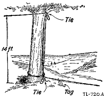
FIGURE 80.—Method of tying wire at junction of surface line with overhead construction.
