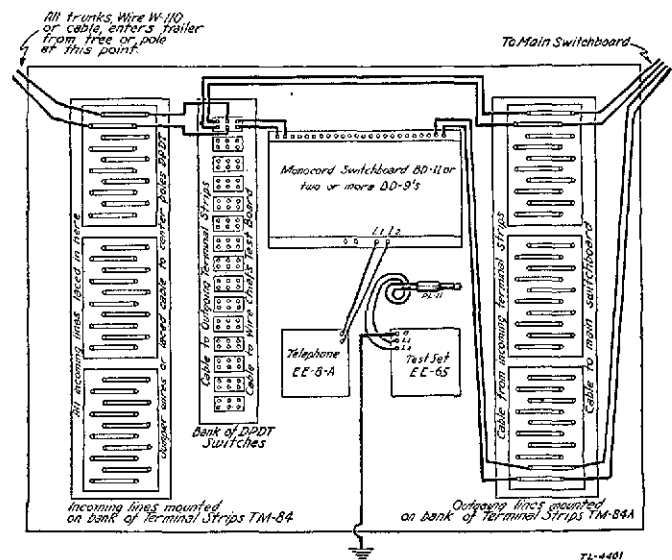
FIGURE 89.—Wiring diagram for the suggested construction center.
