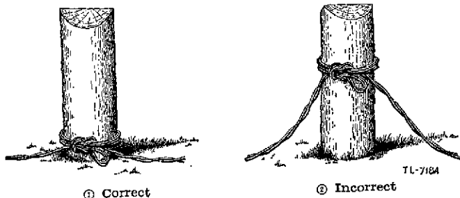
① Correct ② Incorrect FIGURE 78.—Method of tying wire at ground level.
