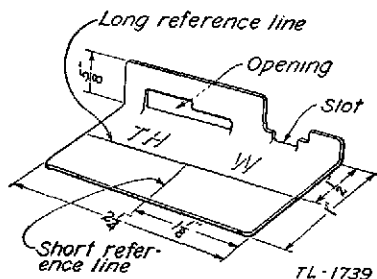
FIGURE 66.—Gaff gage TL-144.
