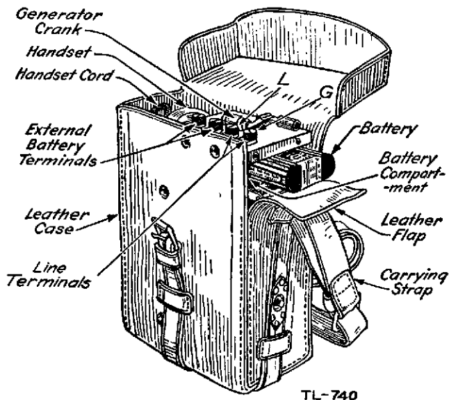
FIGURE 116.—Telephone EE-5.
