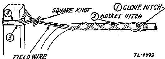
FIGURE 61.1.—Basket hitch tie.
