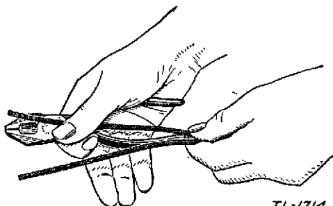
FIGURE 35.—Staggering splice.
