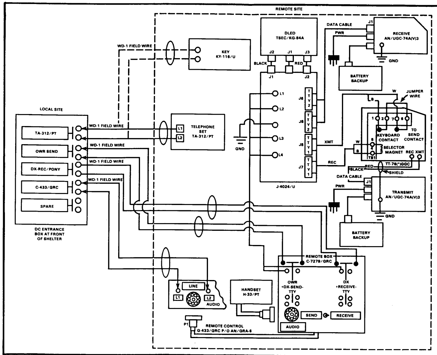
Figure 1-11. Wiring diagram for secure remote operation or Radio Teletypewriter Set AN/GRC-122 with TSEC/KG-84A in duplex operation with TT-76 in line.
