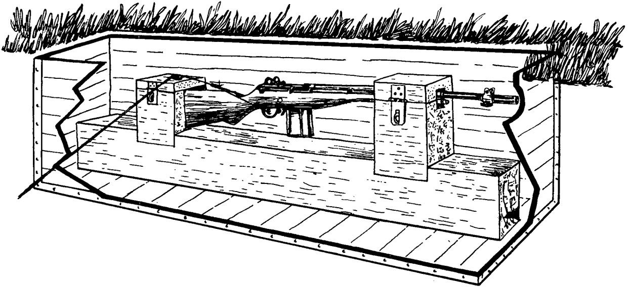
Figure 92. Rifle mount for installation in pit.
