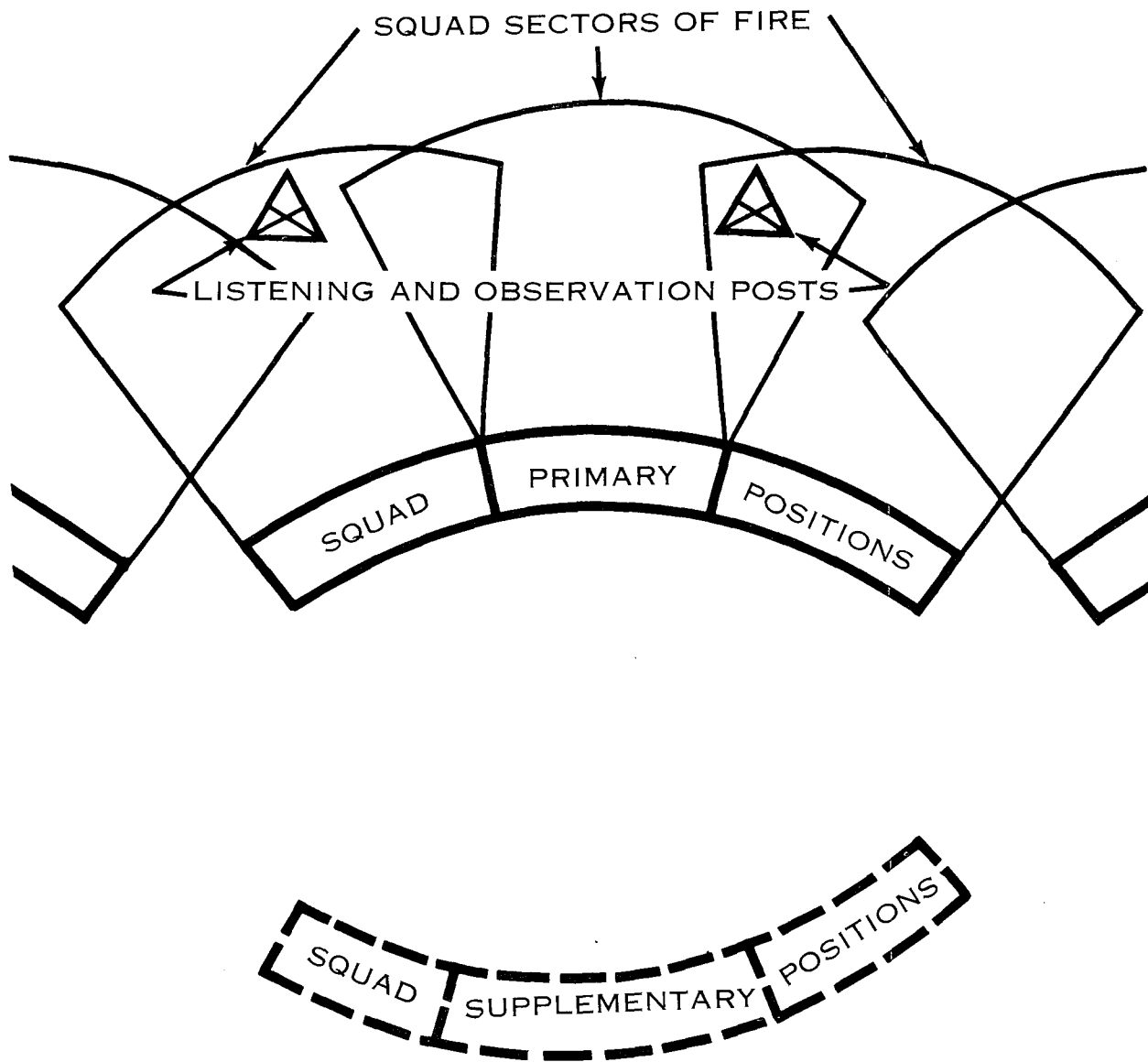
Figure 36. Defensive positions.
