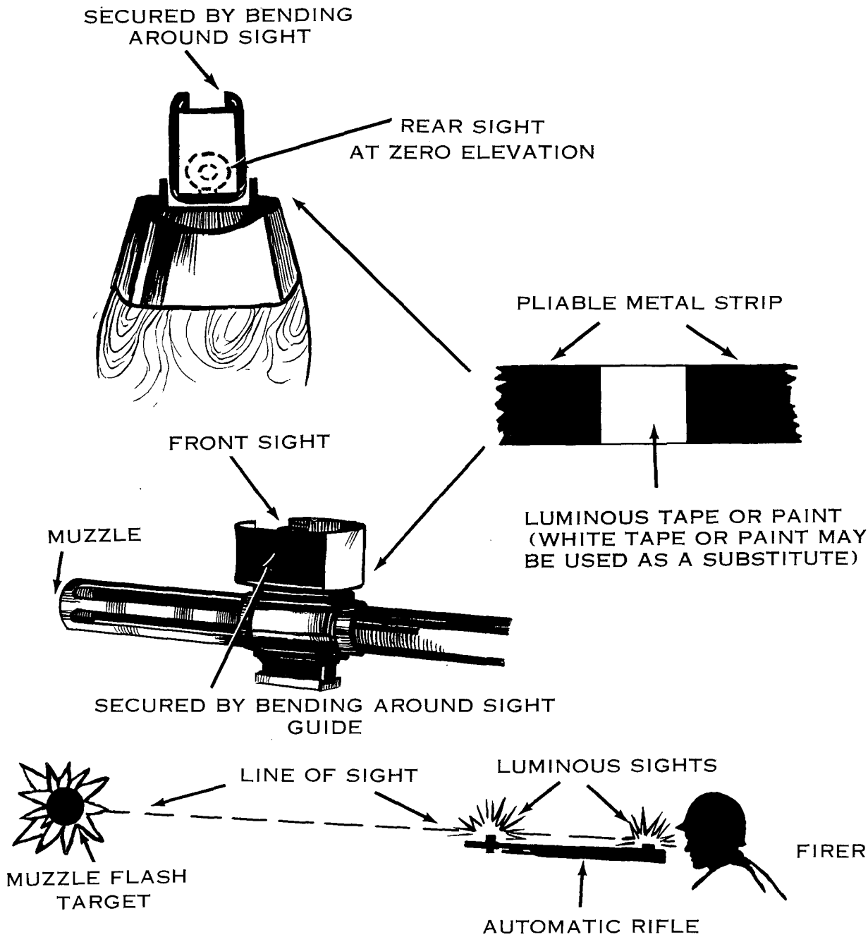
Figure 26. Field expedient night sight and sight picture for the automatic rifle.
