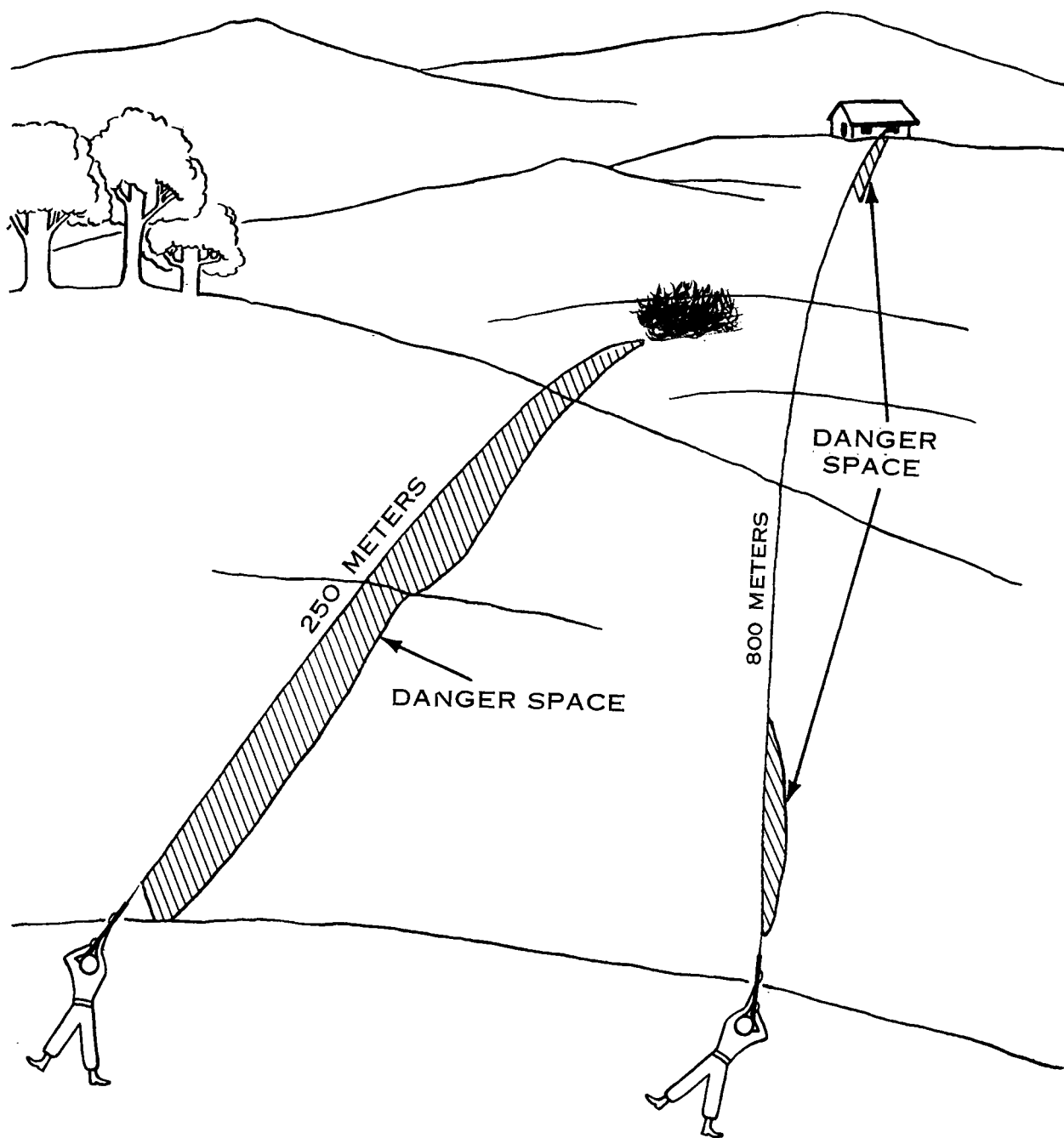
Figure 6. Danger space.
