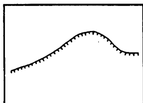
Figure 314. Escarpment. The continuous line represents the point of abrupt change in slope. Tick marks point downslope.
