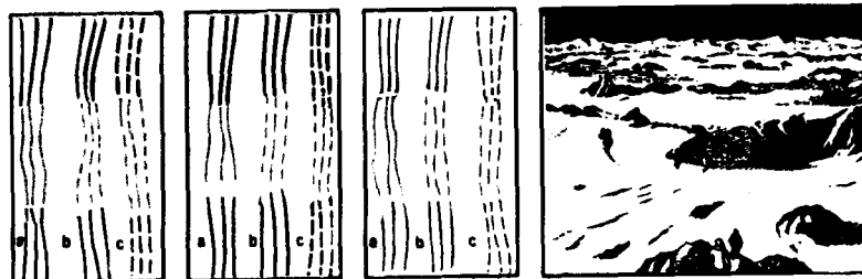
Figure 66. Glacier. Depending upon available information, shapes within the glacial area are shown as: (a) Approximate contours. (b) Form lines.
