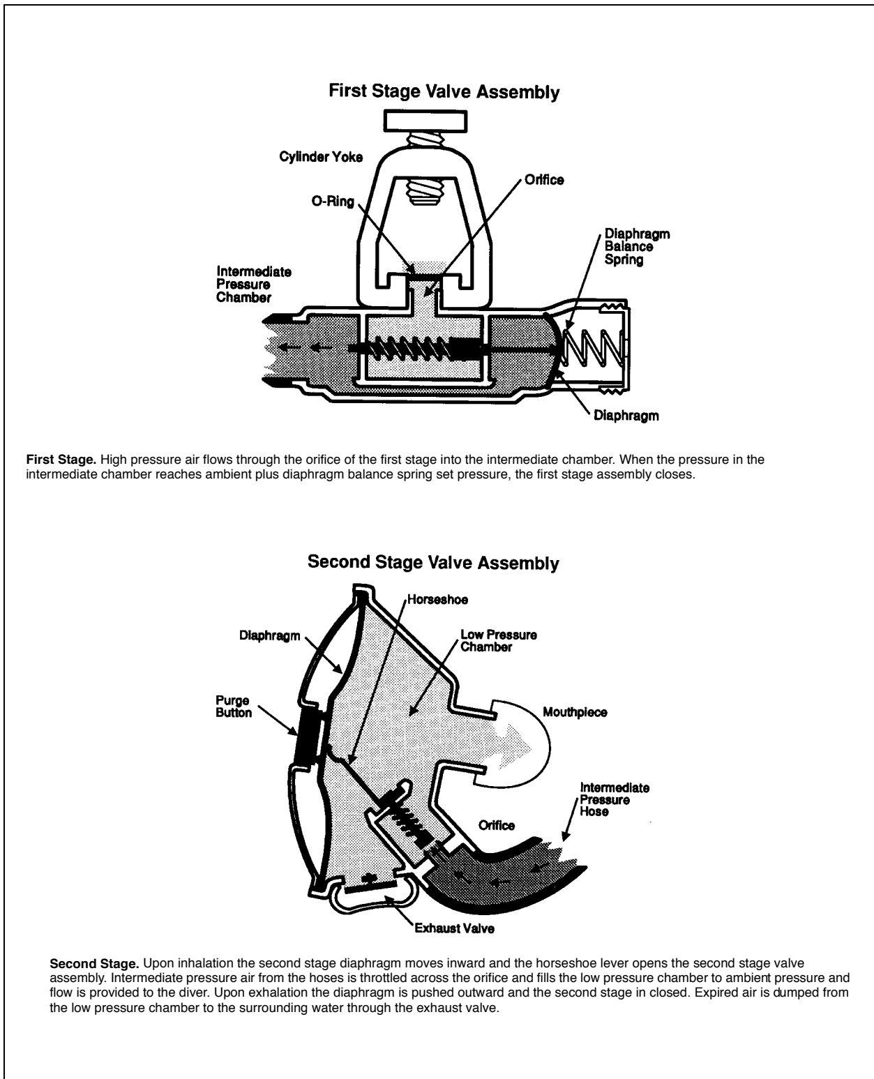
Figure 7-1. Schematic of Demand Regulator.
