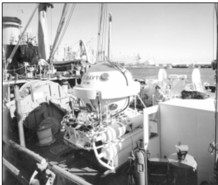
Figure 1-19. DDS MK 1 Personnel Transfer Capsule.
