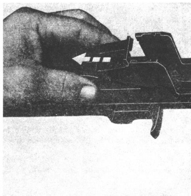
Figure 6. Removing the bullet guide, follower arm, and operating rod catch assembly.
