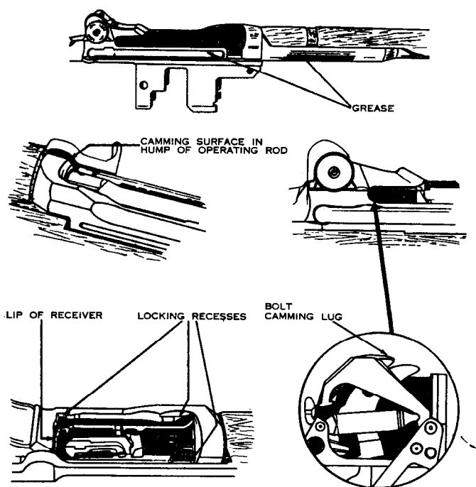
Figure 33. Points to apply rifle grease.
