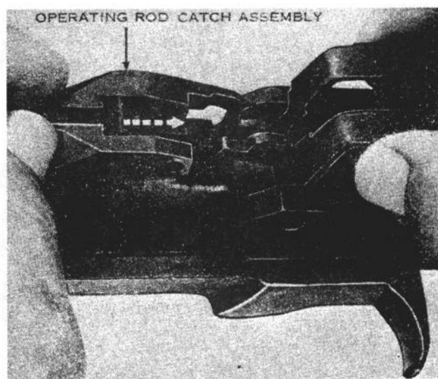
Figure 14. Replacing the operating rod catch assembly.
