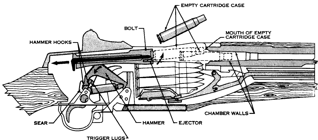
Figure 31. Ejecting and cocking.
