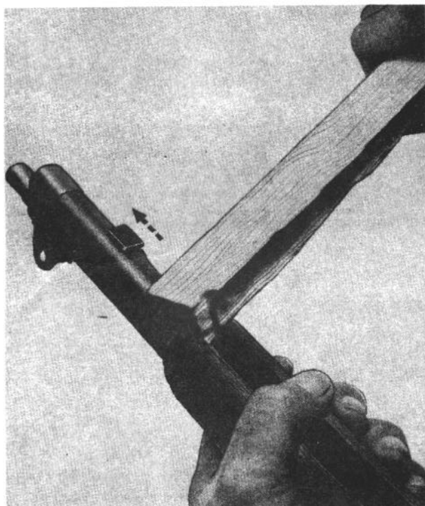
Figure 9. Removing the gas cylinder.
