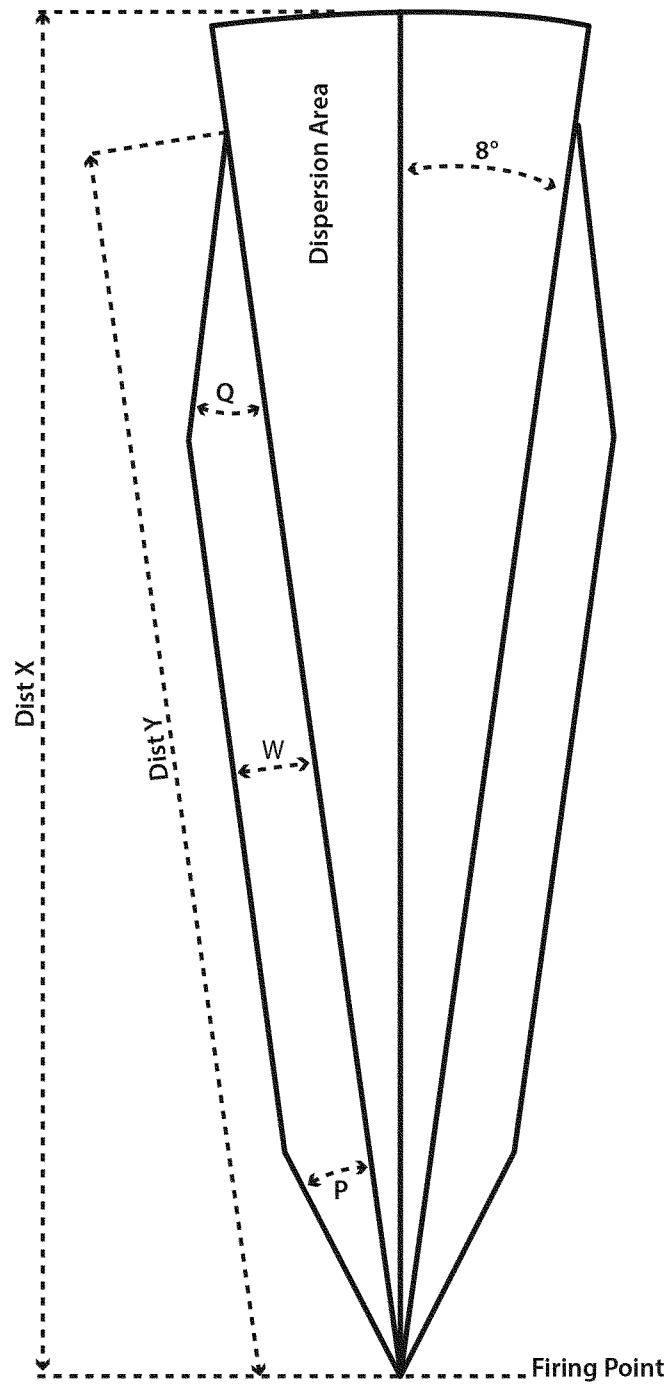
Figure 4-4. Batwing surface danger zone for firing 5.56mm M1037 Short Range Training Ammunition
