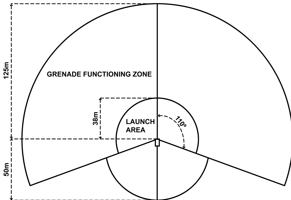
Figure 8-10. Surface danger zones for firing L8A1/A3 smoke grenades
