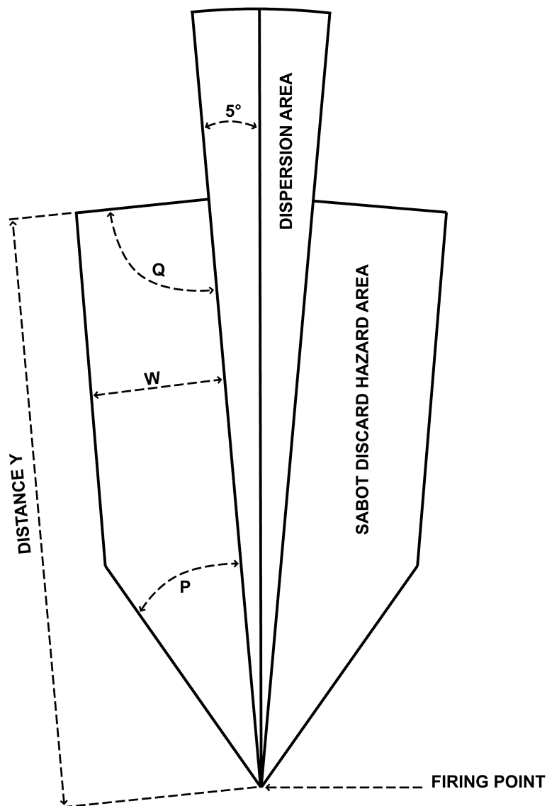
Figure 8-9. 30mm discard hazard area
