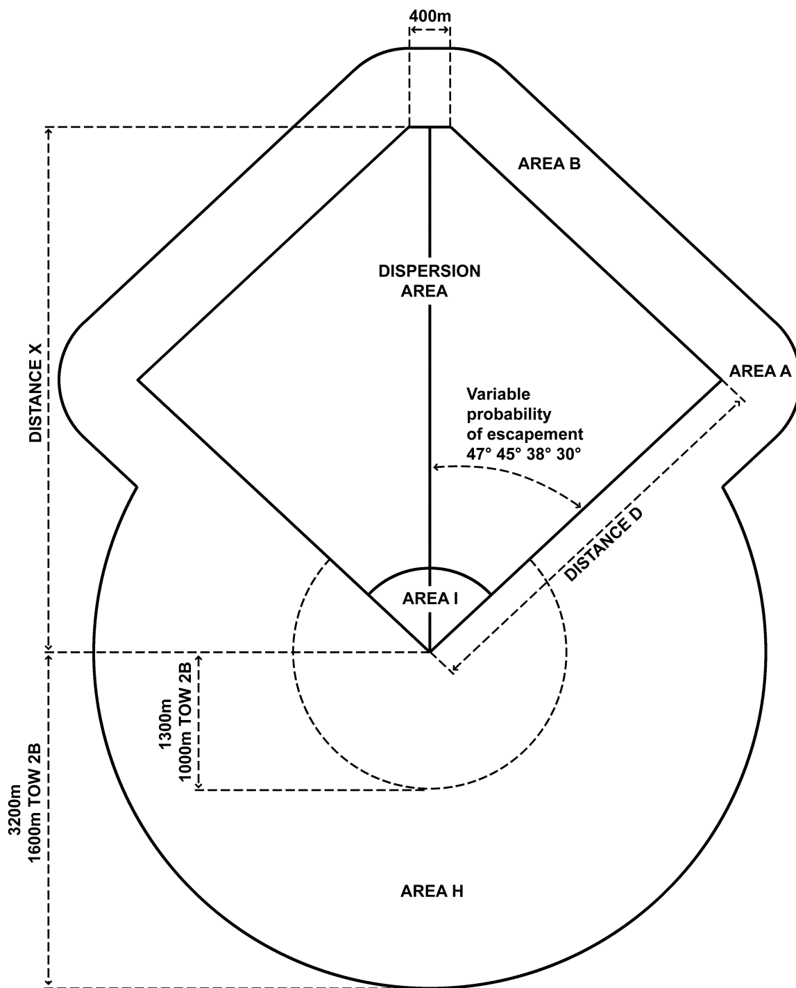
Figure 7-1. Surface danger zone for firing basic TOW, practice TOW, ITOW, TOW 2A, TOW 2B, TOW 2B AERO, and TOW BB missiles
