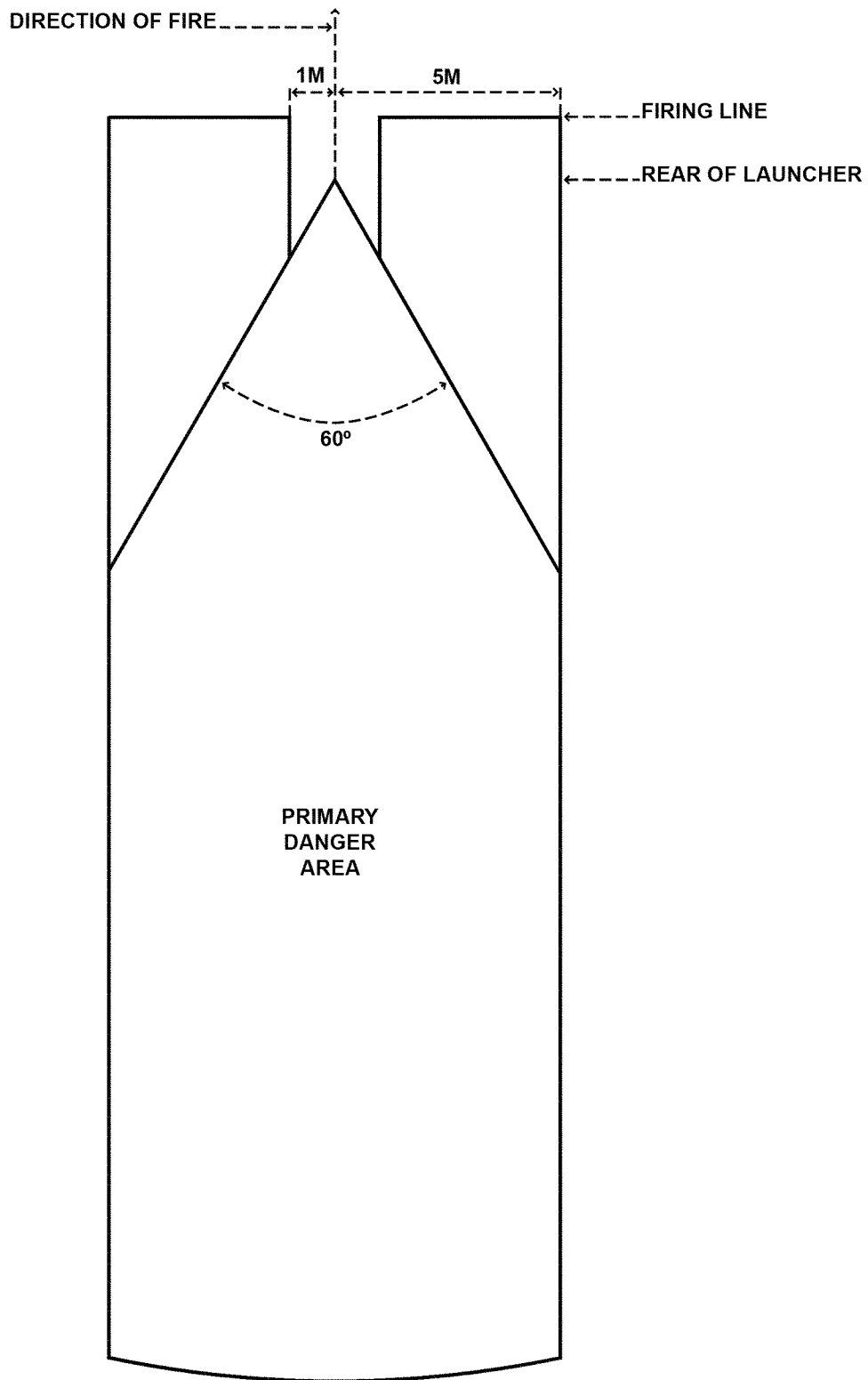
Figure 7-8. Primary danger area, Area F, extension for activation of the Javelin missile flight motor pressure relief system
