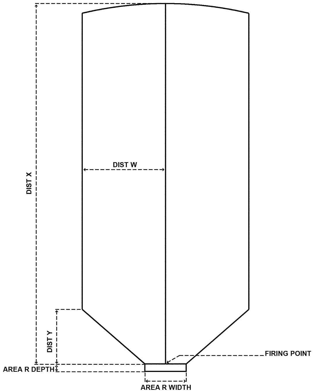
Figure 8-3. Surface danger zone for M865 and M1002 sabot petal discard hazard
