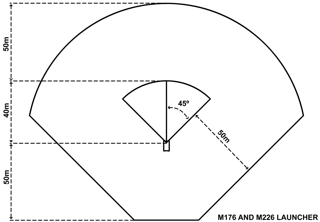
Figure 8-11. Surface danger zones for firing grenades from M176, M226, and M239 grenade launchers
