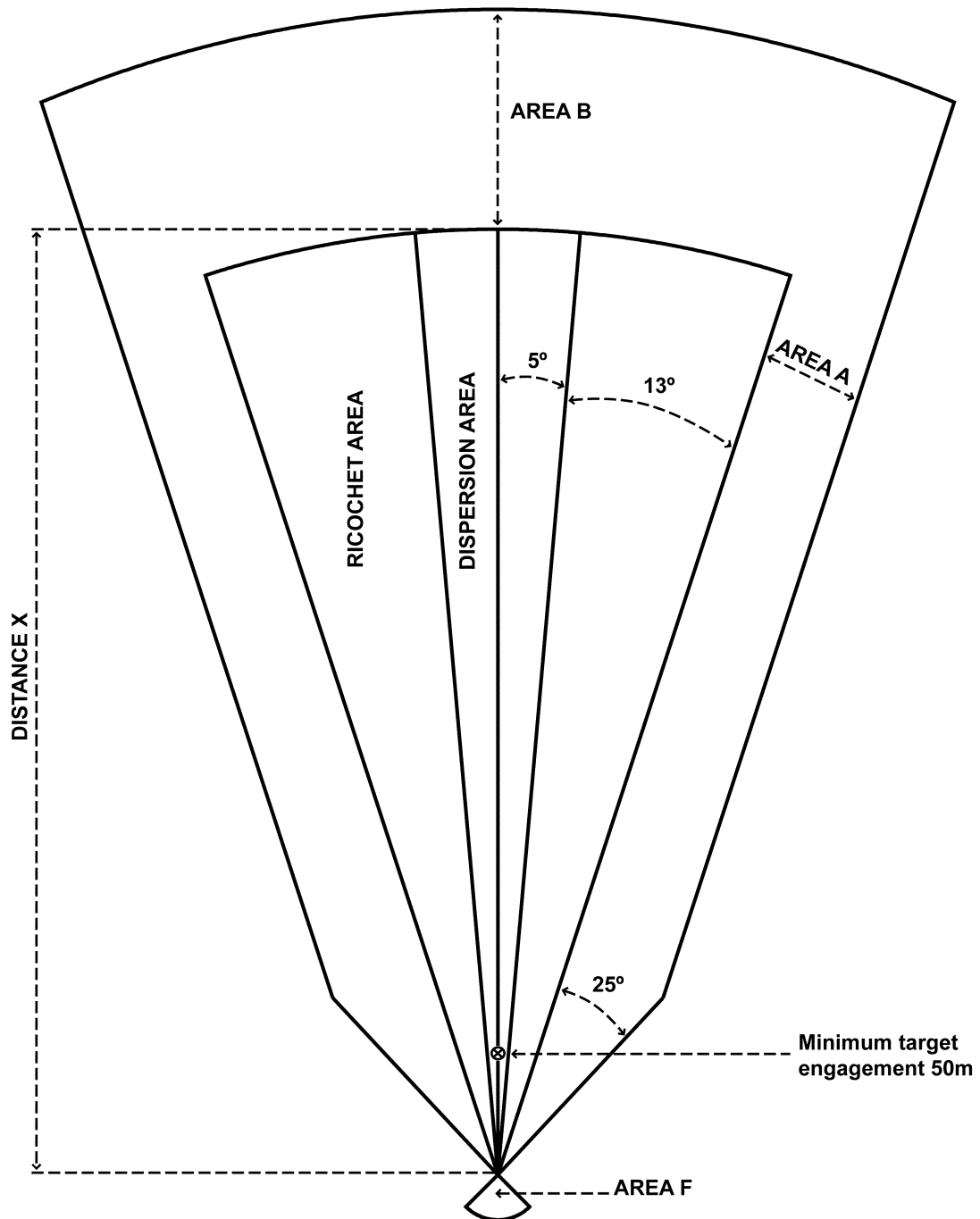
Figure 6-5. Surface danger zone for firing AT4
