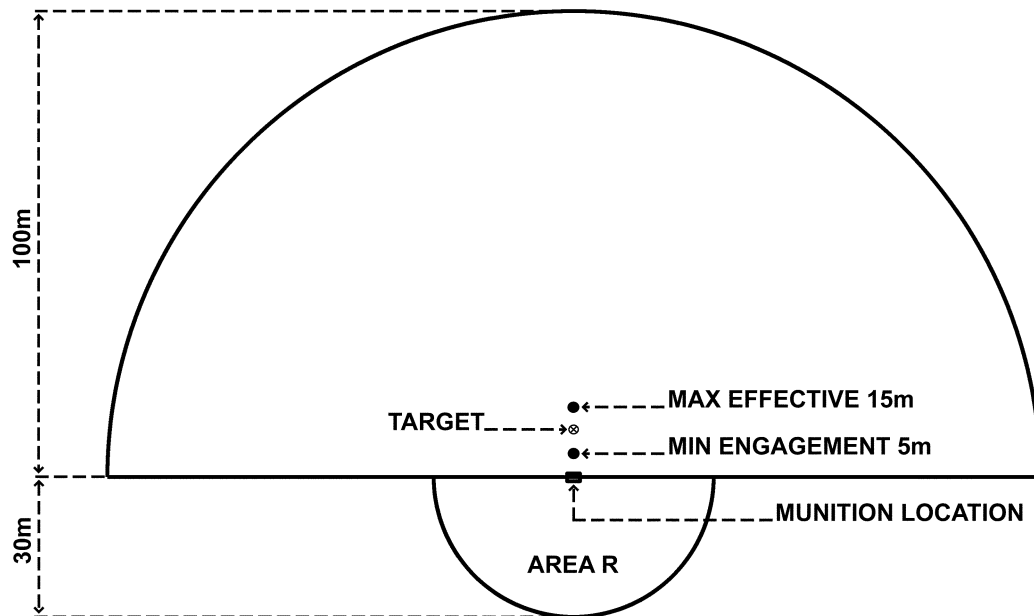
Figure 14-6. Surface danger zone for modular crowd control munition (WA97)
