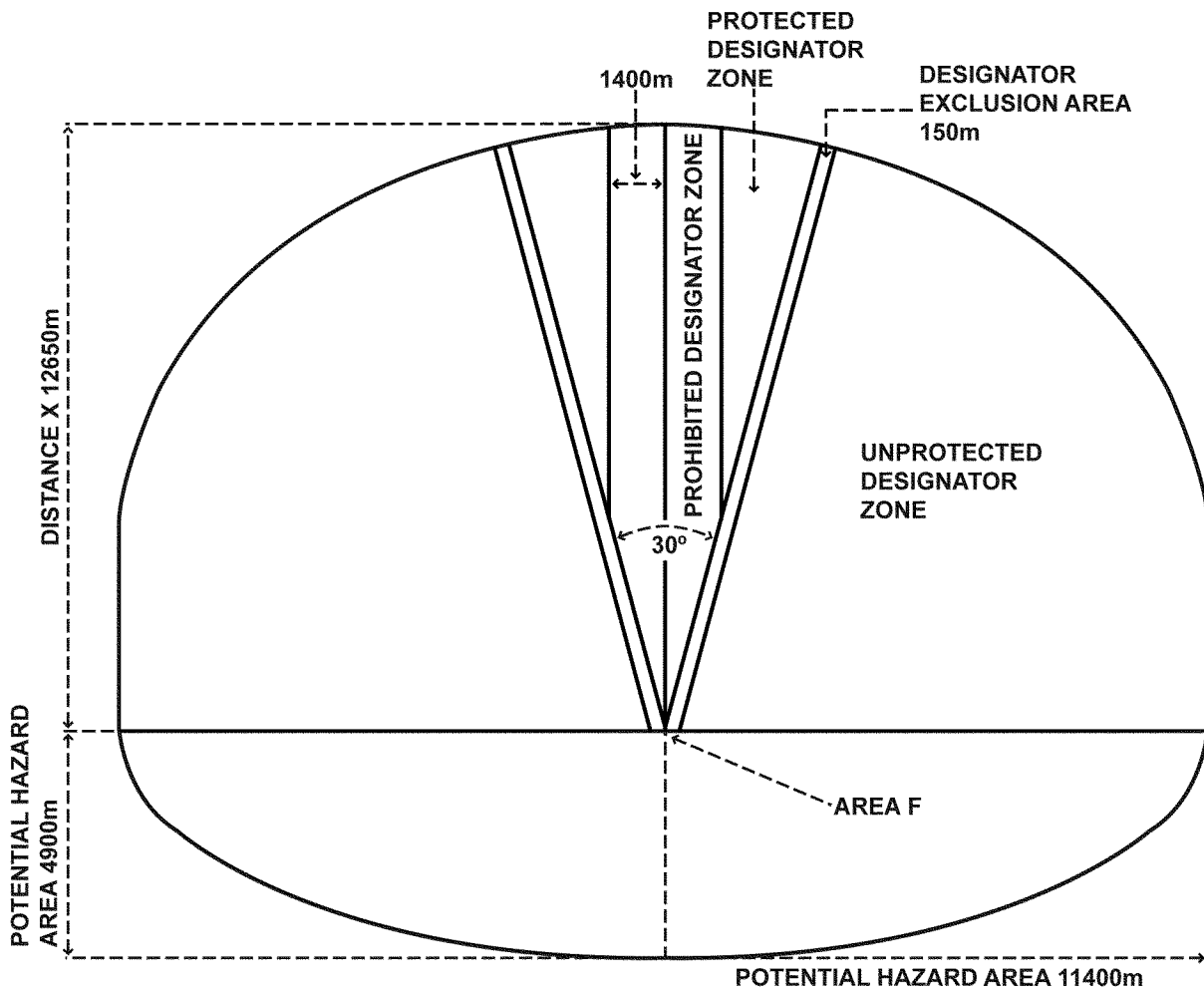
Figure 11-6. Expanded direct weapons danger zone/surface danger zone (Army RW only) for firing AGM-114 A/F HELLFIRE laser-guided missile with associated missile tip-off error in direct launch mode at fixed target (Lock-On-After-Launch autonomous or Lock-On-Before-Launch with remote designation)
