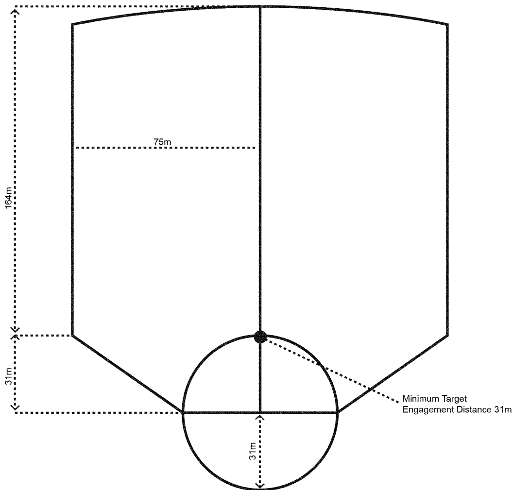
Figure 14–11. Surface danger zone for the non-lethal/tube launched munition system
