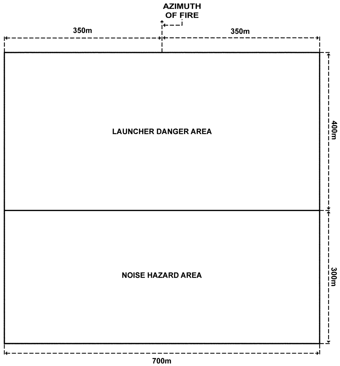
Figure 10-13. Area F for Multiple Launch Rocket System/High Mobility Artillery Rocket Systems reduced range practice rocket
