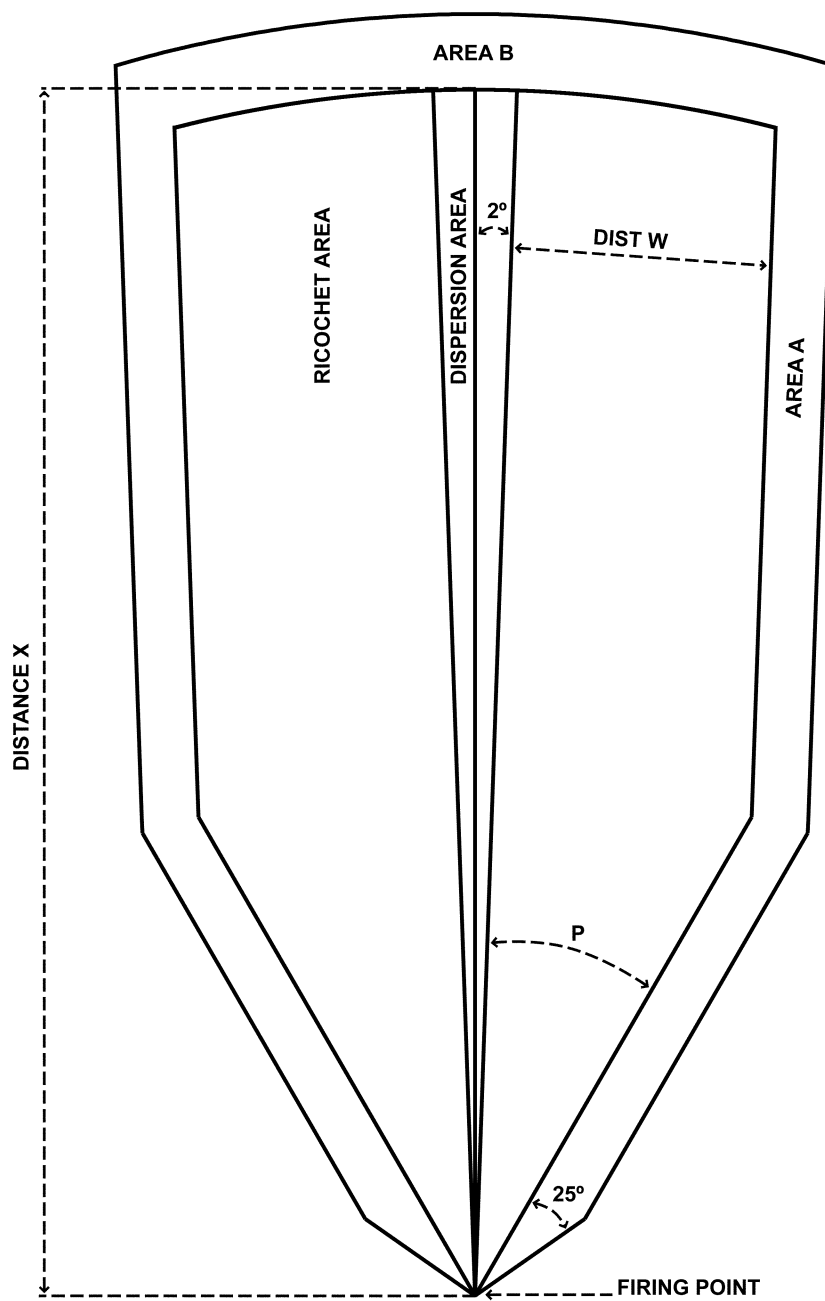
Figure 8-5. Surface danger zone for firing 25mm and 30mm cannon cartridges
