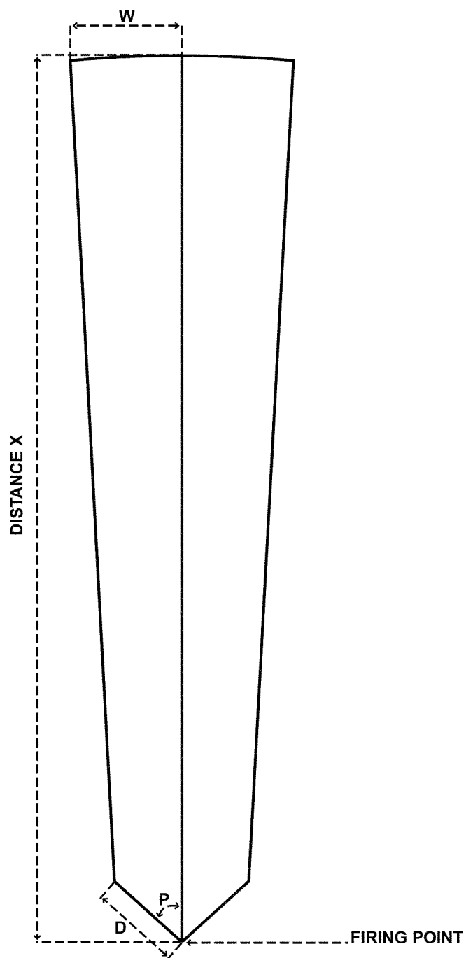
Figure 4-6. Surface danger zone for M903, M962, MK211, and MK 211-0 .50 caliber ammunition
