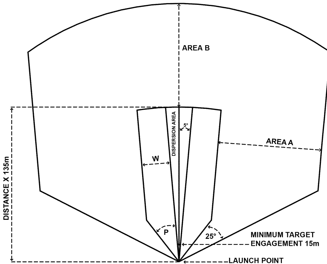
Figure 15-10. Surface danger zone for the Rifle Launched Entry Munition and Grenade Rifle Entry Munition
