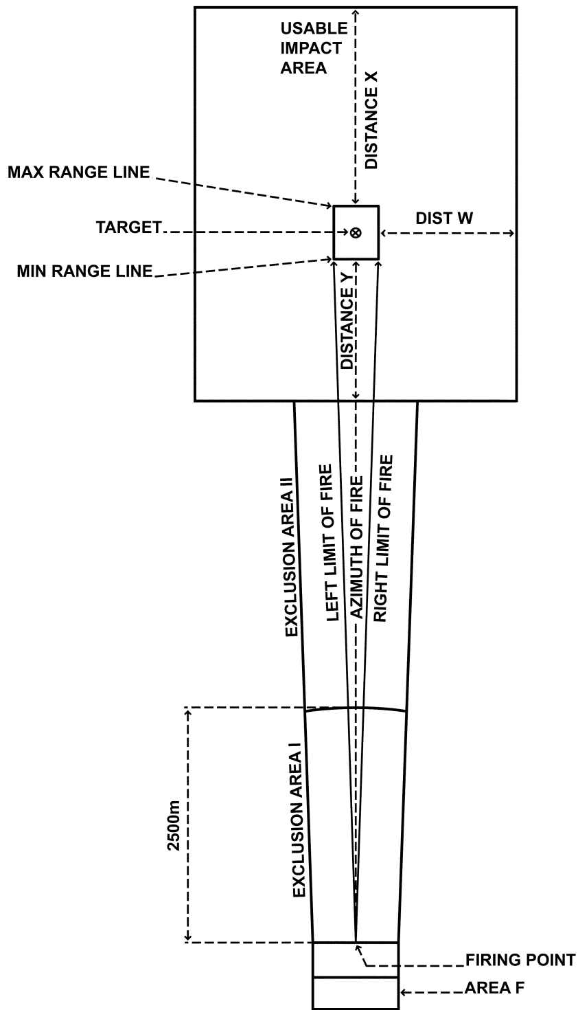
Figure 10-10. Surface danger zone for firing Multiple Launch Rocket System/High Mobility Artillery Rocket Systems reduced range practice rocket point to point
