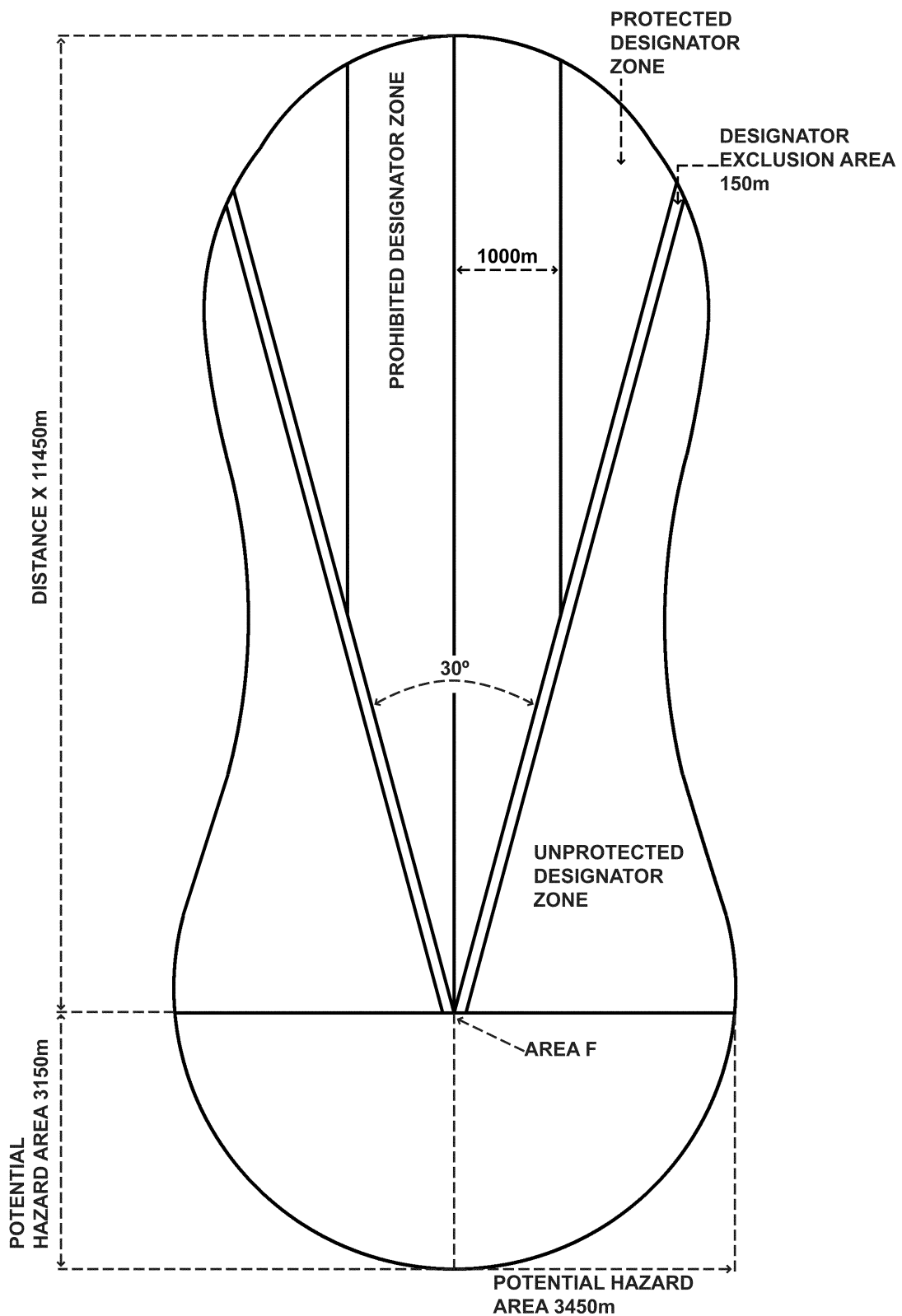
Figure 11-4. Directed fire surface danger zone for firing AGM-114 A/F HELLFIRE laser-guided missiles in direct launch at fixed target (Lock-On-After-Launch autonomous or Lock-On-Before-Launch with remote designation)
