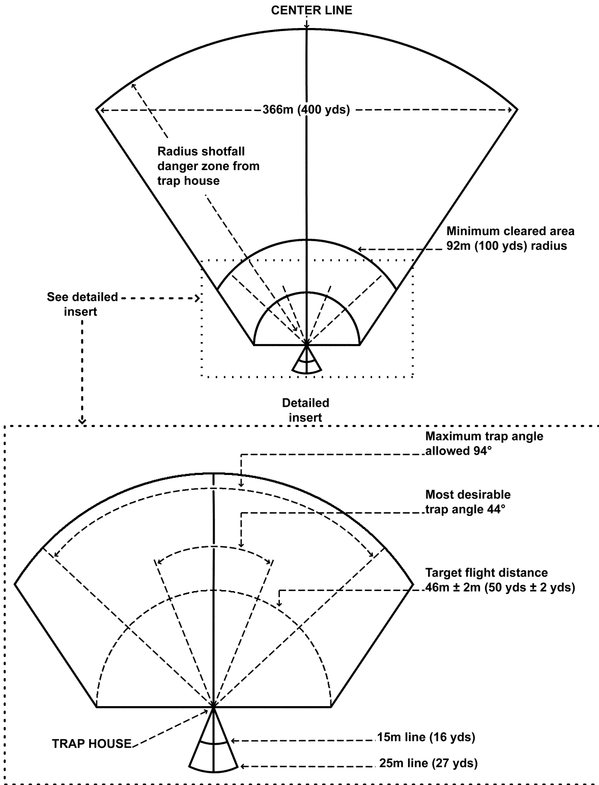
Figure 4-8. Surface danger zone for shotfall
