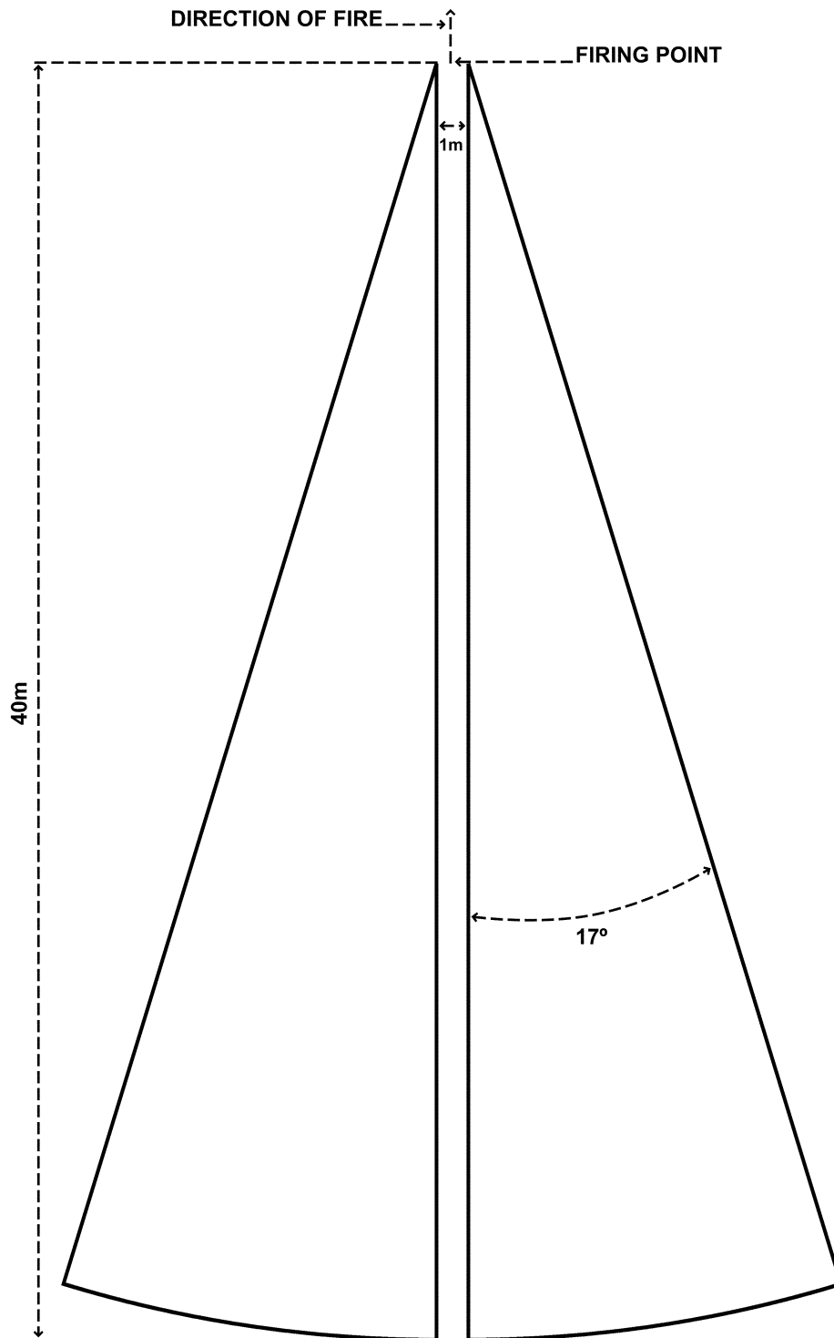
Figure 7-4. Area F for ATWESS and TOW missiles (Multiple Integrated Laser Engagement System training)
