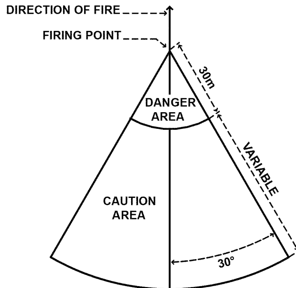
Figure 6-9. Surface danger zone, Area F, for firing SMAW-NE, -HEAA, -HEDP, and common practice round
