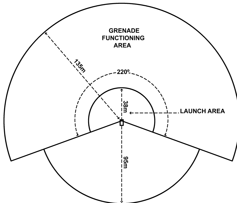
Figure 8–12. Surface danger zones for firing M81 grenade using standard 66mm launchers on armored vehicles
