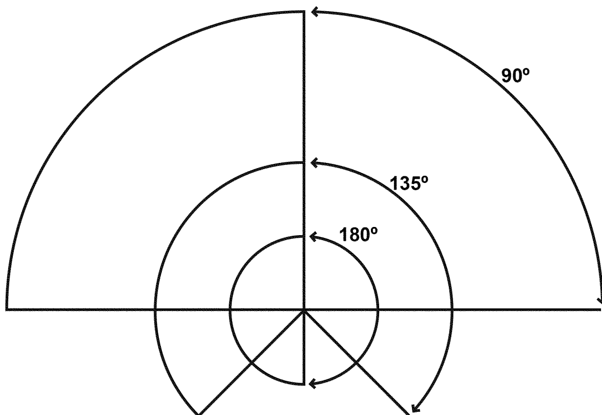
Figure 8–14. Hazardous impulse noise 140 dBP contour zones
