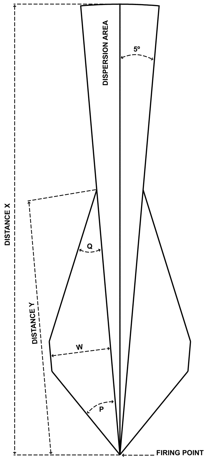
Figure 4-3. Batwing surface danger zone for firing small arms direct-fire weapons without exploding projectiles, except 5.56mm M1037 Short Range Training Ammunition
