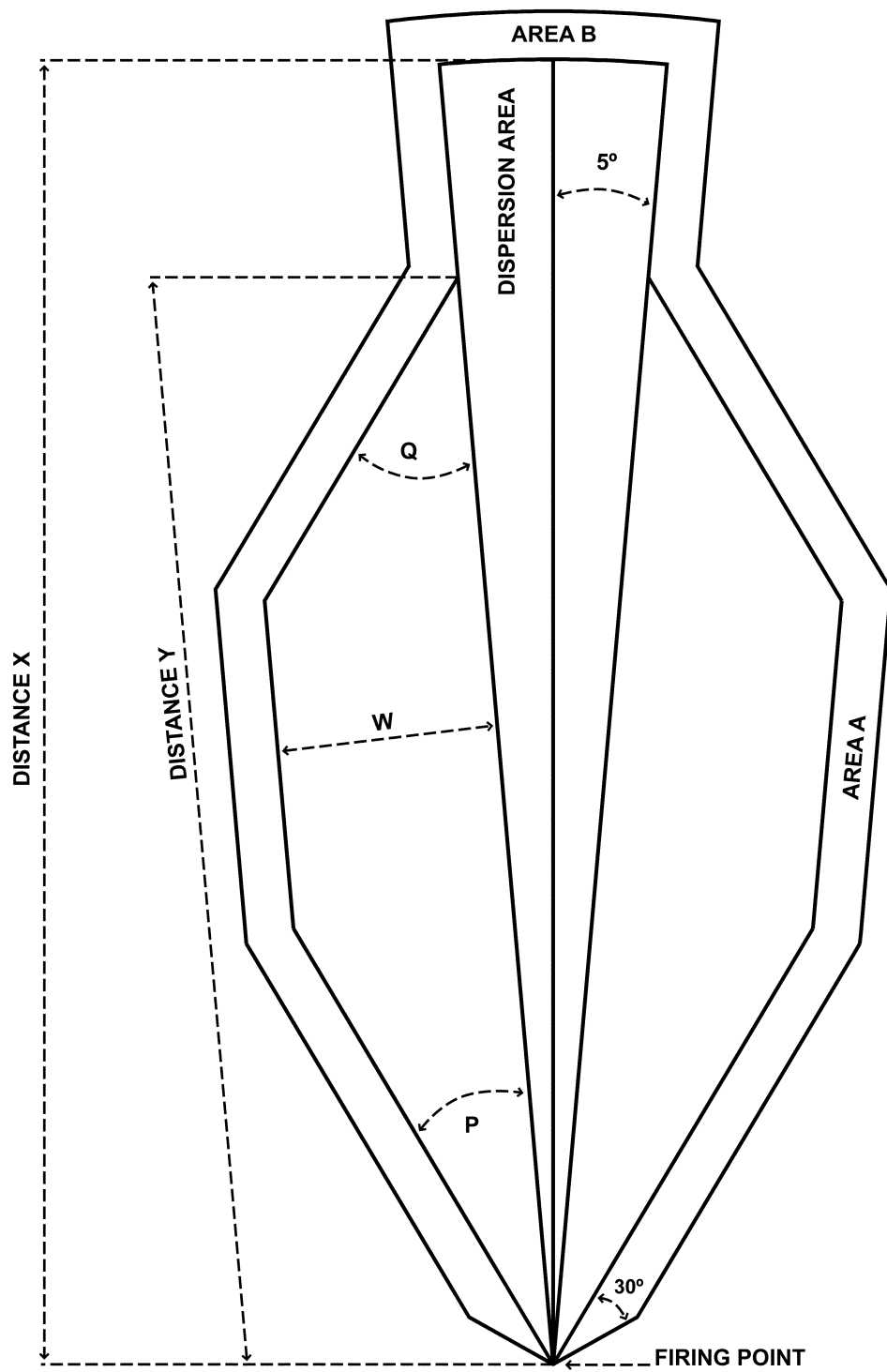
Figure 4-5. Batwing surface danger zone for firing small arms direct-fire weapons with exploding projectiles
