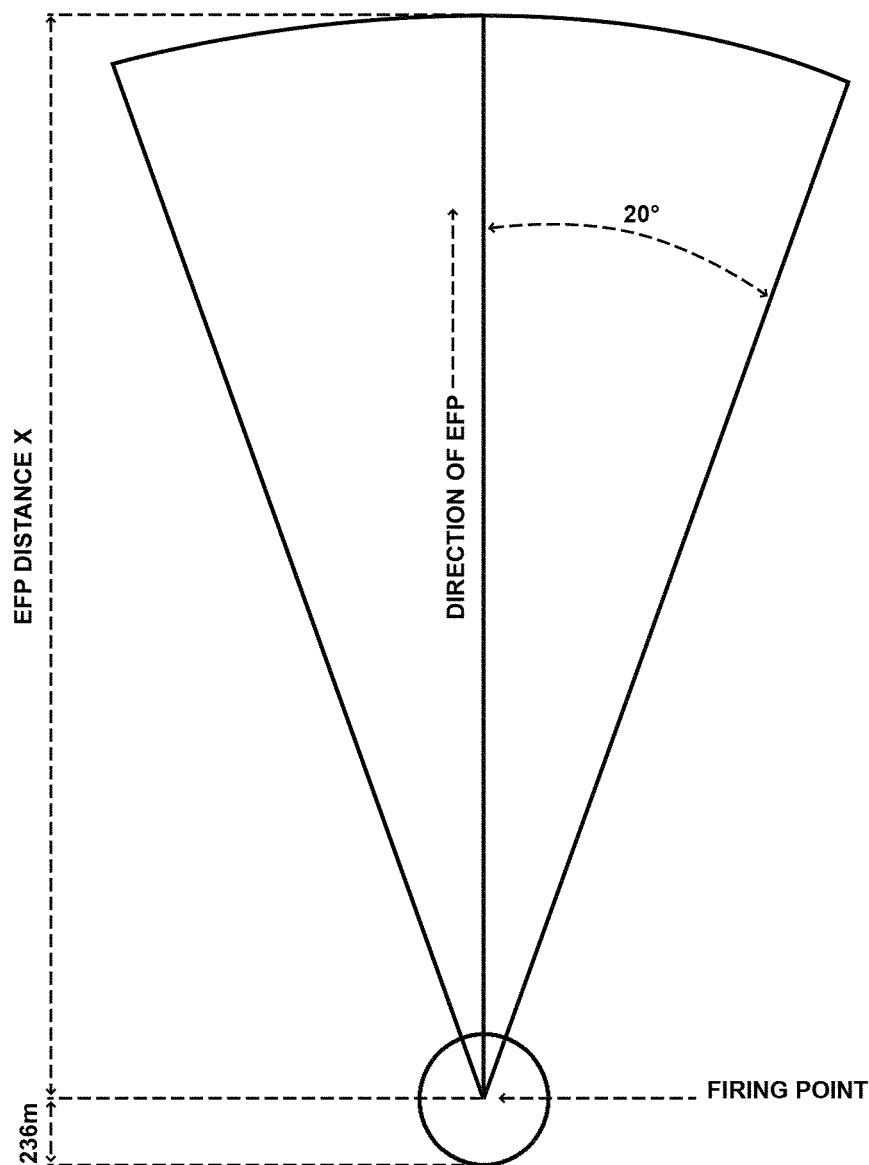
Figure 15–9. Surface danger zone for M2/M4A1 Selectable Lightweight Attack Munition and M3 Demolition Attack Munition
