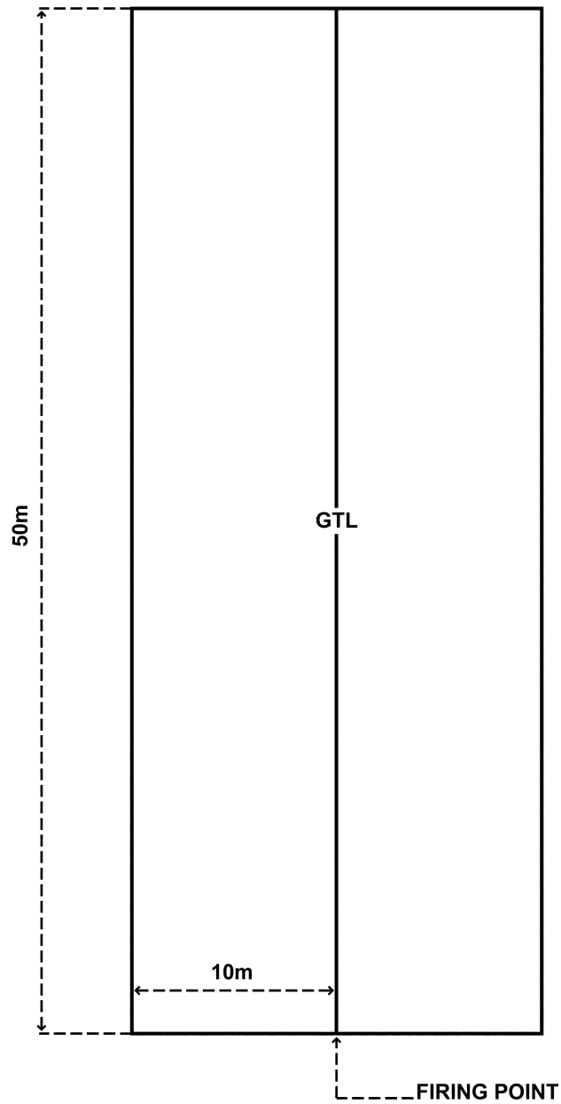
Figure 4-7. Surface danger zone for .50 caliber M903 SLAP and M962 SLAP-T ammunition sabot discard area
