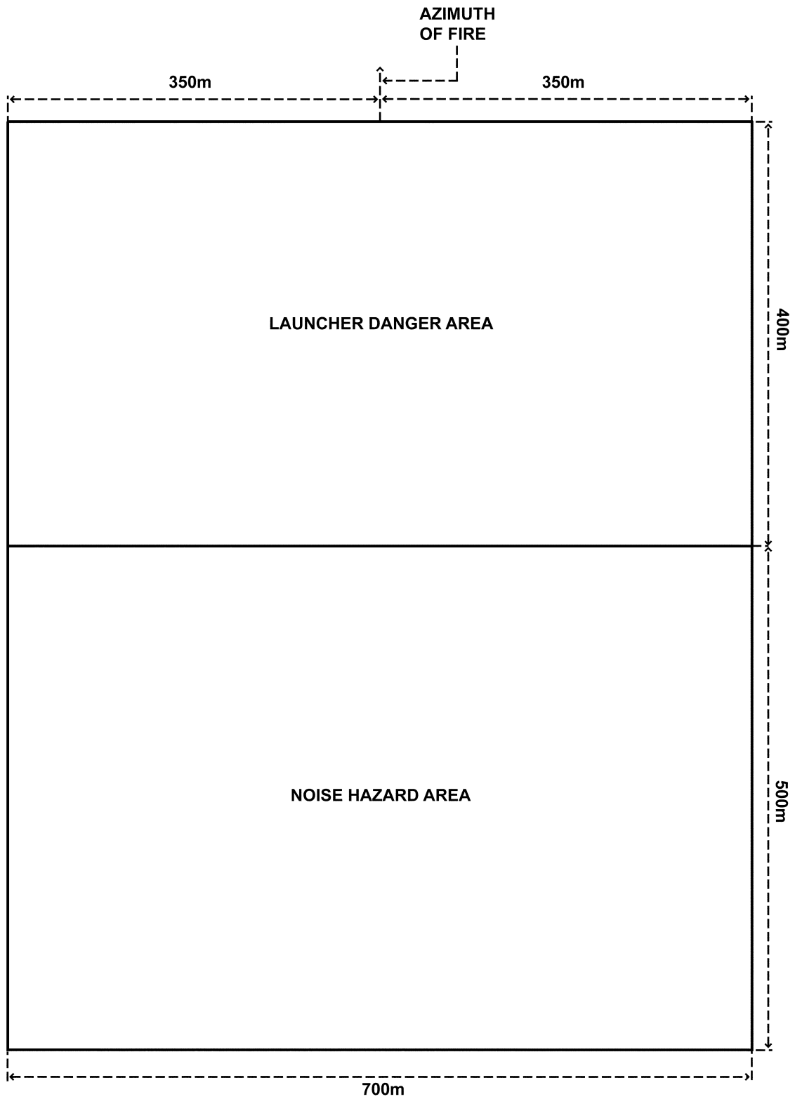
Figure 10-9. Area F for Multiple Launch Rocket System/High Mobility Artillery Rocket System
