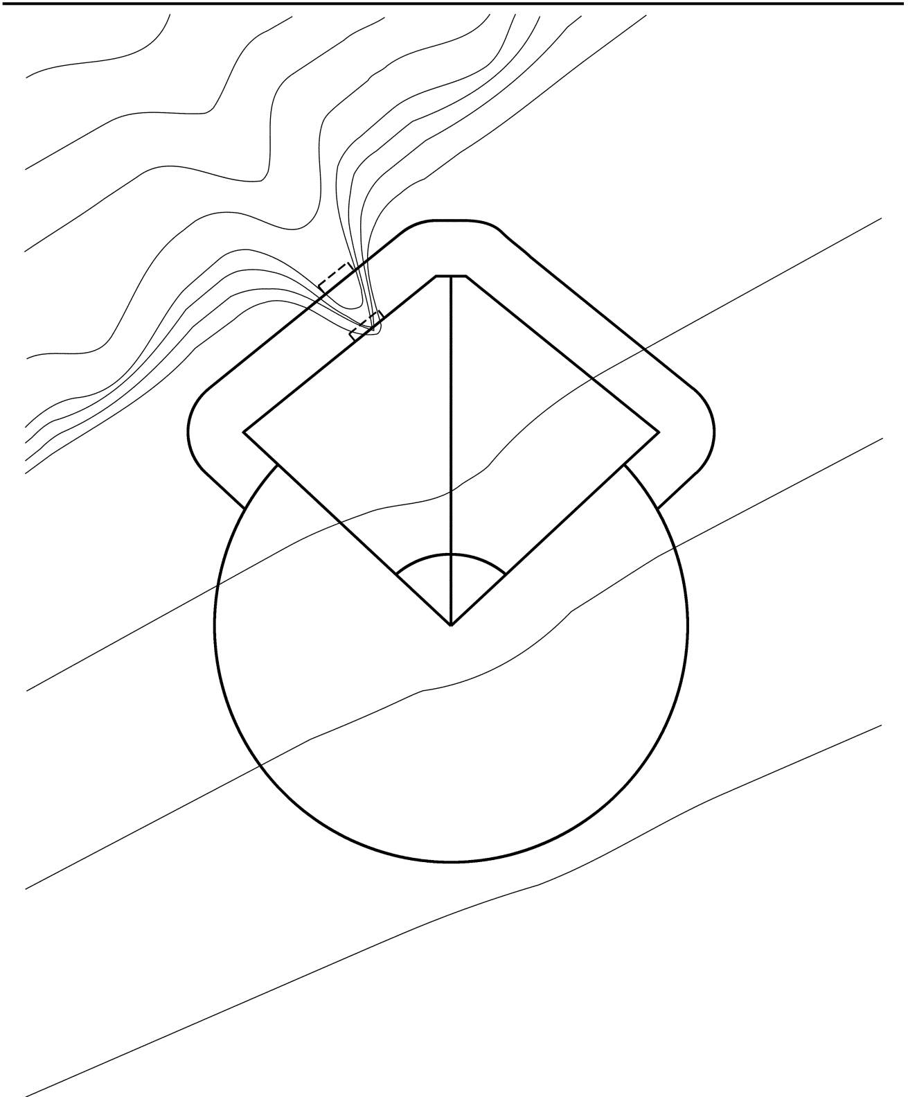
Figure 7-3. Surface danger zone adjustments for firing basic TOW, practice TOW, ITOW, TOW 2A, TOW 2B, TOW 2B AERO, and TOW BB missiles in a ground launch mode
