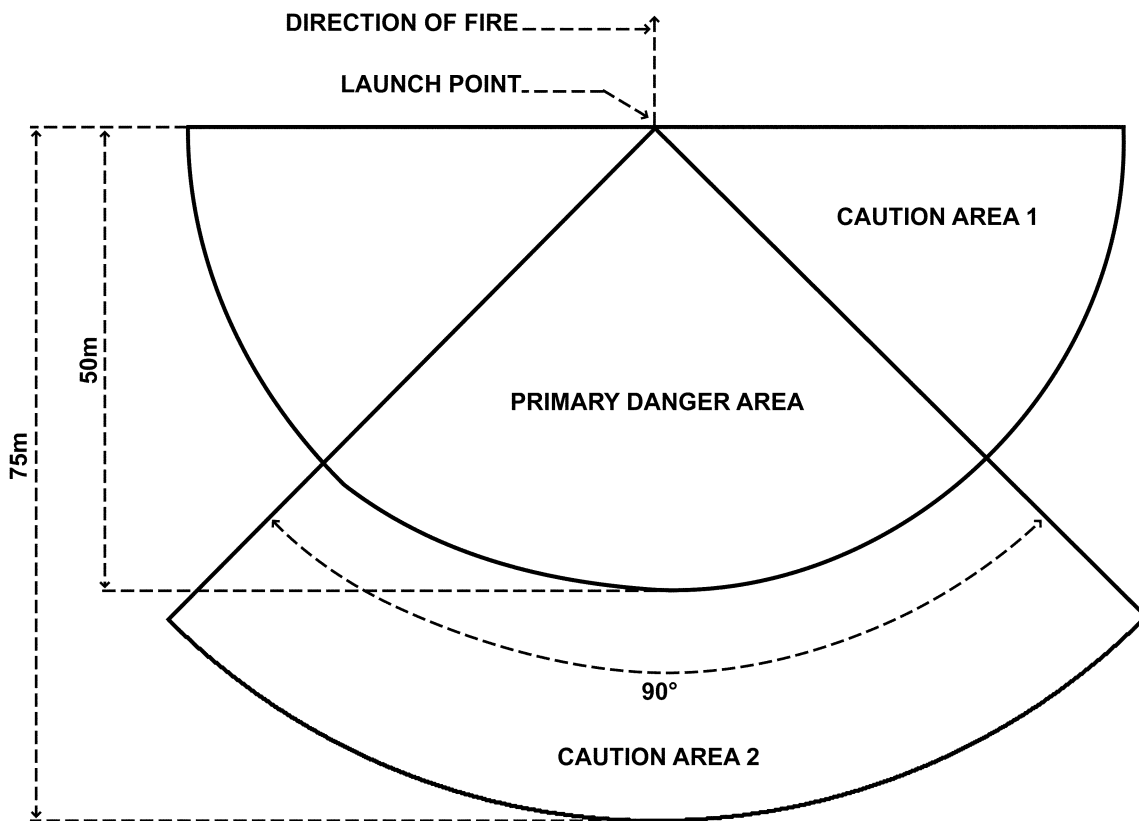
Figure 7-2. Surface danger zone, Area F, for firing basic TOW, practice TOW, ITOW, TOW 2A, TOW 2B, TOW 2B AERO, and TOW BB missiles
