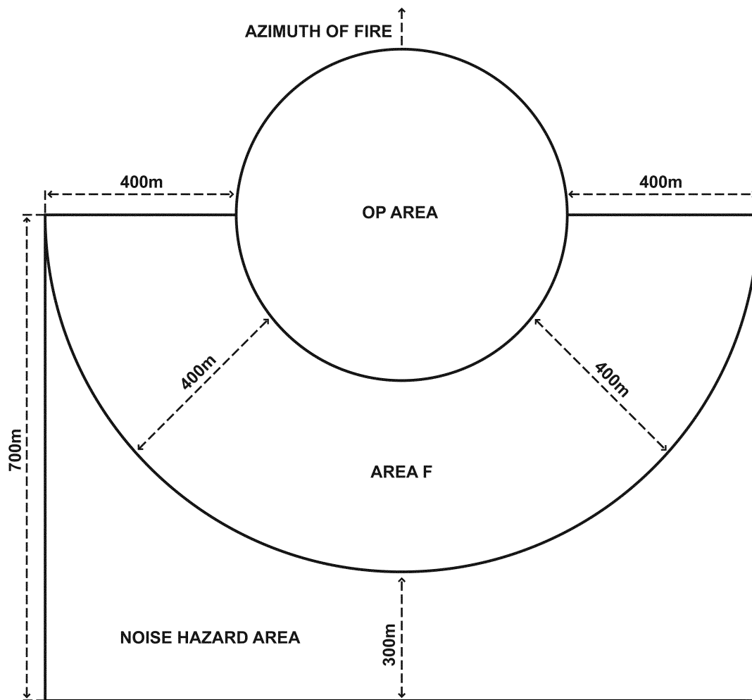
Figure 10-14. Area F for reduced range practice rocket operational area
