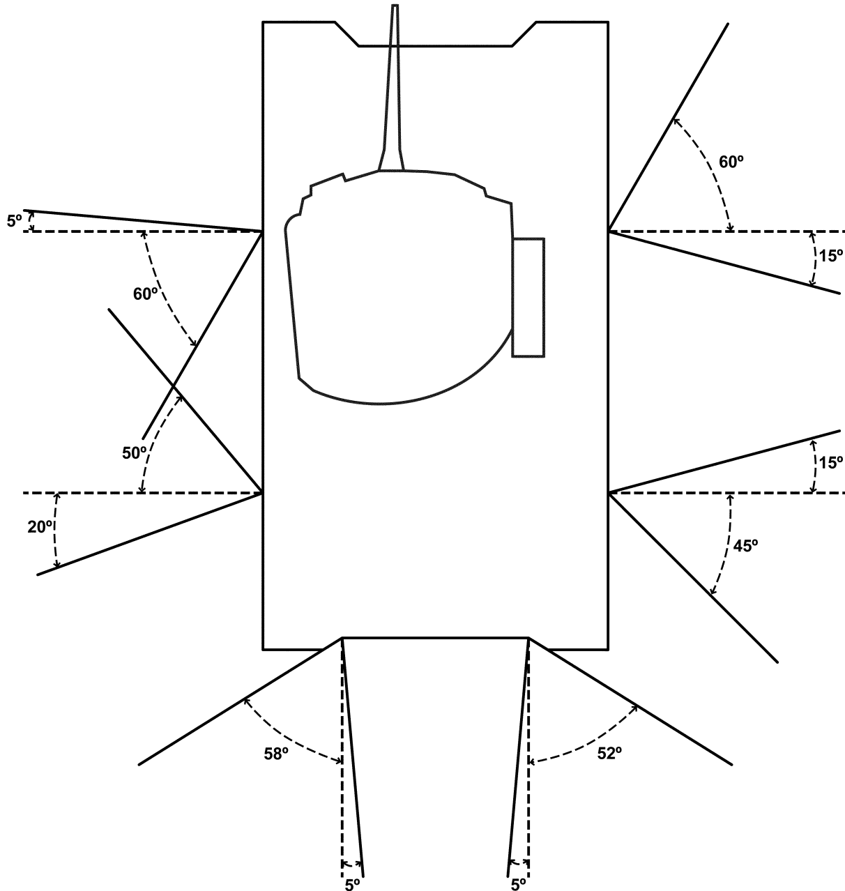
Figure 8-6. Surface danger zone for fighting vehicle firing port weapon systems
