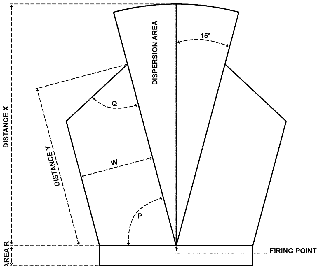
Figure 14-3. Surface danger zone for the 40mm grenade foam rubber baton (BA07), rubber ball grenade (BA08), and M1029 (BA13)
