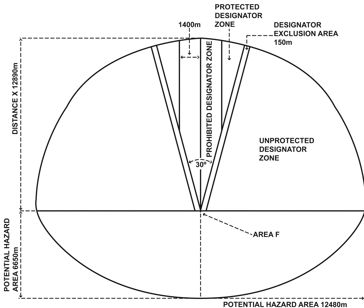
Figure 11-7. Expanded indirect weapons danger zone/surface danger zone for firing AGM-114 A/F HELLFIRE laser-guided missile with associated tip-off error in the indirect launch mode (Lock-On-After-Launch with remote designation) at fixed target or firing the AGM 114-K/N missile with associated tip-off error in either the direct or indirect launch mode
