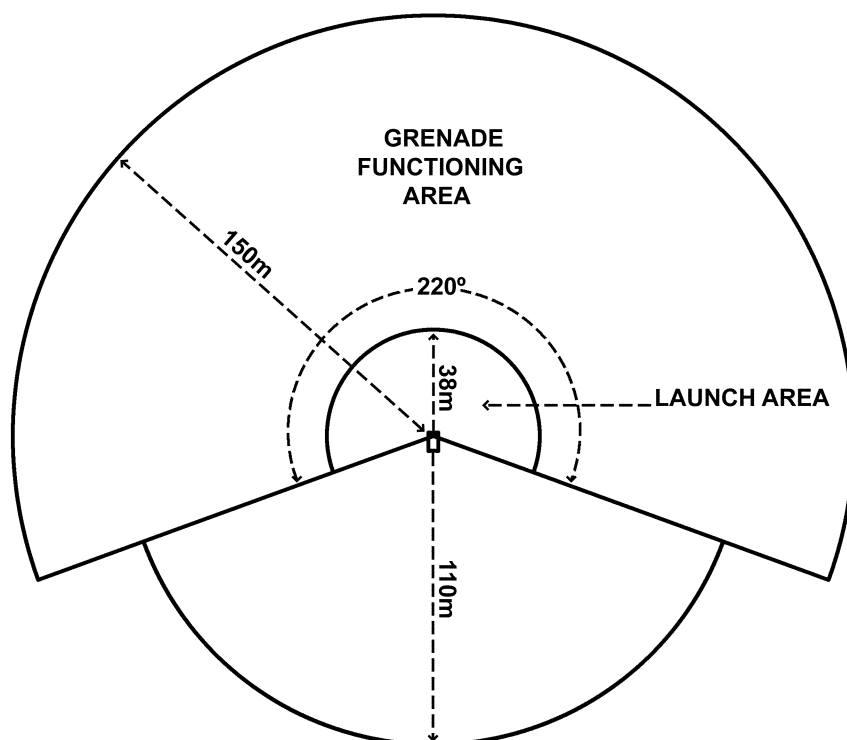
Figure 8–13. Surface danger zones for firing M82 grenades using standard 66mm launchers on armored vehicles
