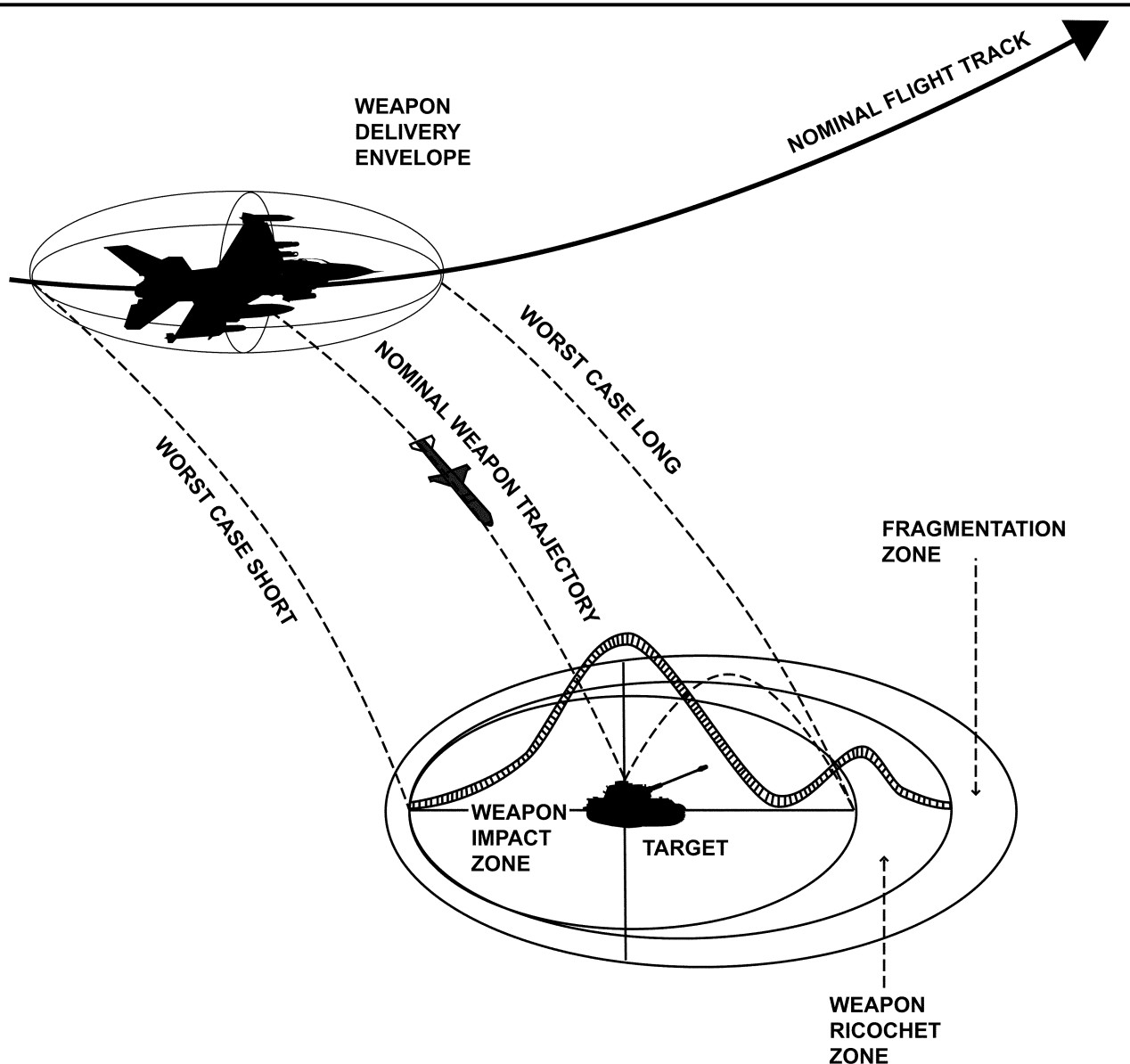
Figure 3-14. Basic weapon danger zone profile
