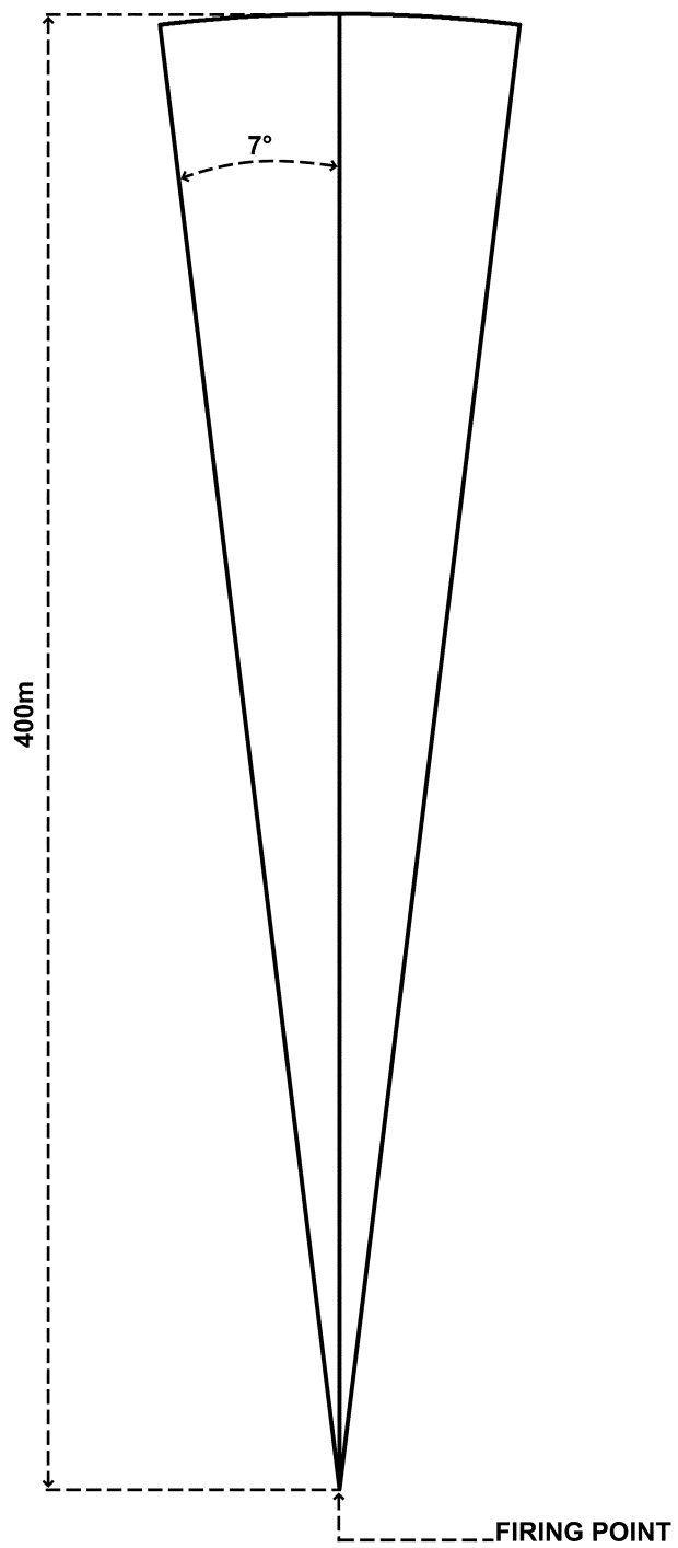
Figure 8-7. 25mm aluminum base Sabot discard hazard area
