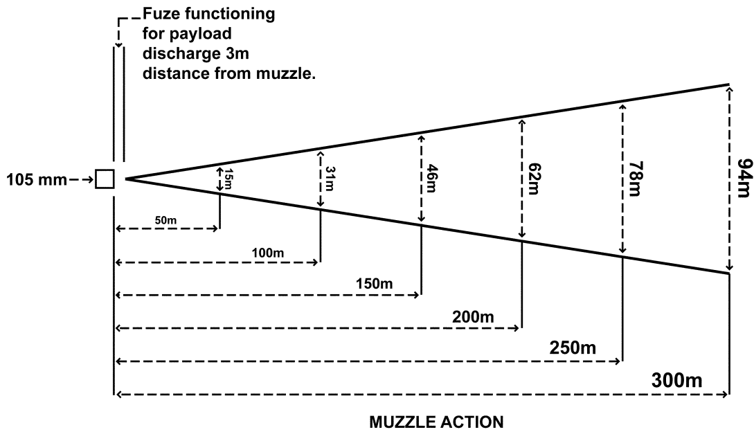
Figure 8-4. Flechette dispersion pattern for for M494 105mm, APERS-T
