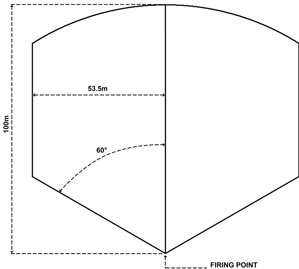
Figure 8-8. 25mm plastic base Sabot discard hazard area
