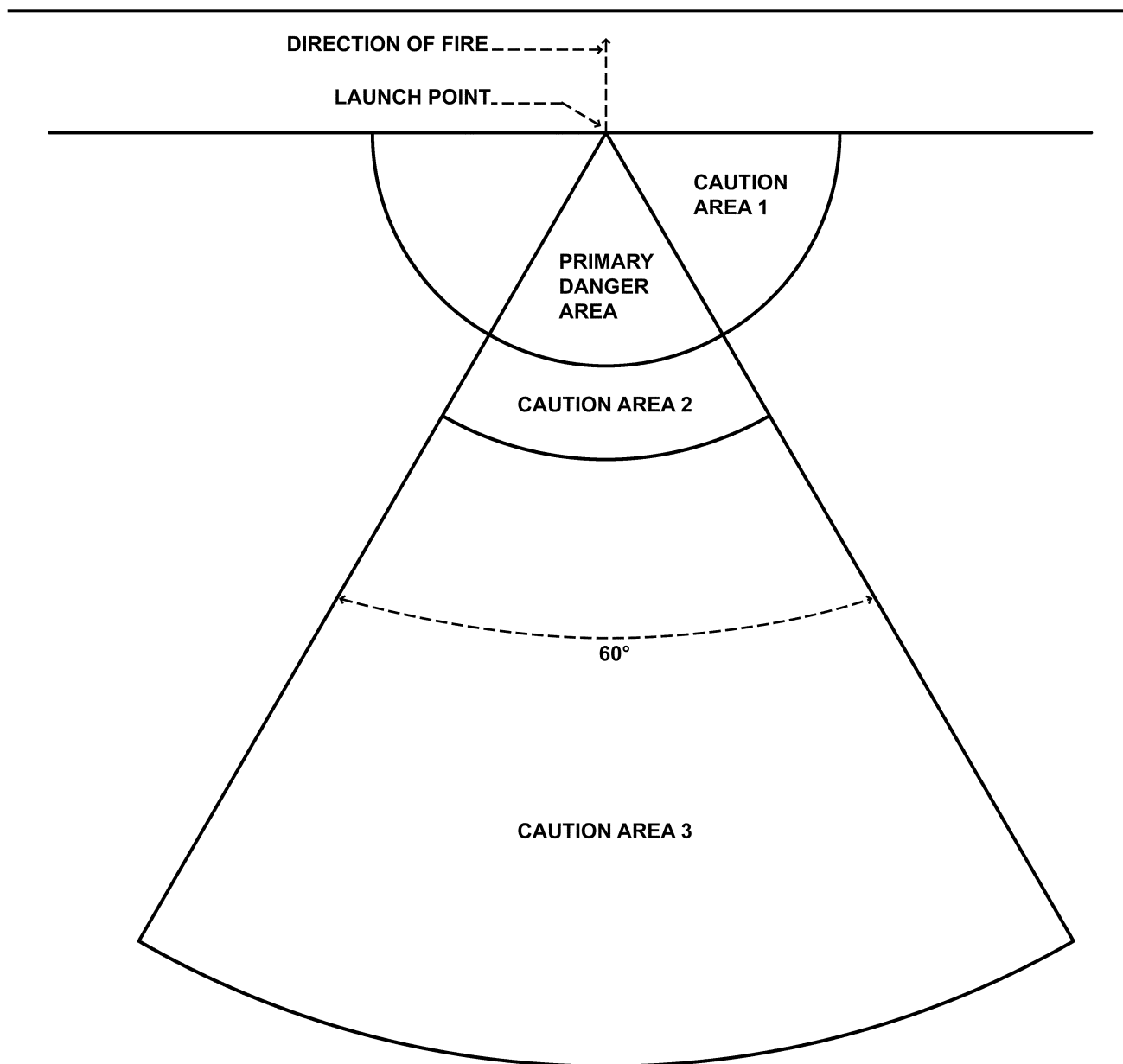
Figure 7-7. Surface danger zone Area F, for Javelin missiles
