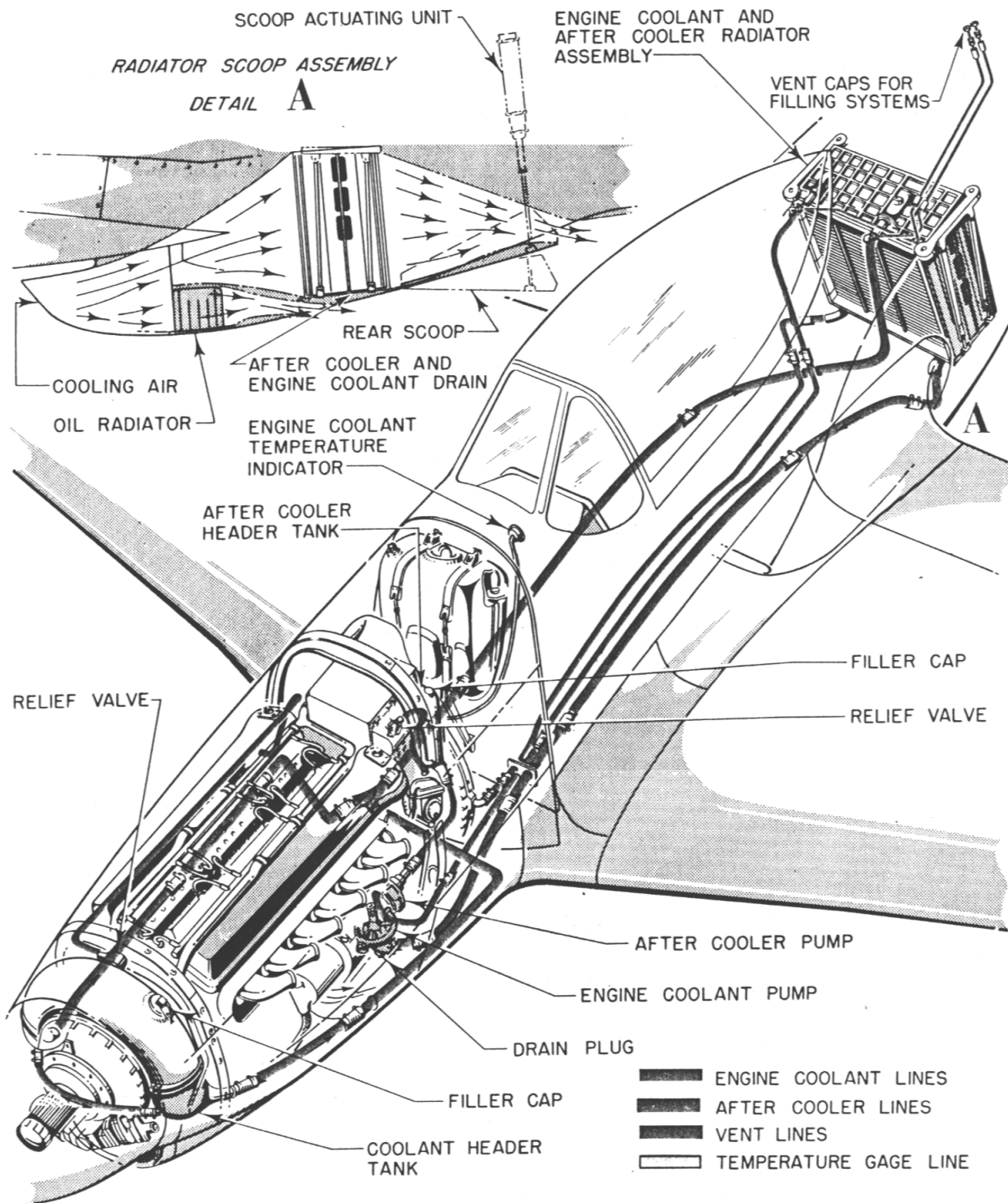
Figure 11—Cooling Systems
