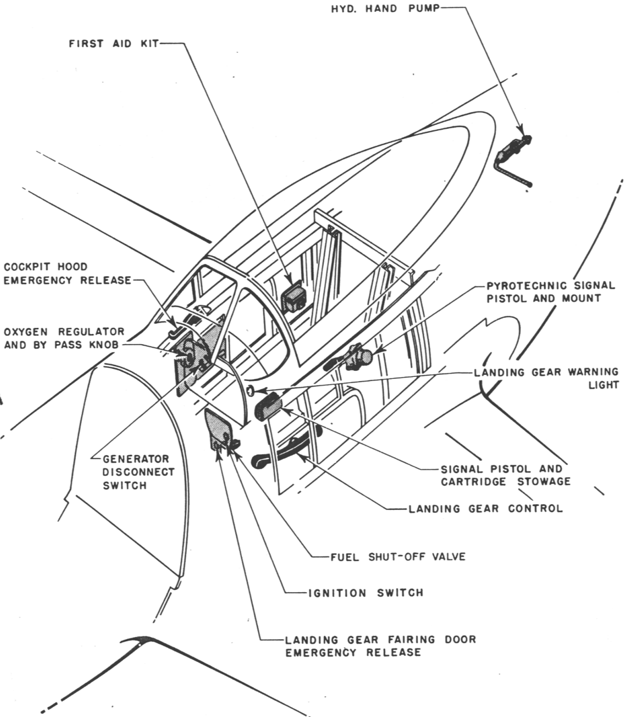
Figure 30—Emergency Equipment
