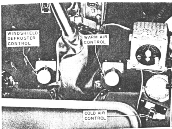
Figure 41—Heating, Ventilating, and Defrosting Controls
