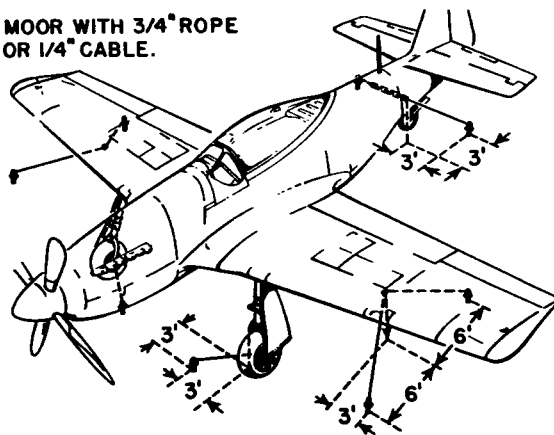
Figure 27—Mooring Airplane
