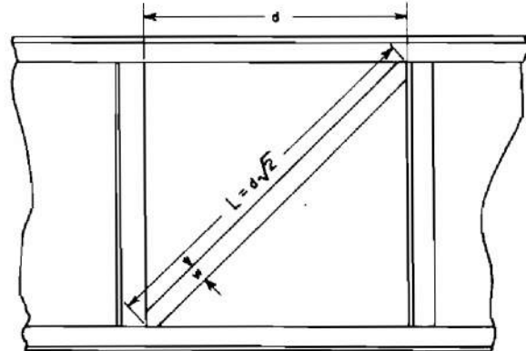
Figure 18. Stiffener Spacing Based on Column Analogy
