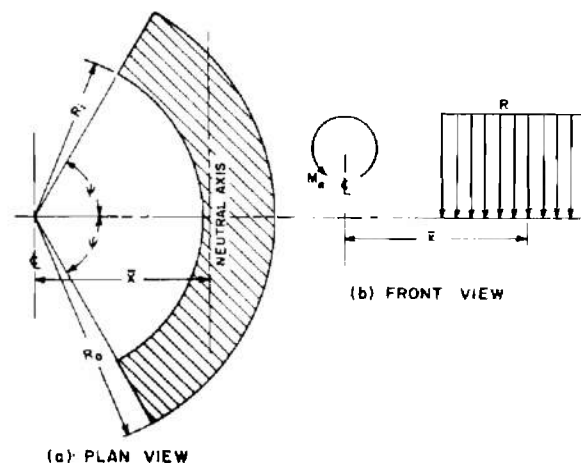
Figure 9. Uniform Load Distribution on Annular Sector
