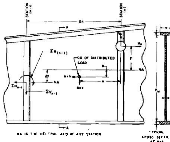
Figure 16. Load Analysis of a Side Frame Panel
