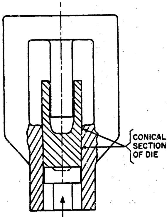
Figure 5-9. French extrusion process
