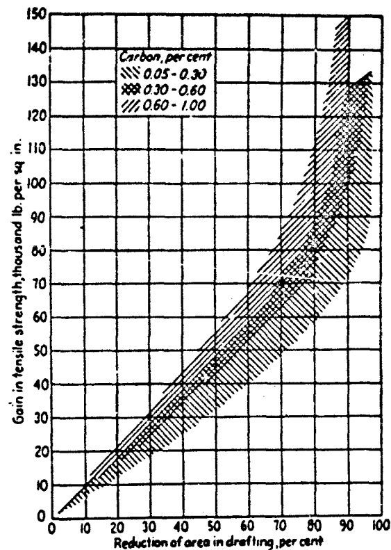
Figure 6-2. Effect of cold working on the tensile strength of carbon steel, gain in tensile strength versus area reduction
