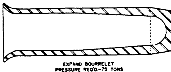
Figure 6-18. Expand bourrelet
