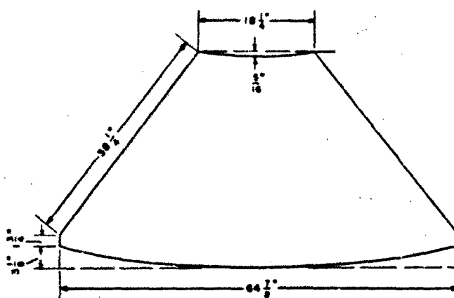
Figure 6-32. Body layout
