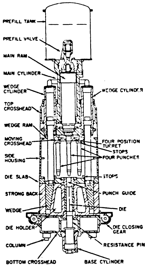
Figure 6-5. One-shot press
