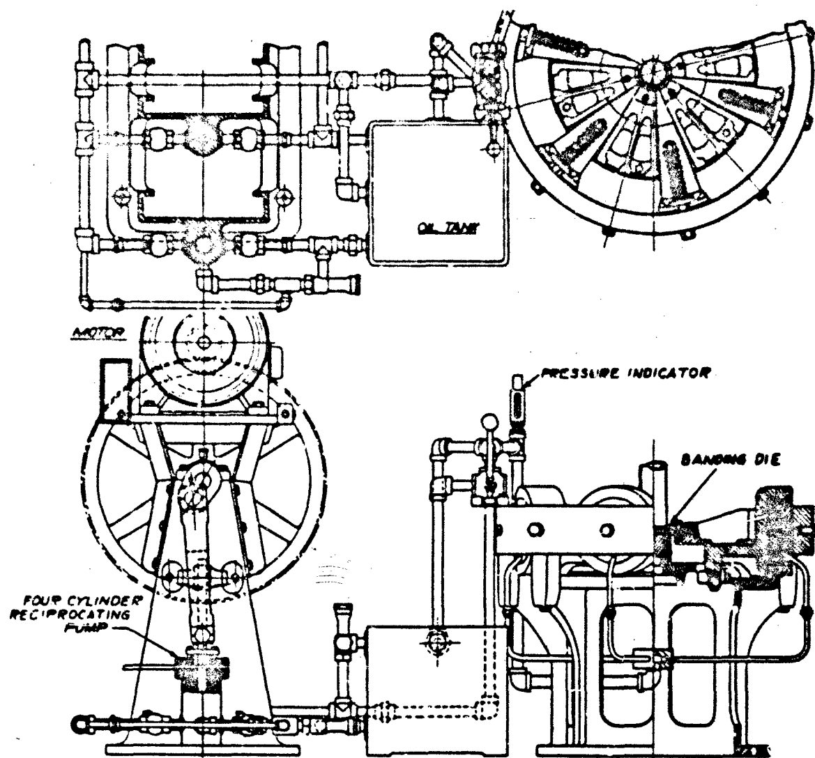
Figure 6-13. Hydraulic banding press and pump
