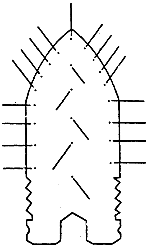
Figure 6-25. AP shot profile
