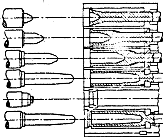
Figure 6-10. Upsetter forging
