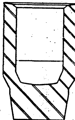
2ND HIT-1ST EXTRUDE PRESSURE REQ'D.-800 TONS D
