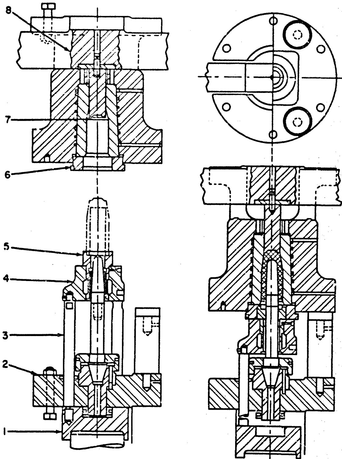
Figure 6-6. Hydraulic press tools
