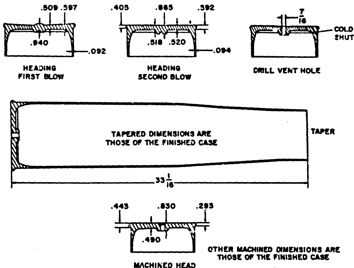
Figure 6-30. Cartridge case process drawing
