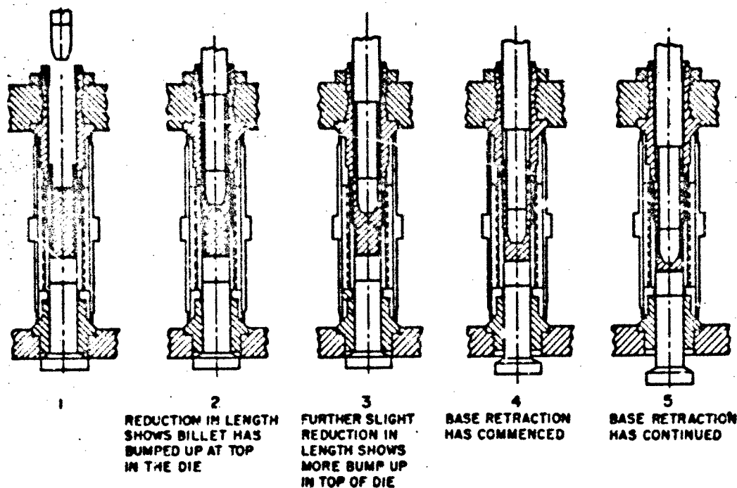
Figure 6-4. Progressive stages of one-shot piercing method
