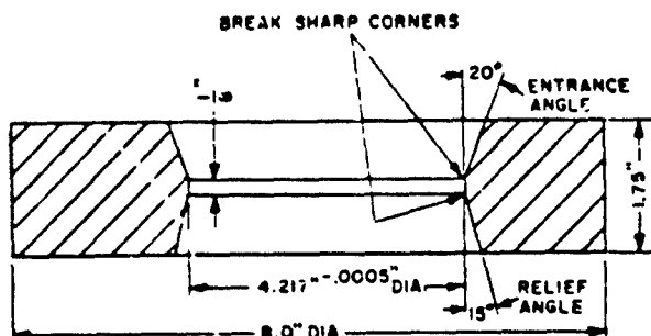
Figure 6-15. Banding die
