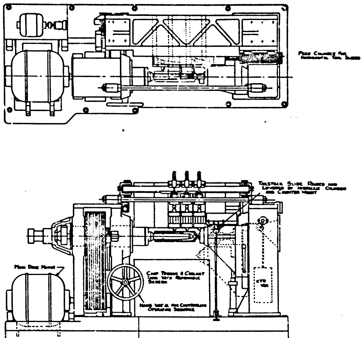
Figure 6-11. Lathes for rough turning
