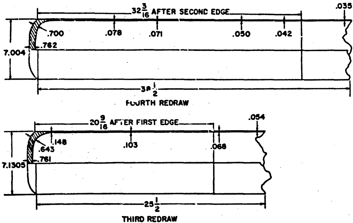
Figure 6-29. Cartridge case process drawing
