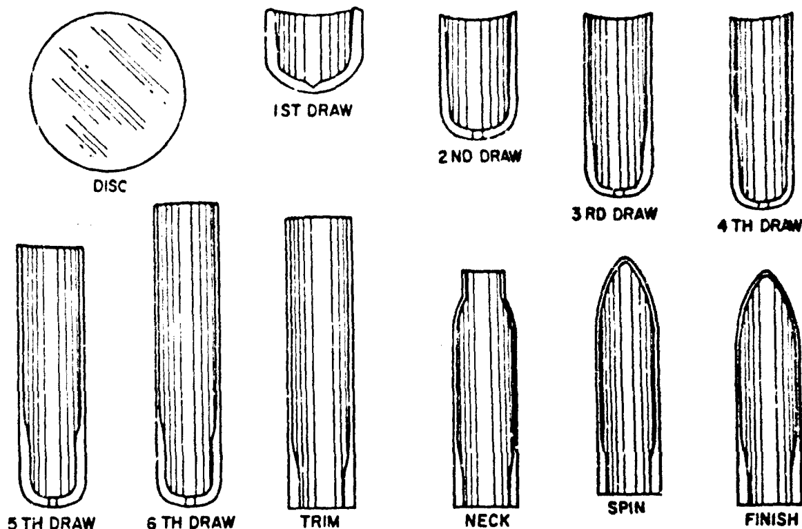
Figure 6-21. HEP fabrication
