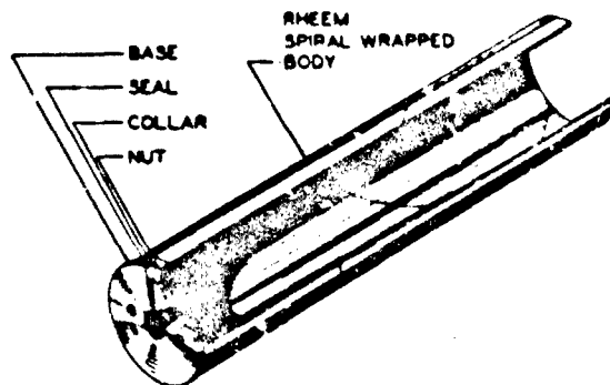
Figure 6-33. 120-mm case assembly
