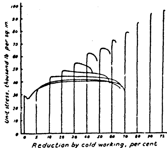
Figure 6-1. Stress-strain curves of cold-worked, low-carbon steel
