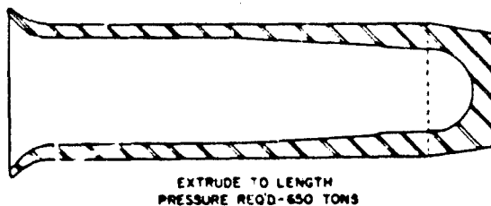
Figure 6-17. Slug, extrude to length
