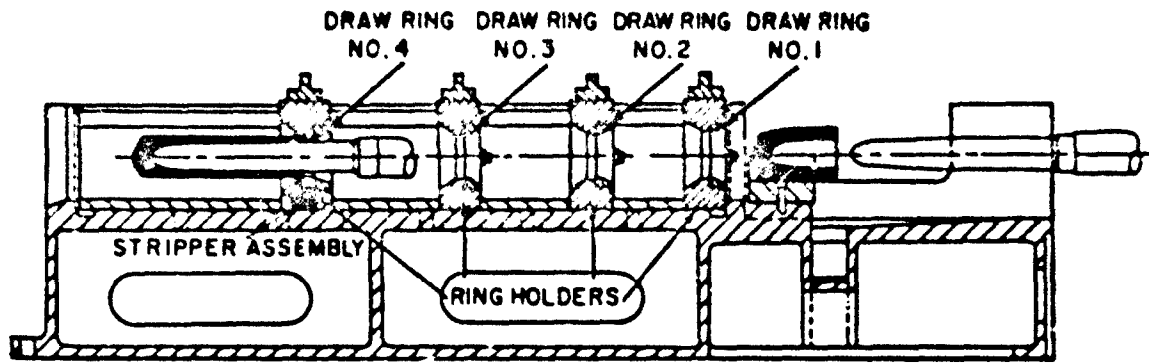
Figure 6-7. Draw bench
