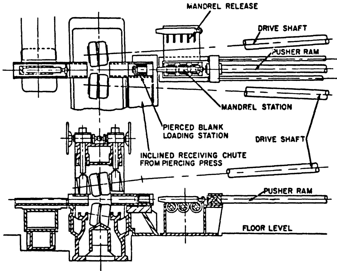
Figure 6-8. Cross rolling mill
