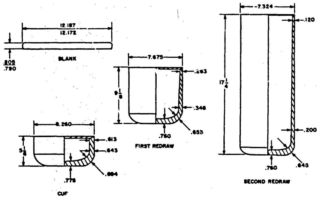
Figure 6-28. Cartridge case process drawing
