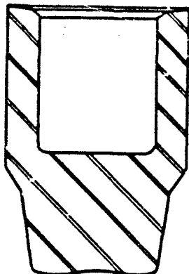
1ST HIT-1ST EXTRUDE PRESSURE REQ'D.-1100 TONS C
