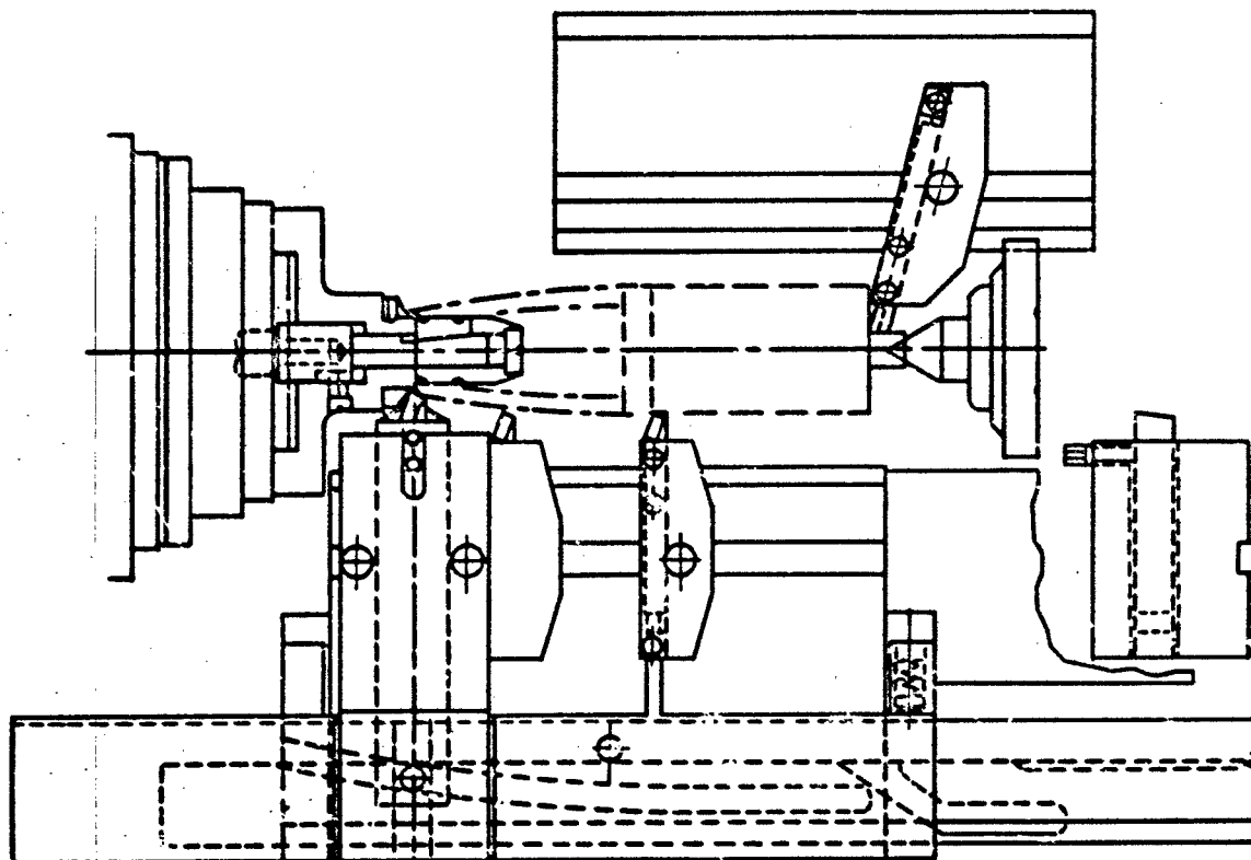
Figure 6-12. Tooling setup for turning
