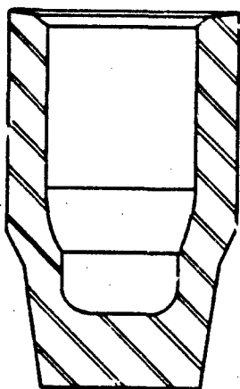
2ND EXTRUDE PRESSURE REQ'D.-650 TONS E
