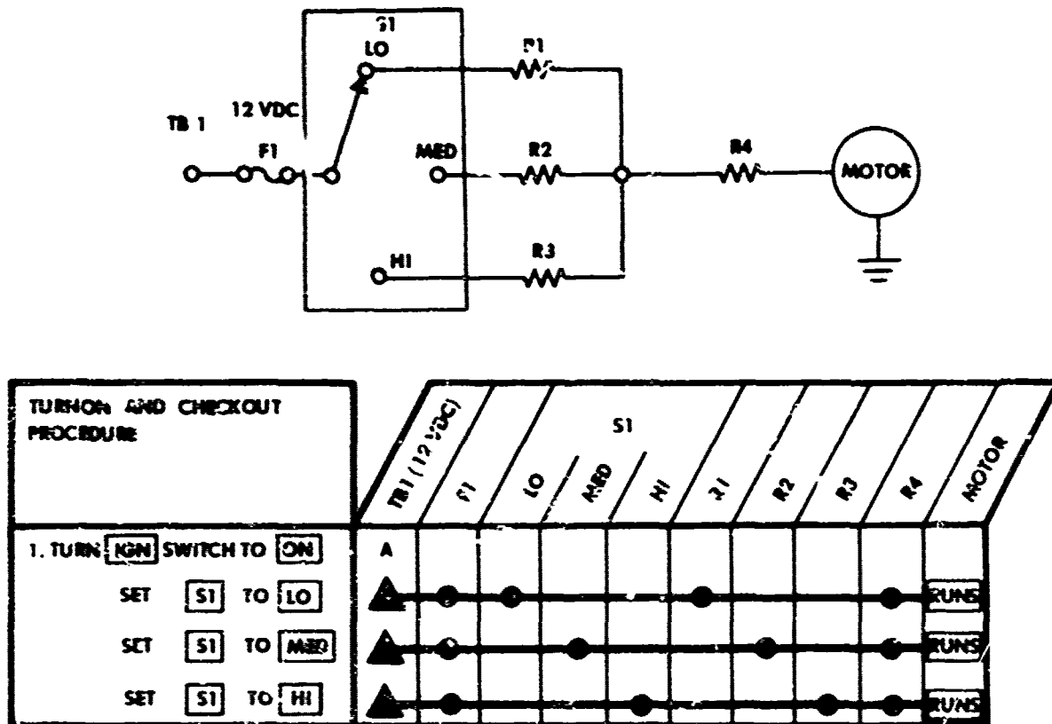
Figure 9-7. Simplified Maintenance Dependency Chart (Ref. 17)
