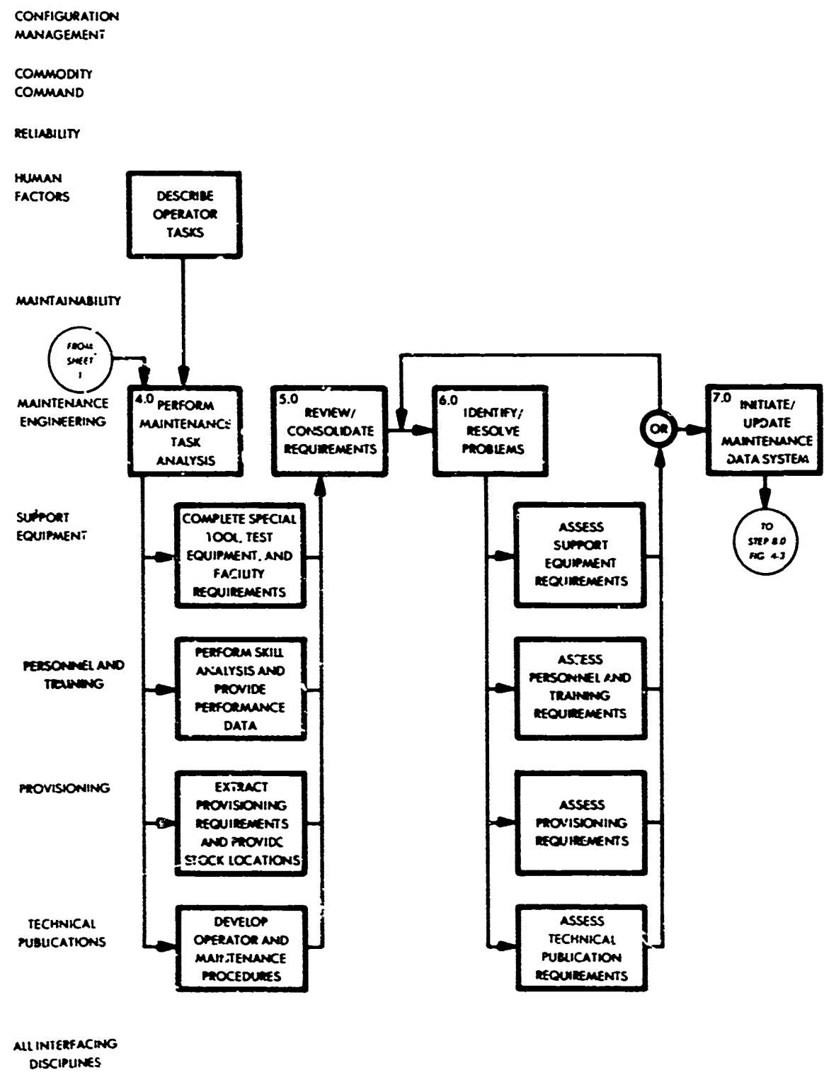
Figure 4-4. Maintenance Procedural Model - Second level (sheet 2 of 2)
