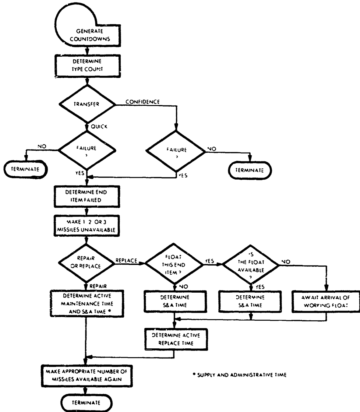
Figure 8-2. Simulation Model Basic Flow
