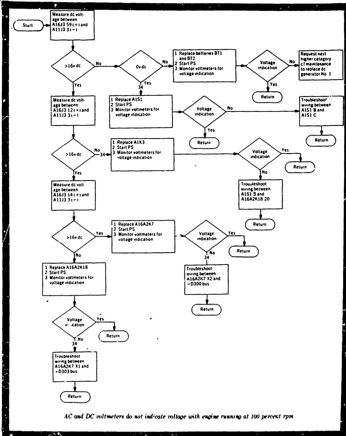
Figure 4-5. Sample Flow Diagram
