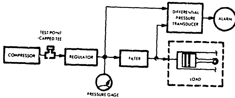
(A) HYDRAULIC/PNEUMATIC SYSTEM
