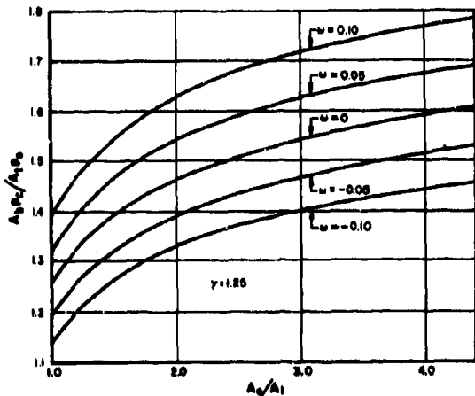
FIGURE 23. Lines of Constant Dimensionless Recoil.
