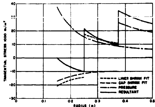
FIGURE 64. Tangential Stress of Shrink Fitted Tube.
