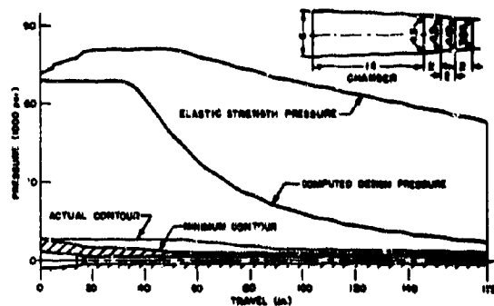
FIGURE 61. Design Data, Monobloc Artillery Tube.
