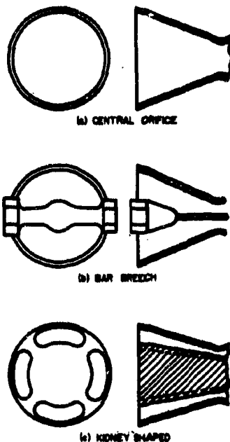
FIGURE 24. Nozzle Shapes-Schematic.
