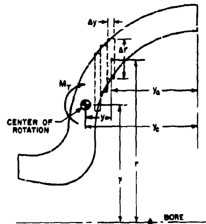
FIGURE 46. Toroidal Internal Moment Center.
