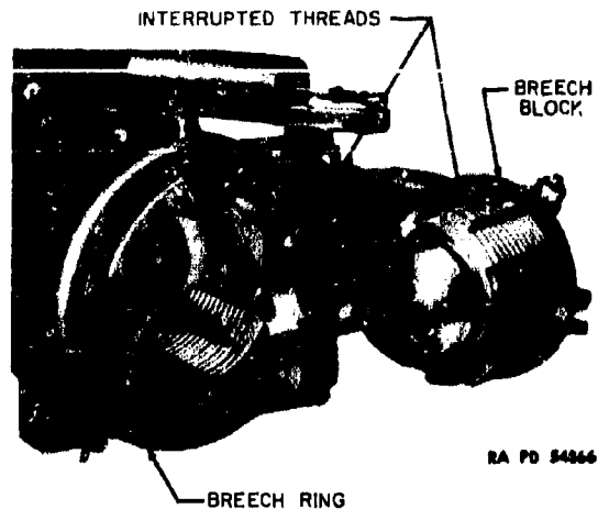
FIGURE 51. Interrupted Threads.
