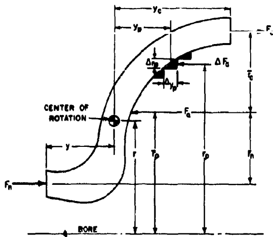
FIGURE 47. Toroidal External Loads.
