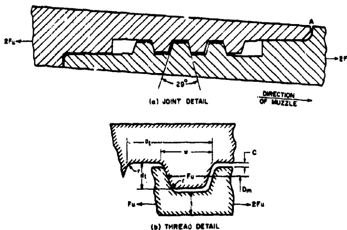
FIGURE 52. Threaded Joint.
