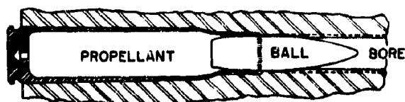
(b) SMALL ARMS CHAMBER CONTAINING FIXED ROUND
