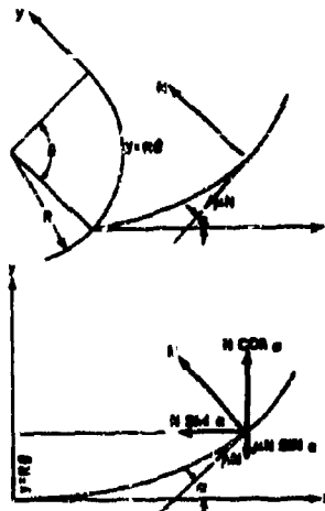
FIGURE 23. Rifling Force Diagram.
