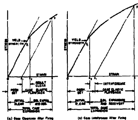
FIGURE 17. Case-Chamber Stress-Strain Curves.
