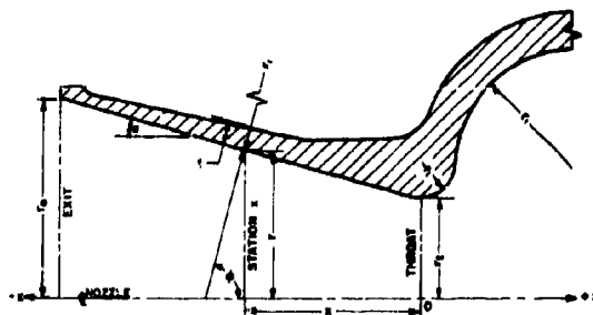
FIGURE 48. Nozzle With General Dimensions.
