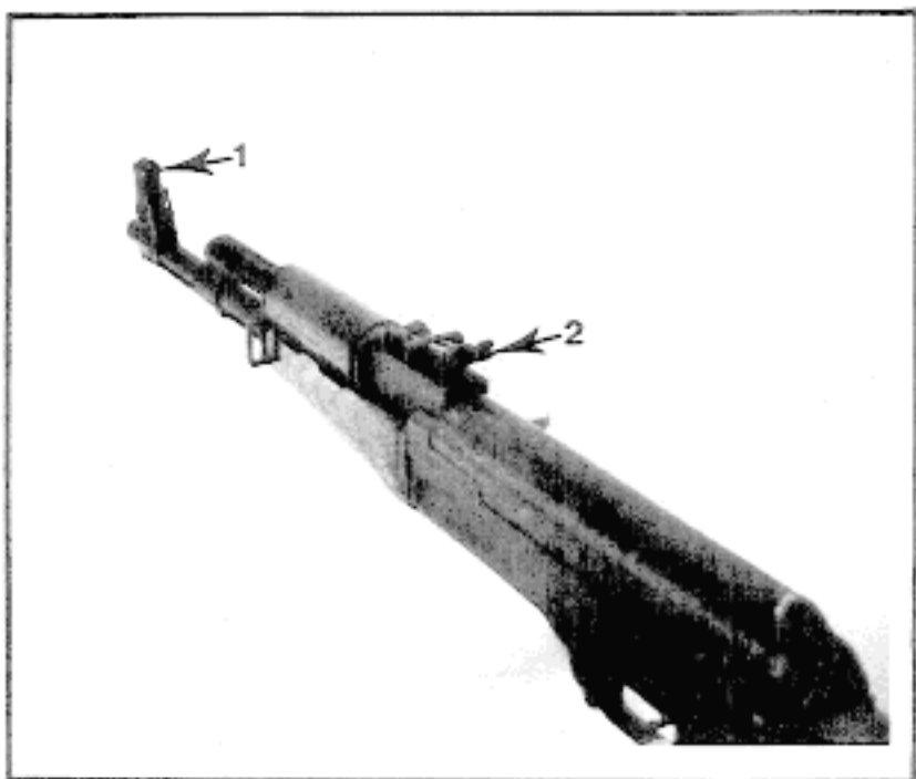
FIGURE 50. LUMINOUS DOTS
