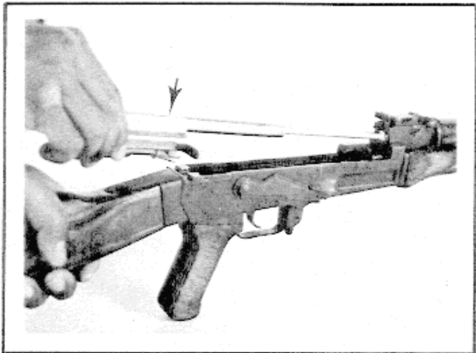
FIGURE 28. REMOVING CARRIER
