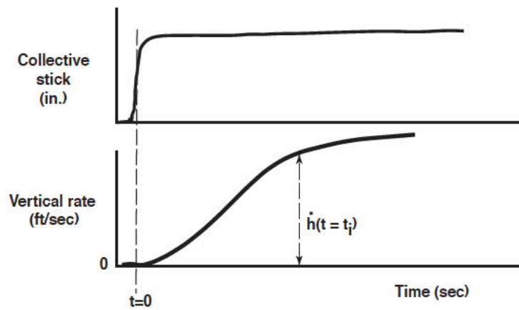
Figure 13. Procedure for obtaining equivalent time domain parameters for the height response to collective controller
