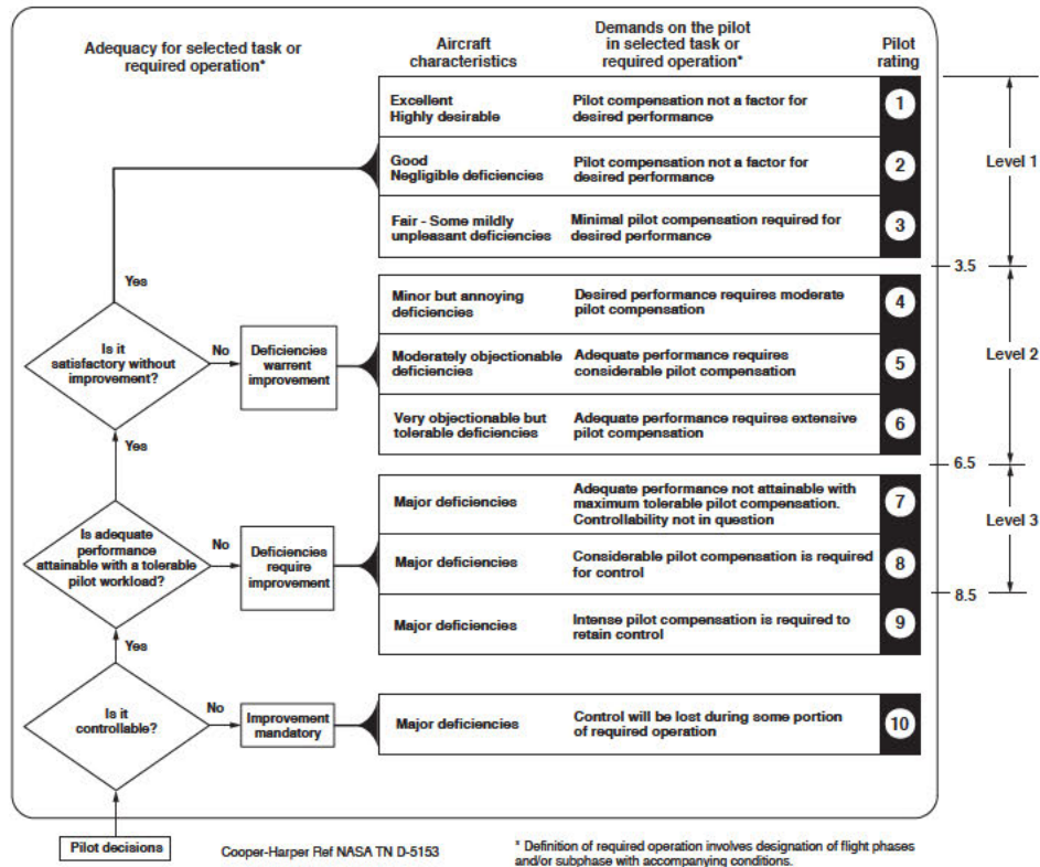
Figure 1. Definition of handling qualities Levels
