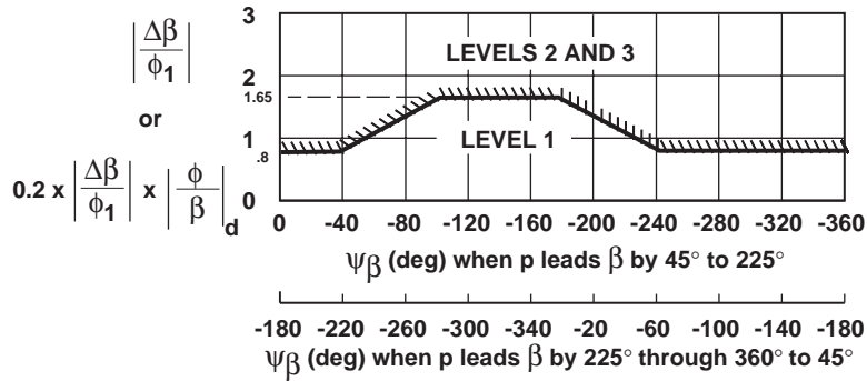
Figure 21. Sideslip excursion limitations
