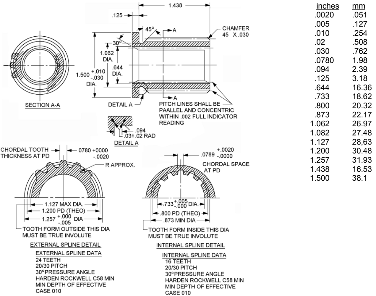
FIGURE 1. Coupling, Shaft, rigid.
