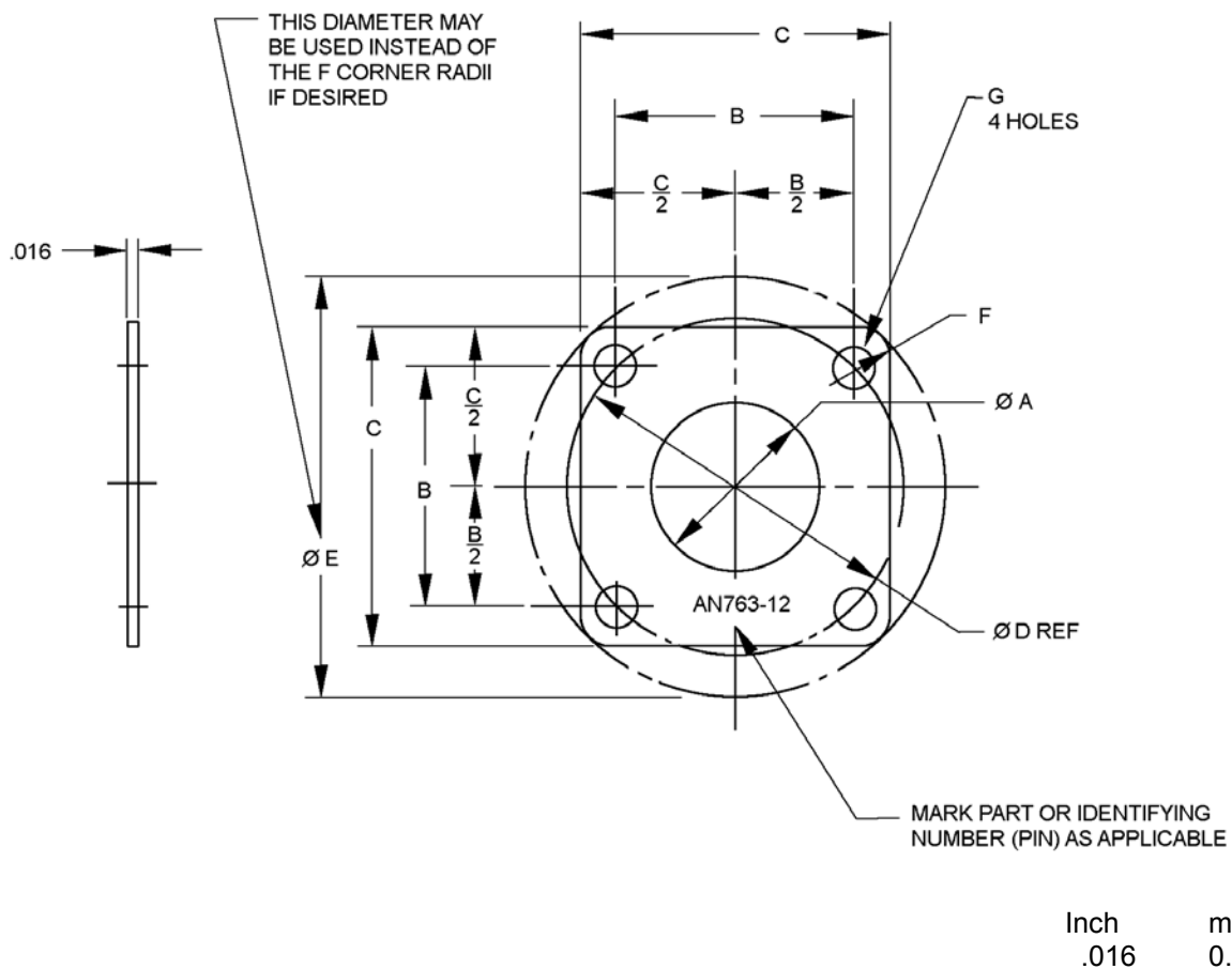
FIGURE 1. Gasket sizes -12 through -32.
