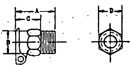
HINGED LID OIL CUP MATERIAL - BRASS & STEEL
