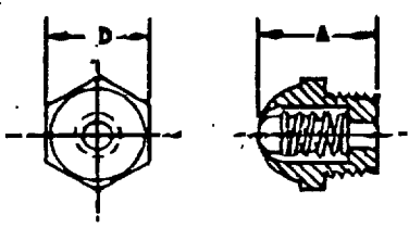
SELF CLOSING OIL CUP MATERIAL - BRASS
